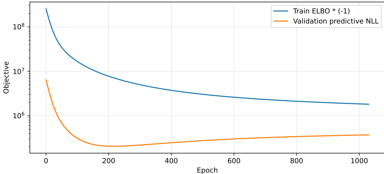
ELBO and validation predictive log-likelihood over epochs
