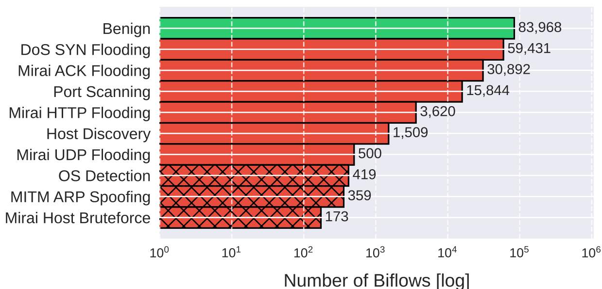
IoT-NID
