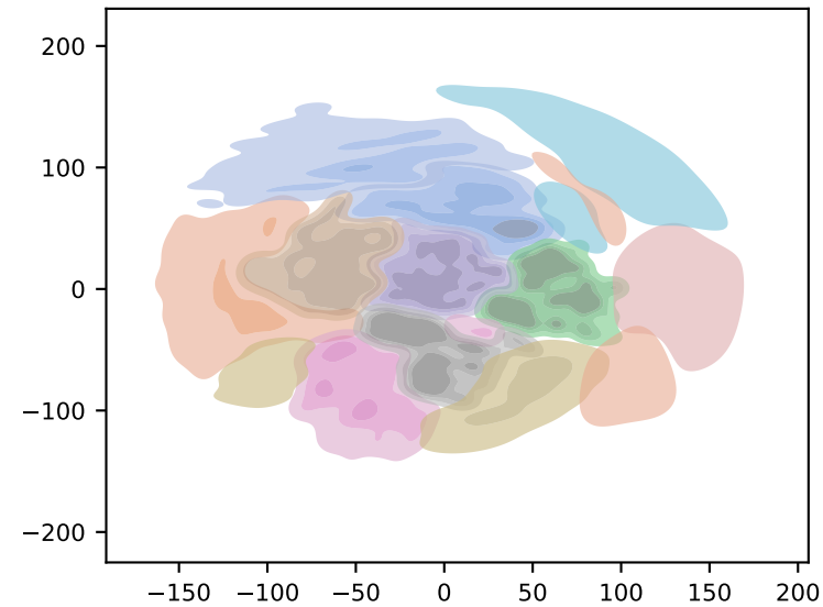
NN-Noise
