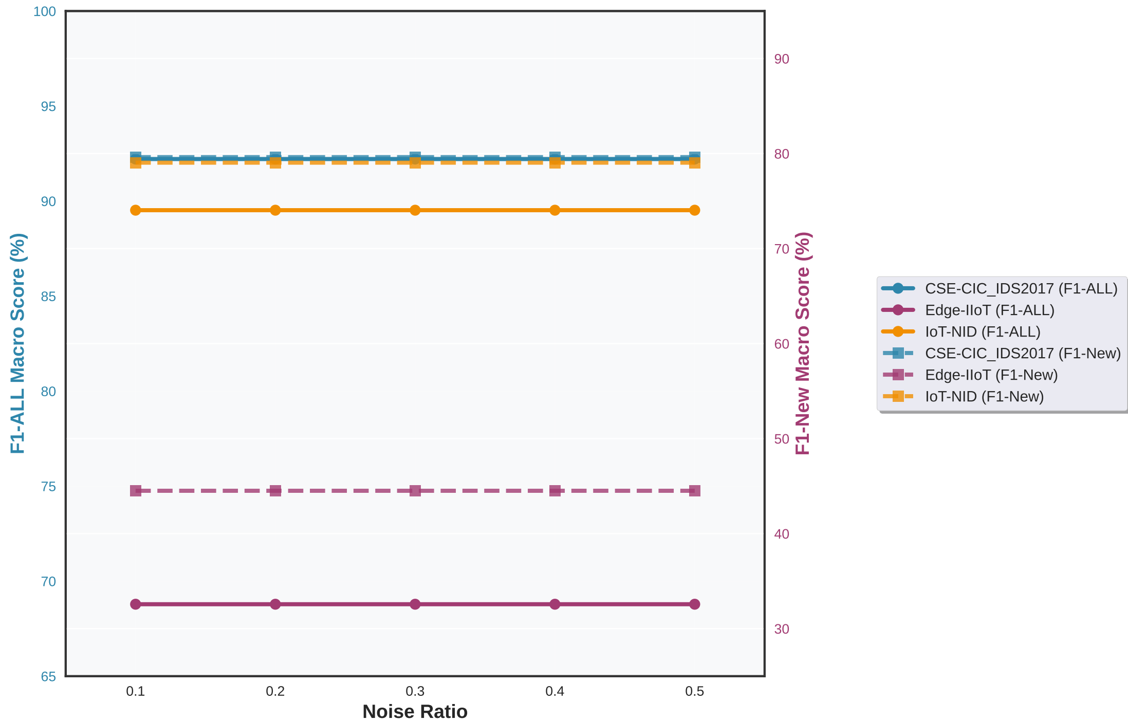
Logistic Regression (LR) Performance vs Noise Ratio
