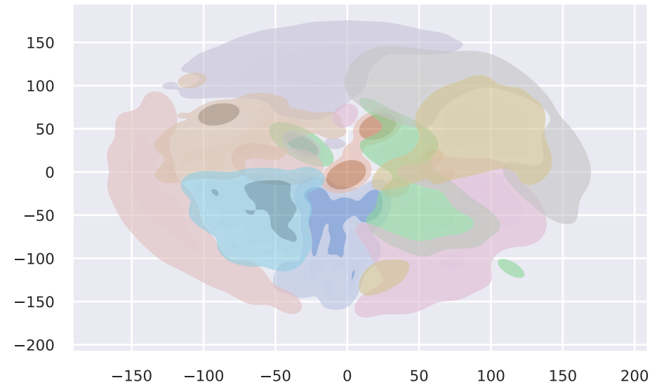
NN-Noise
