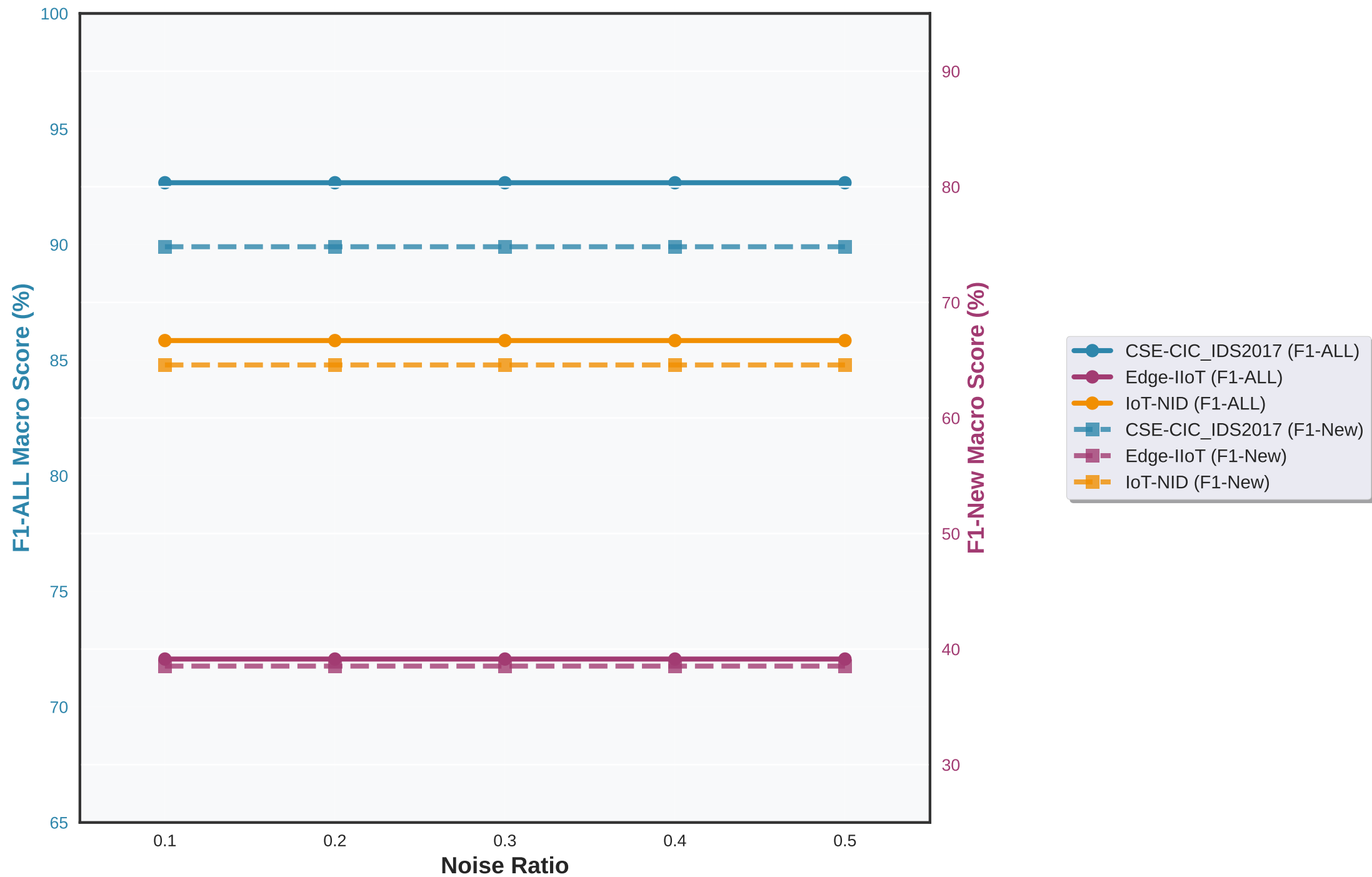
Neural Network (NN) Performance vs Noise Ratio
