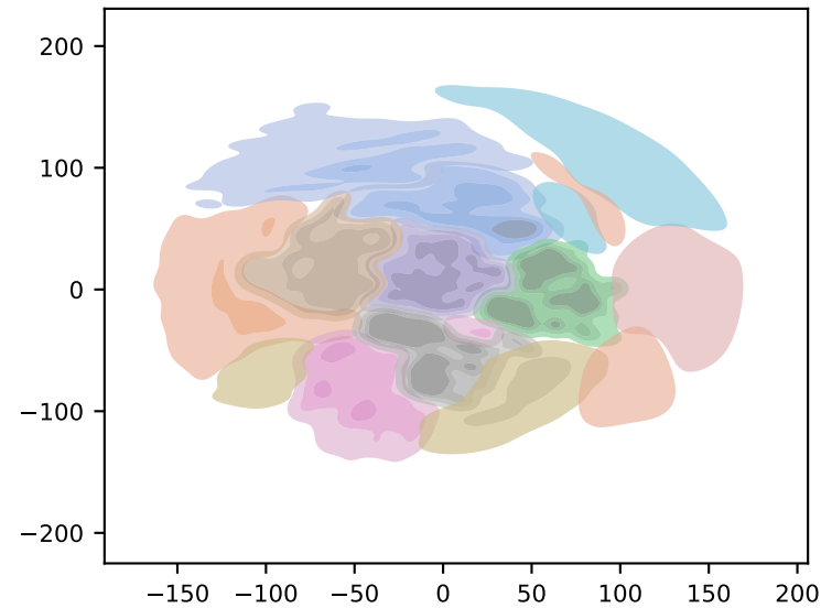
LR-Noise
