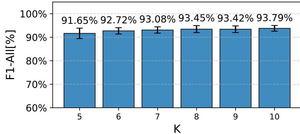
IoT-NID
