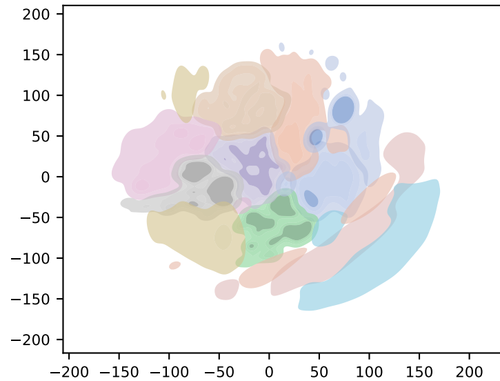
LR-Denoise
