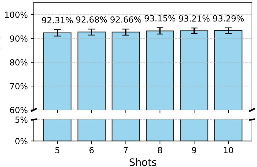
IoT-NID
