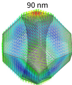
single-vortex/flower
