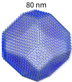
single-domain
