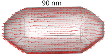
single-domain
