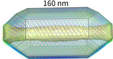
single-vortex
