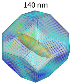
single-vortex
