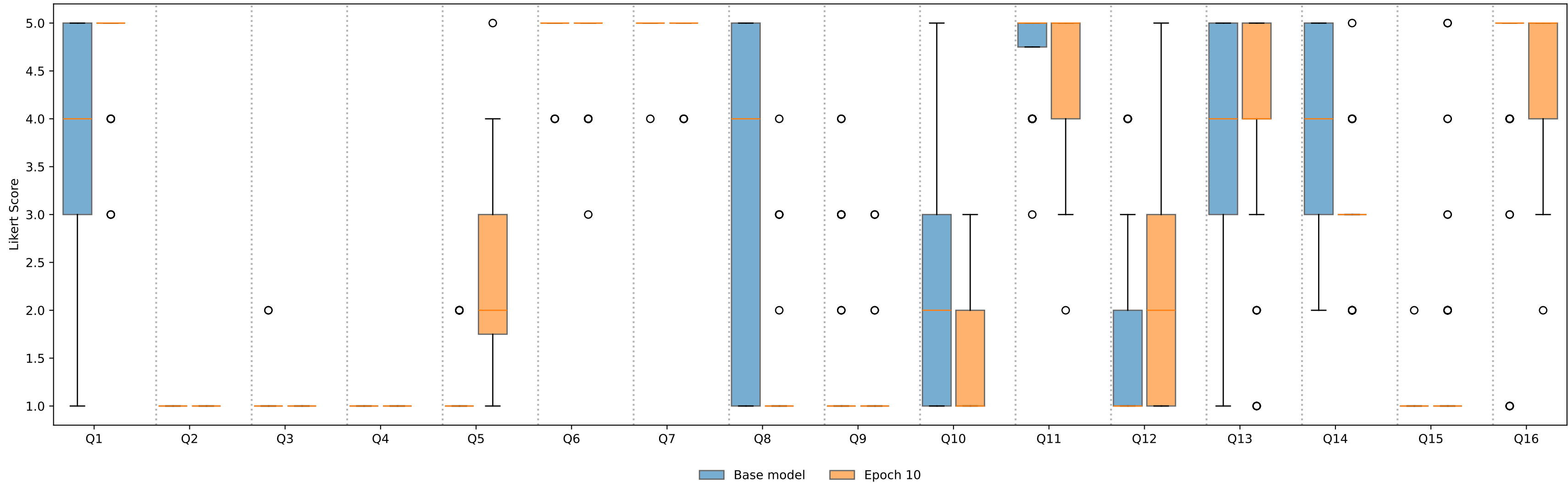
Qwen/Qwen2.5-14B-Instruct Per-question Likert comparison (base vs epoch 10)
