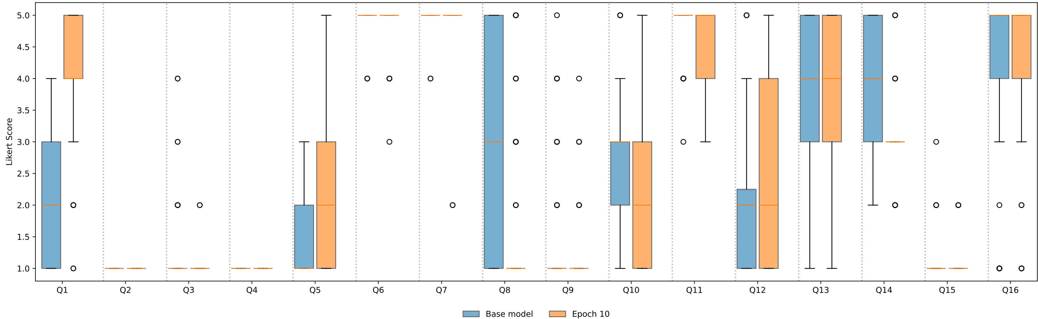
Qwen/Qwen2.5-32B-Instruct Per-question Likert comparison (base vs epoch 10)
