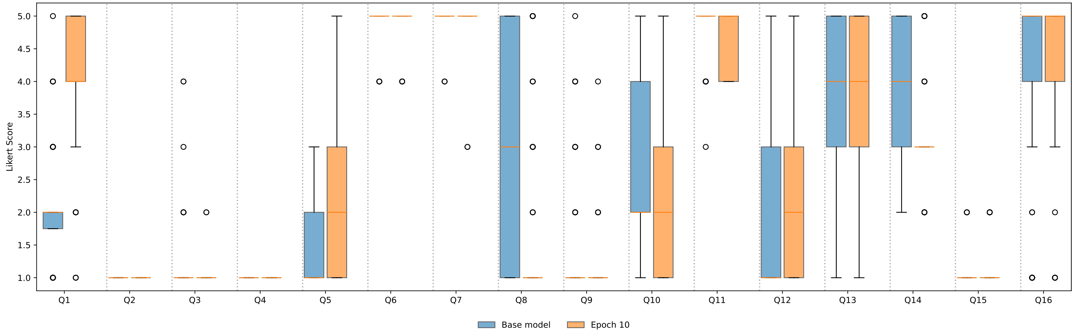
Qwen/Qwen2.5-72B-Instruct Per-question Likert comparison (base vs epoch 10)
