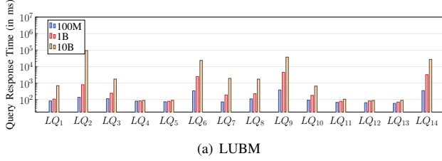
Fig. 9. Scalability Test of Offline Performance
