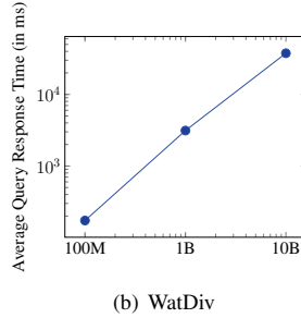
Fig. 10. Scalability Test of Online Performance
