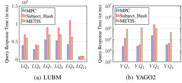
Fig. 11. Online Performance Using gStoreD
