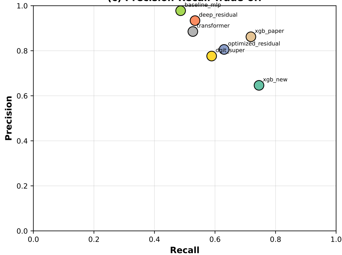
(c) Precision-Recall Trade-off
