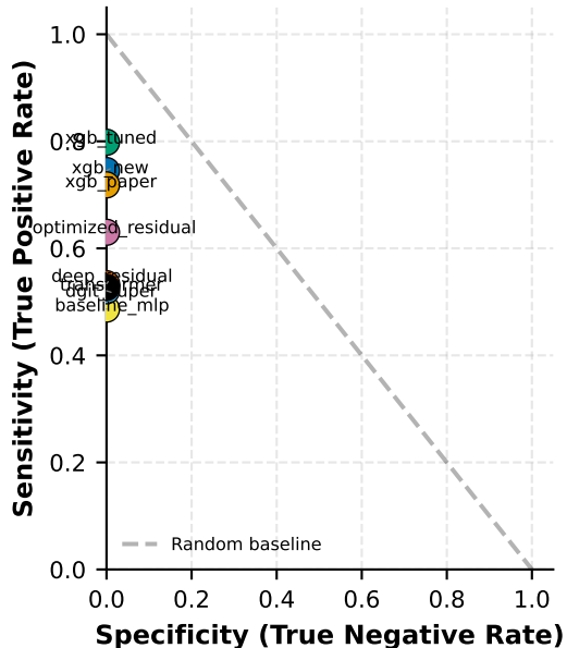
(b) Sensitivity-Specificity Trade-off
