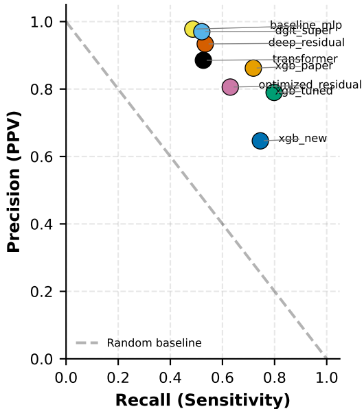
(a) Precision-Recall Trade-off
