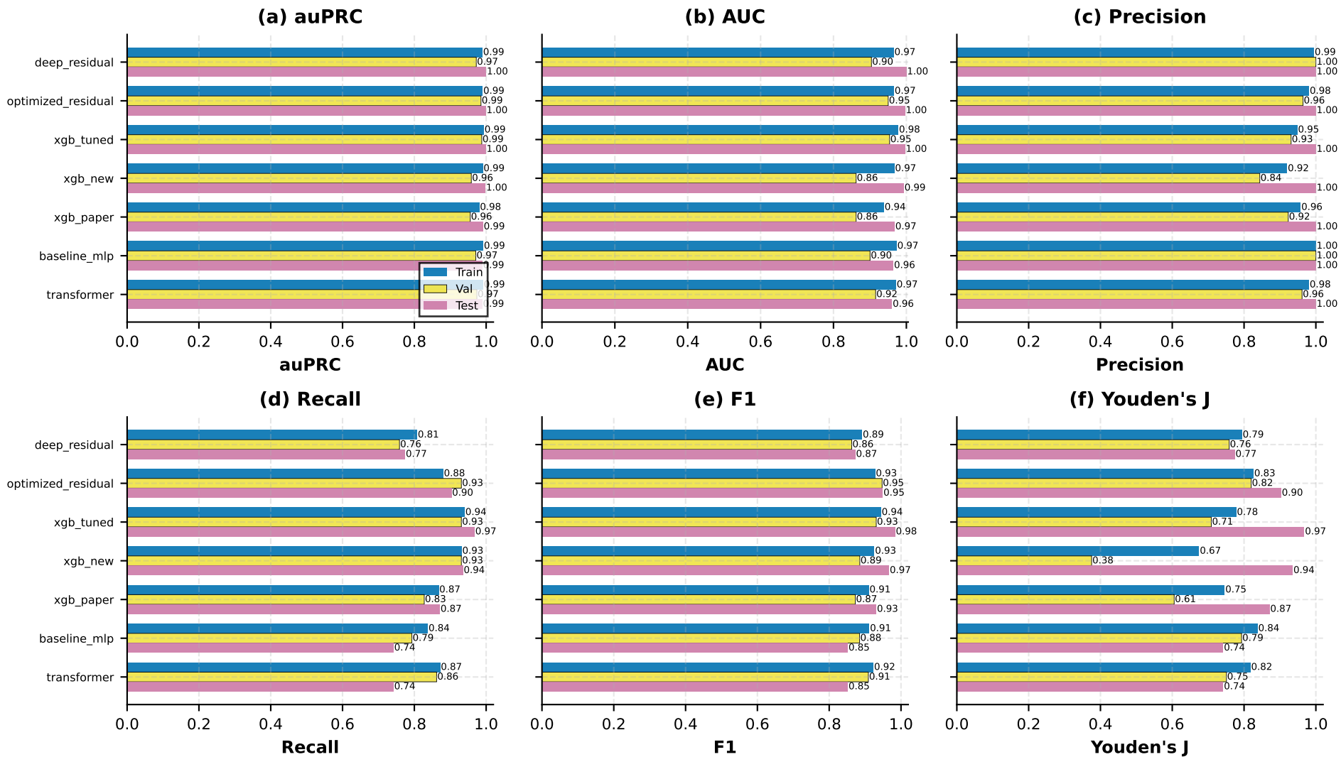
Sample-Level Performance on Test Set
