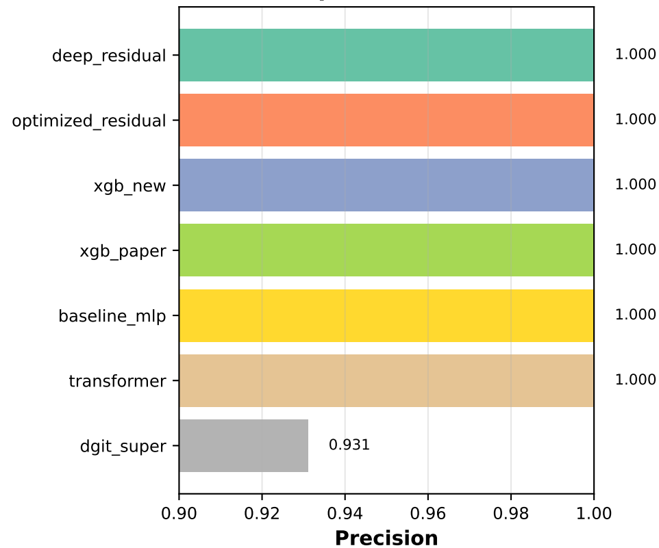
(b) Sample-Level Precision
