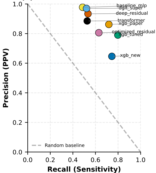
(a) Precision-Recall Trade-off
