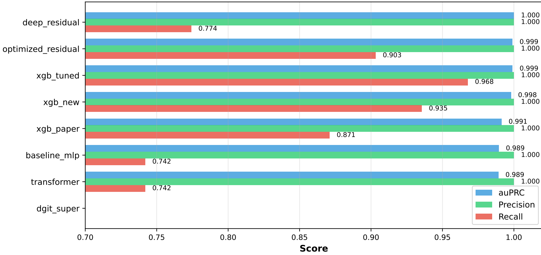
Sample-Level Performance (Circular Detection)
