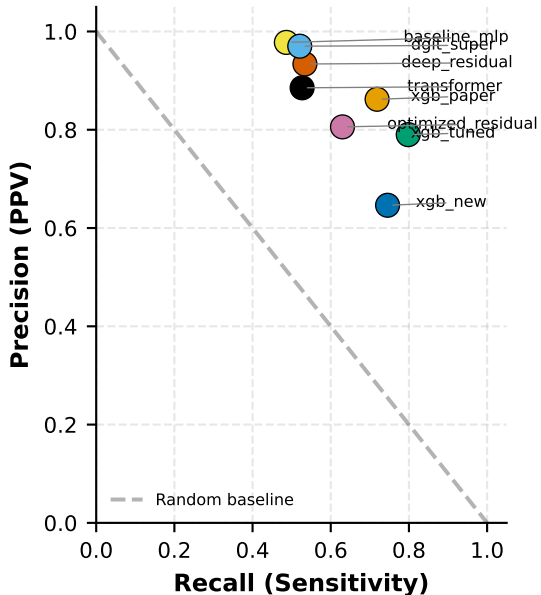
(a) Precision-Recall Trade-off
