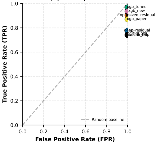
(a) ROC Space
