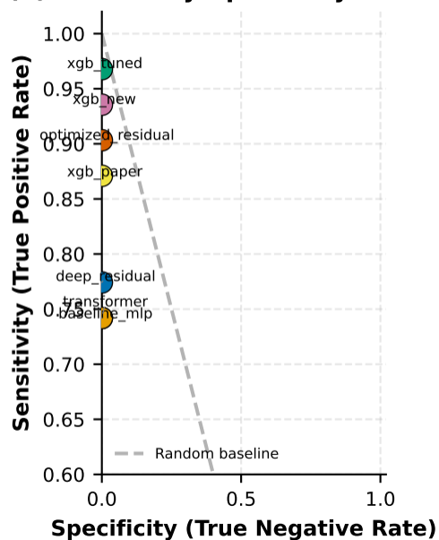
(b) Sensitivity-Specificity Trade-off
