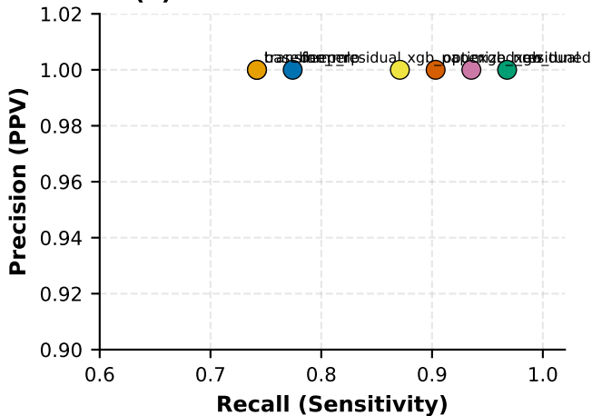
(a) Precision-Recall Trade-off
