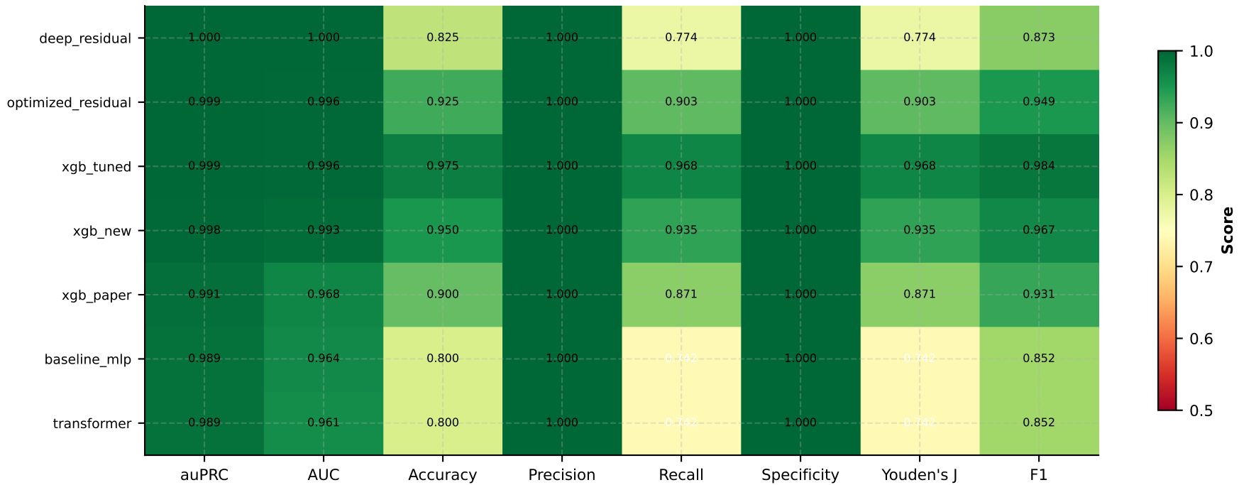
Sample-Level Model Performance Heatmap (Test Set)
