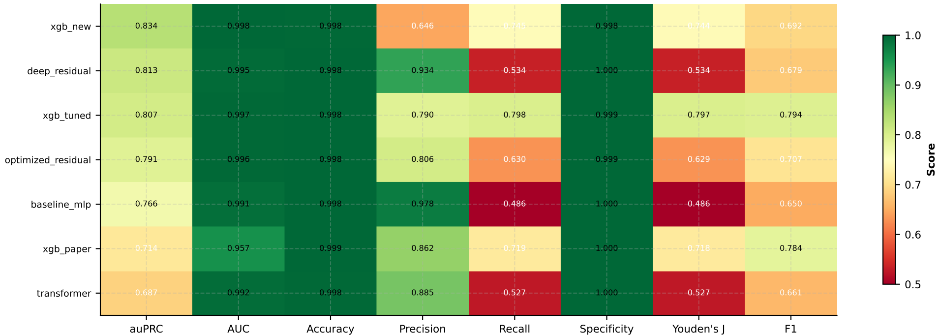
Gene-Level Model Performance Heatmap (Test Set)
