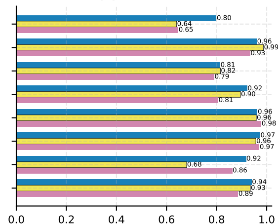
(c) Precision
