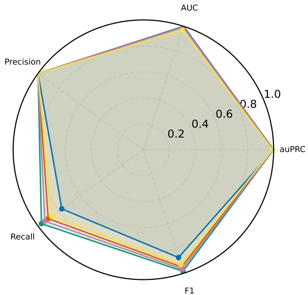
(b) Sample-Level
