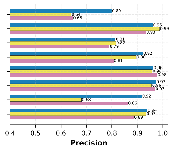
(c) Precision
