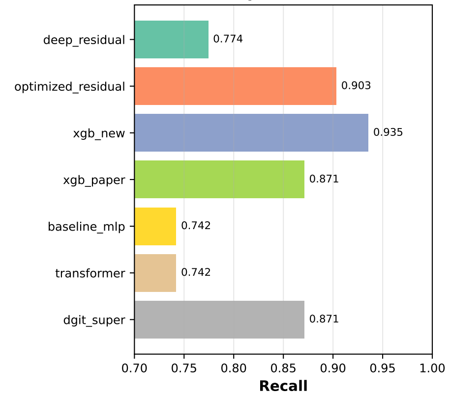
(c) Sample-Level Recall
