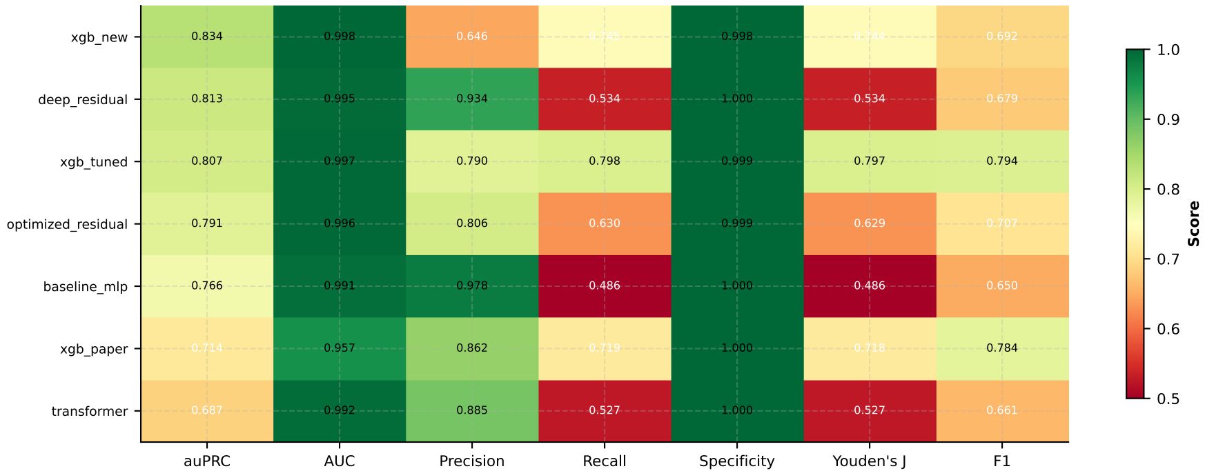
Gene-Level Model Performance Heatmap (Test Set)
