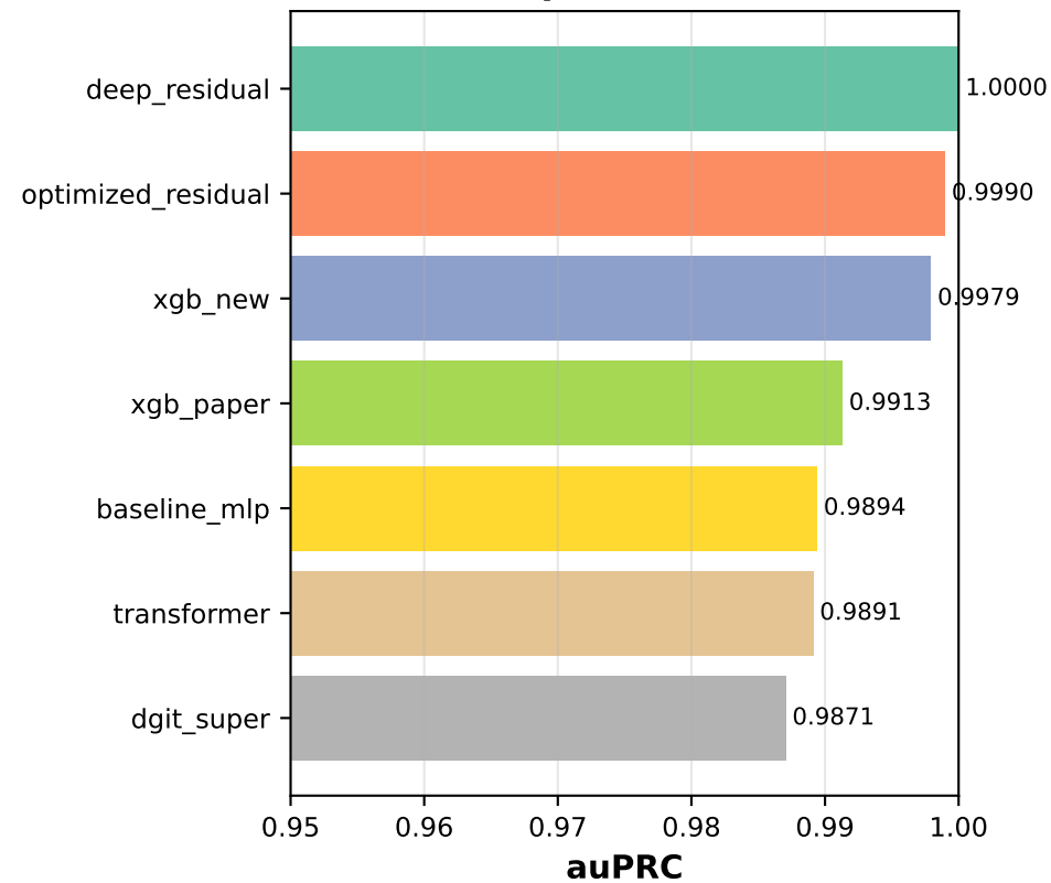
(a) Sample-Level auPRC
