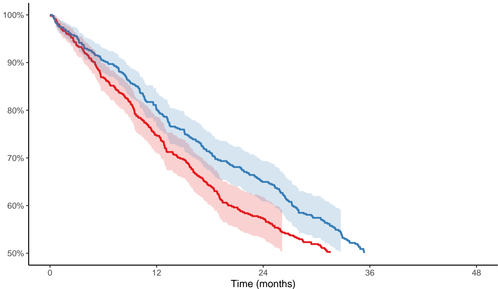
Disease-Free Survival by Treatment Group
