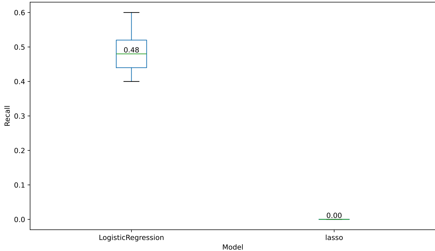
Boxplot for Recall
