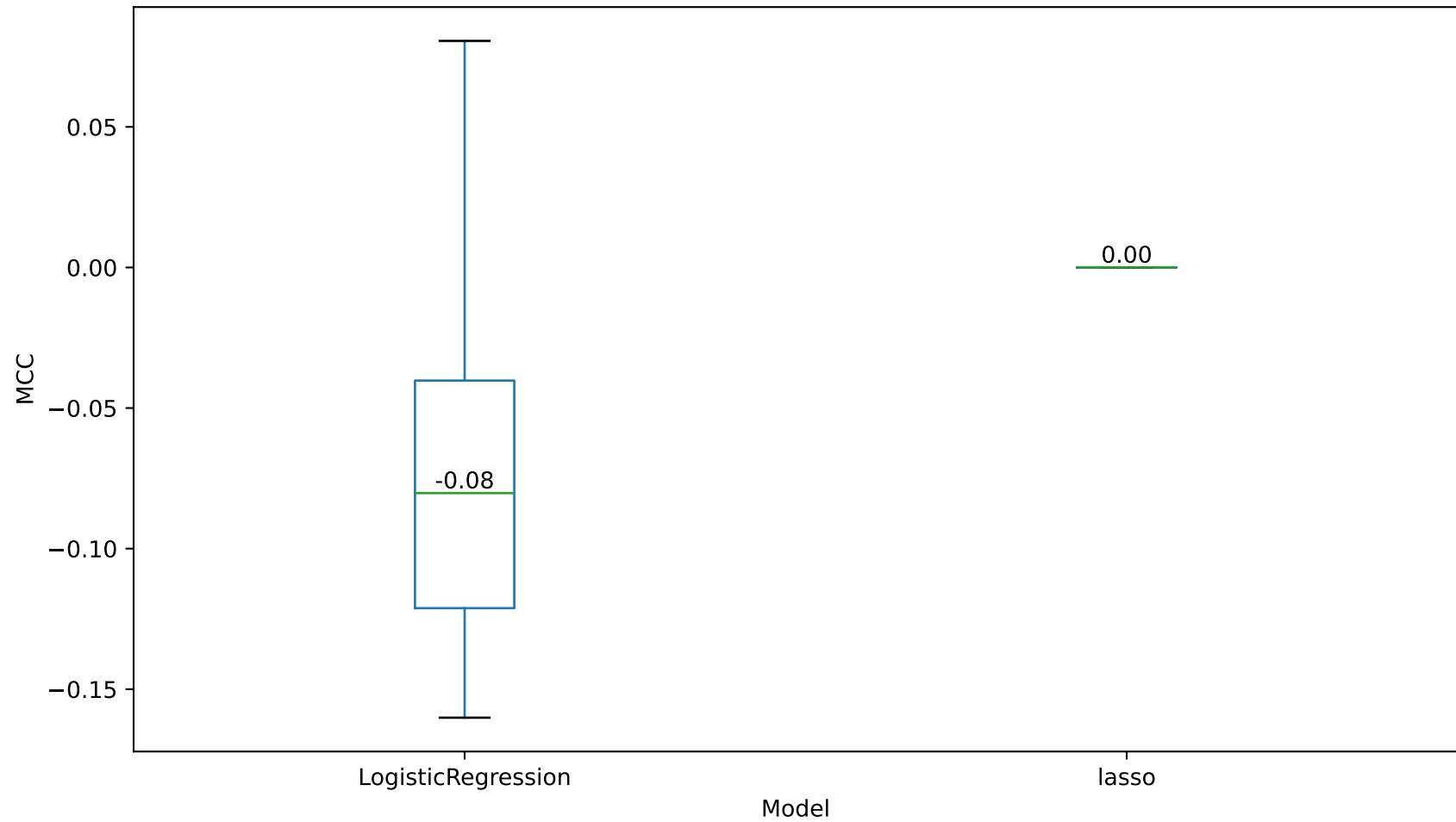
Boxplot for MCC
