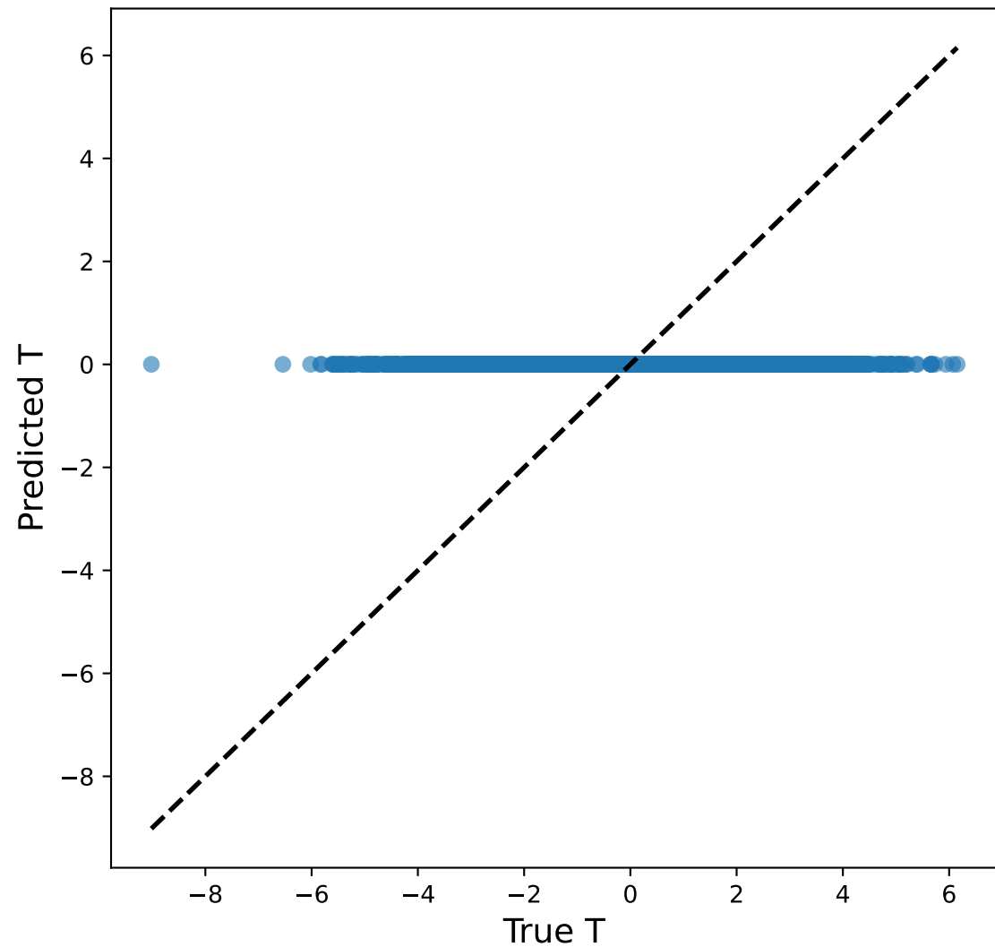
IRM ( \lambda=1000.0 )
