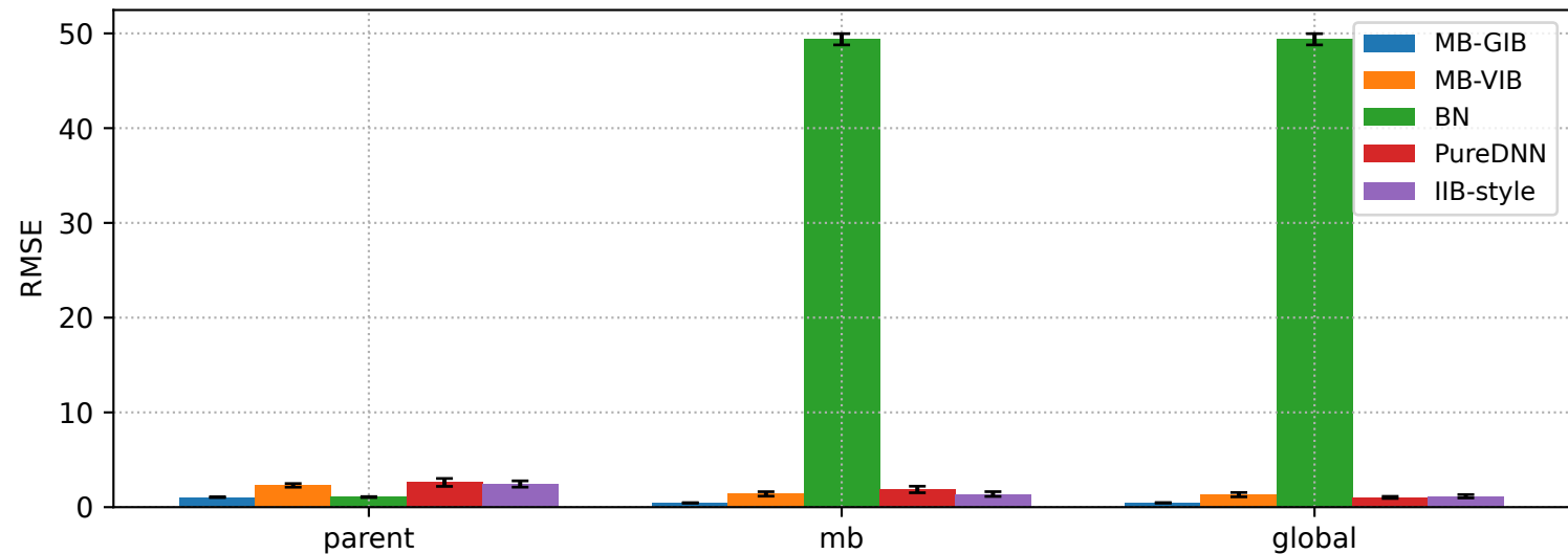
Ablation: Scope — RMSE
