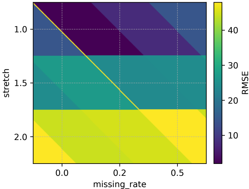
MB-VIB: RMSE — stretch \times miss
