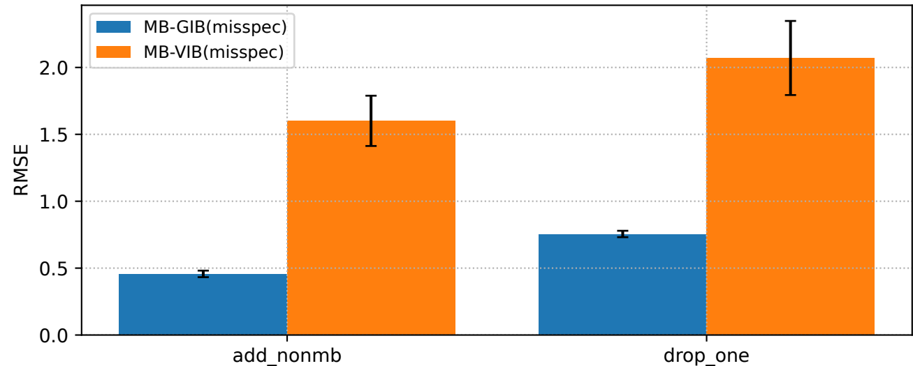
MB Misspecification — RMSE
