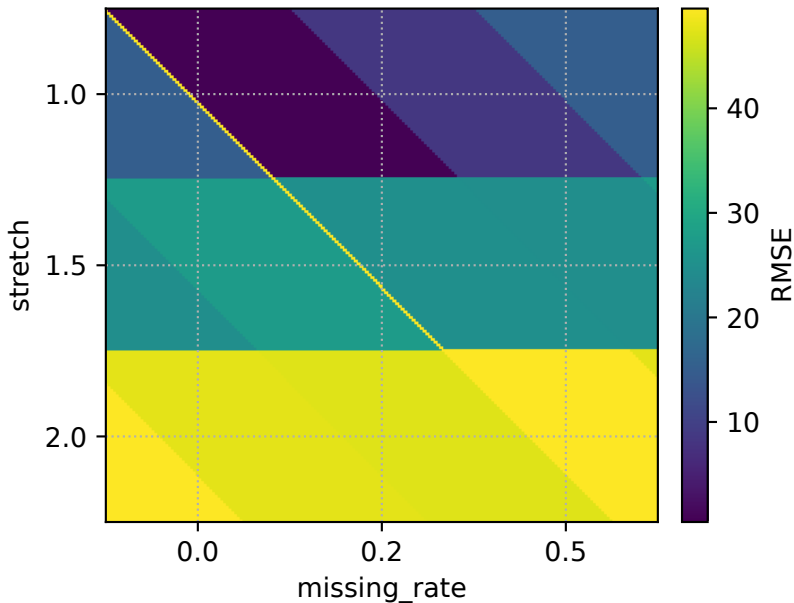
MB-GIB: RMSE — stretch \times miss
