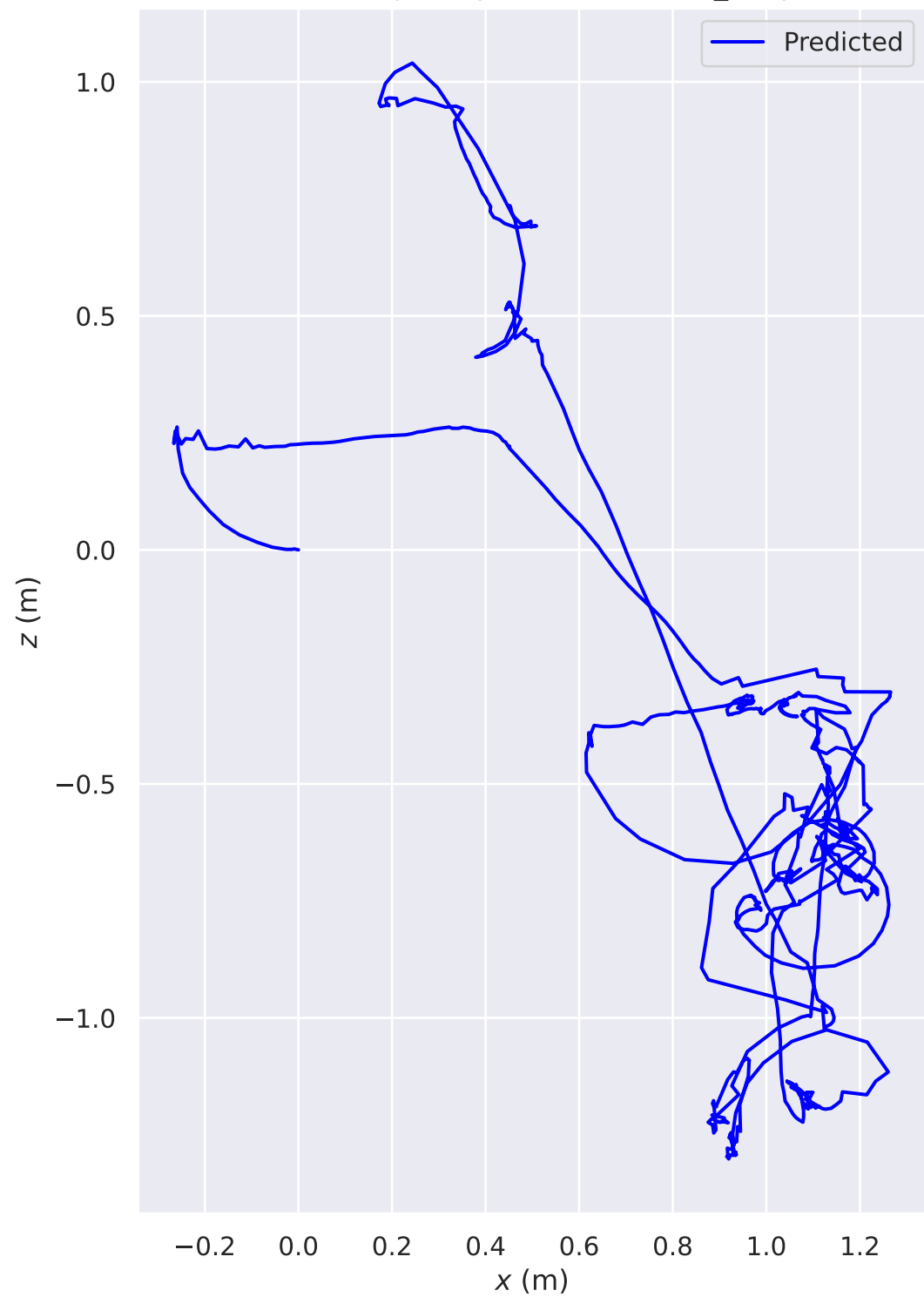
DPVO Trajectory Prediction for 1_body
