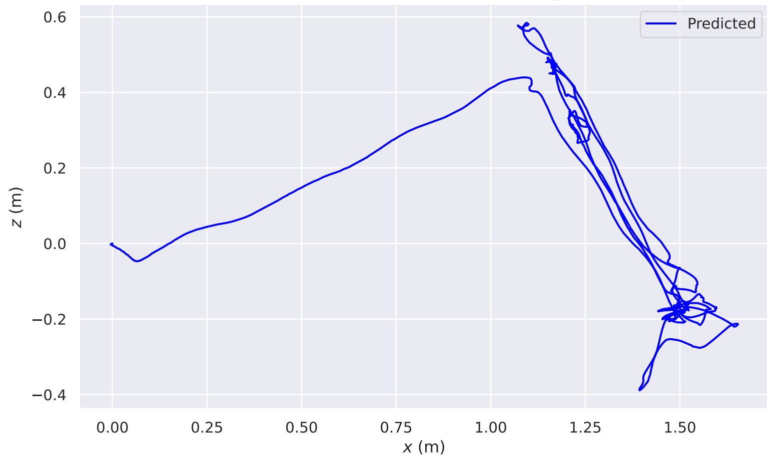
DPVO Trajectory Prediction for kitchen_body
