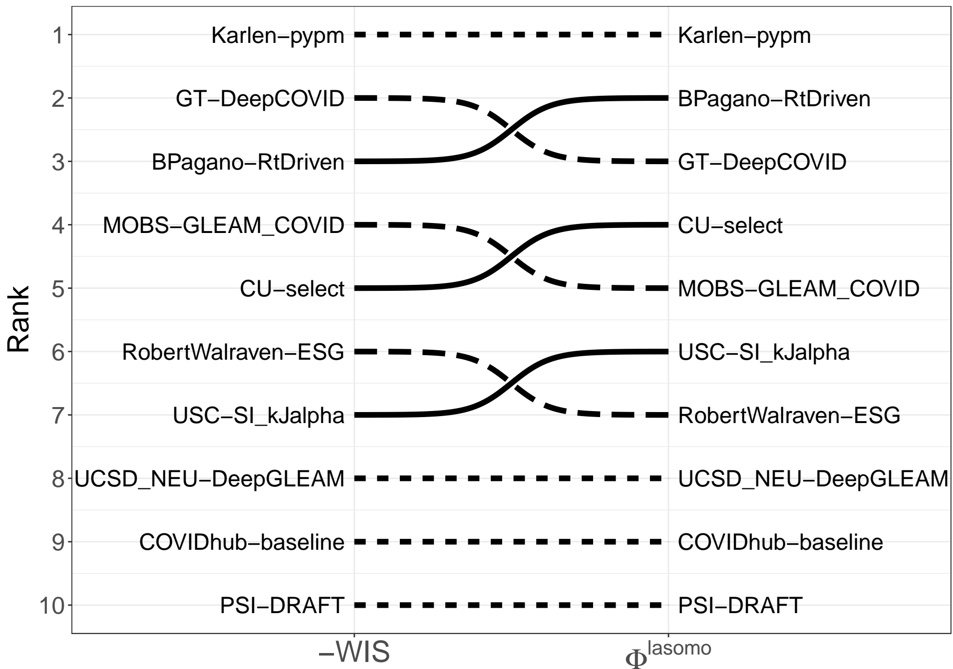
(a) -WIS vs. \Phi^{\text{lasomo}}
