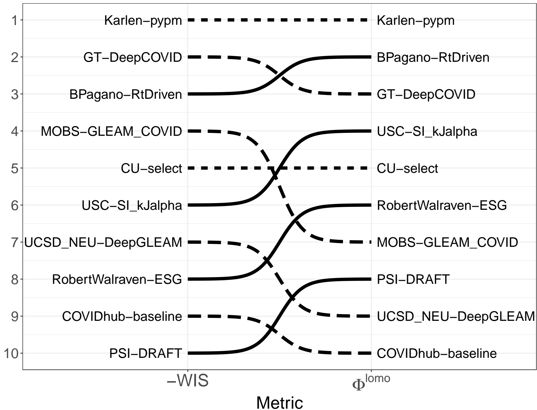
(b) -WIS vs. \Phi^{lomo}
