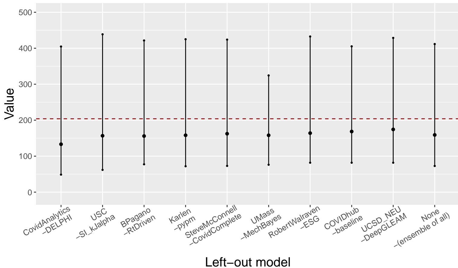
95% Prediction Intervals of Ensembles Built Leaving One Model Out
