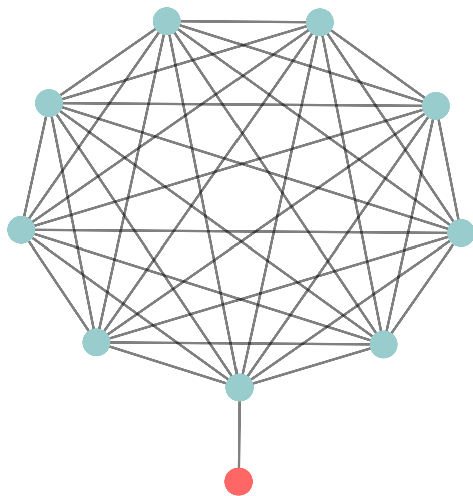
Lollipop graph
