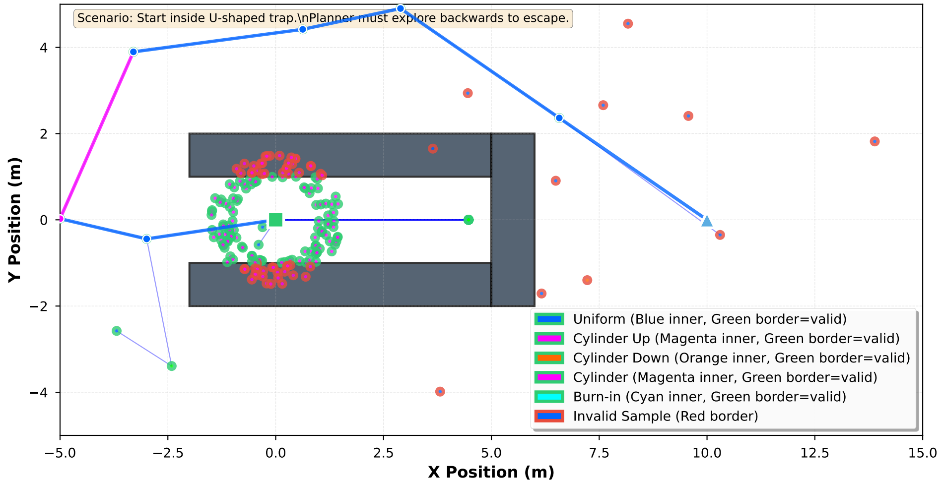
Samples by Sampler Arm (Border Color)
