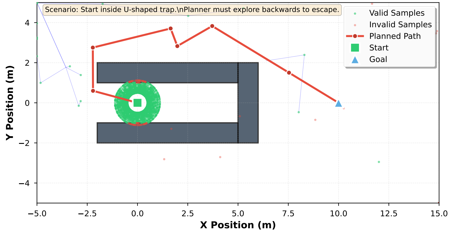
RRT Tree with Valid/Invalid Samples
