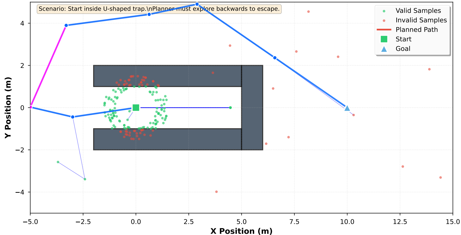
RRT Tree with Valid/Invalid Samples
