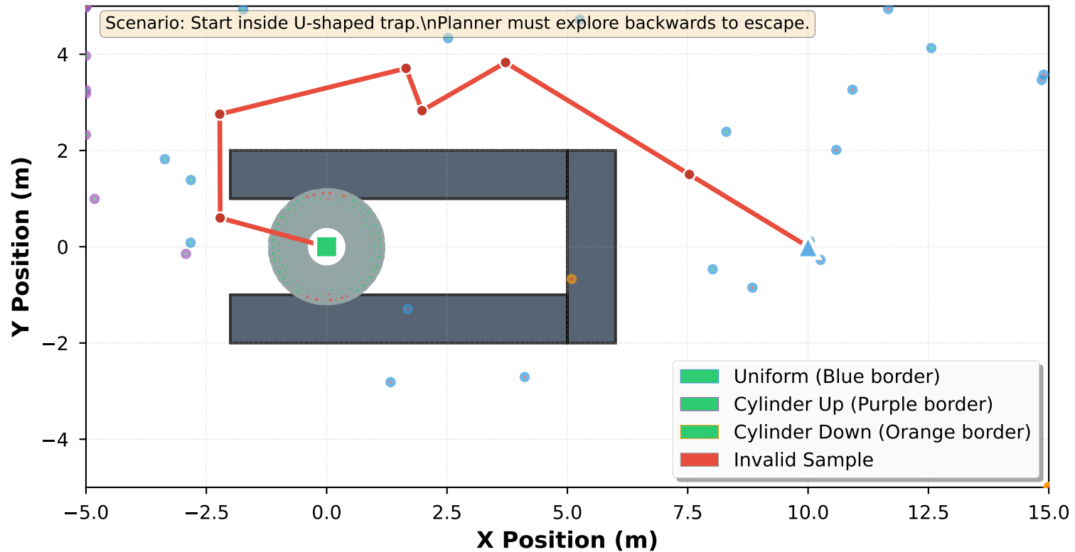
Samples by Sampler Arm (Border Color)
