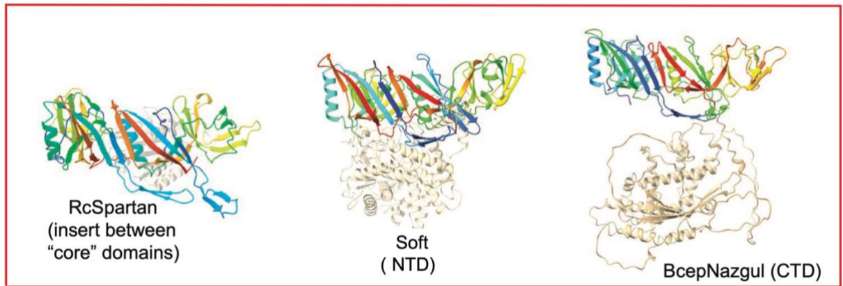
Fig.S1. Examples of MP22-like DTNs with large extra domains.
