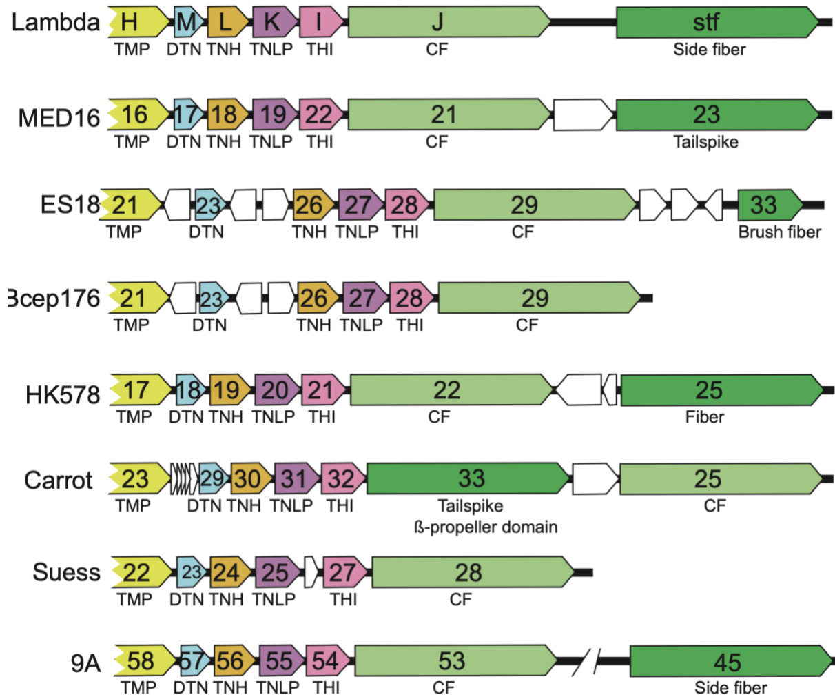
Figure S3A. Lambda-like tail tip gene clusters.
