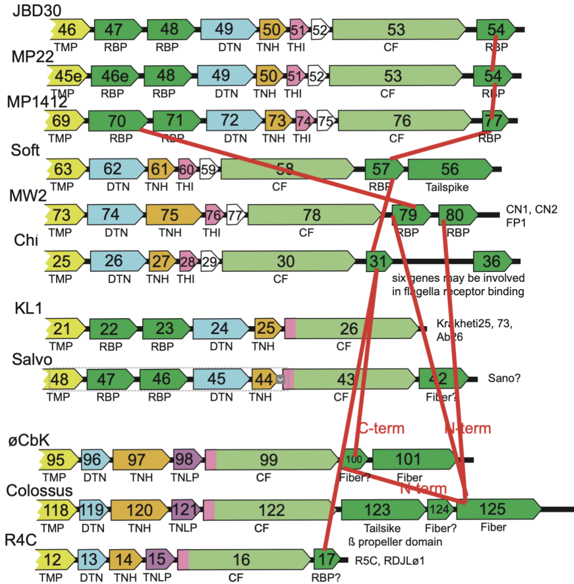
Figure S3C. MP22-like, KL1-like, and \sigma CbK tail tip gene clusters.
