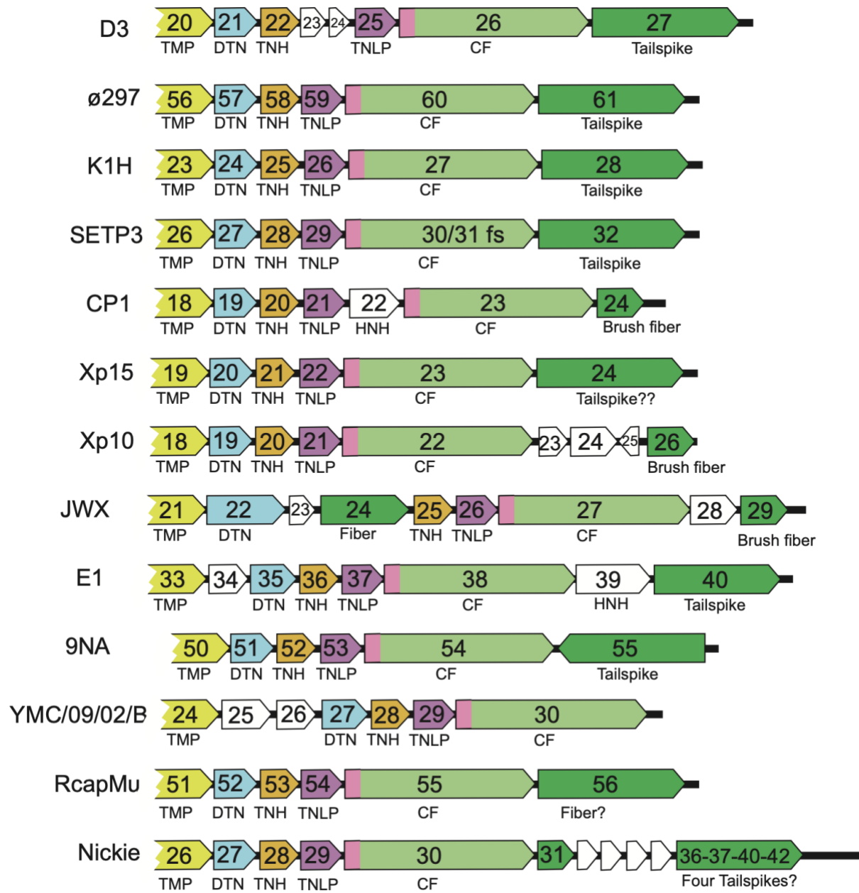
Figure S3B. D3-like tail tip gene clusters.
