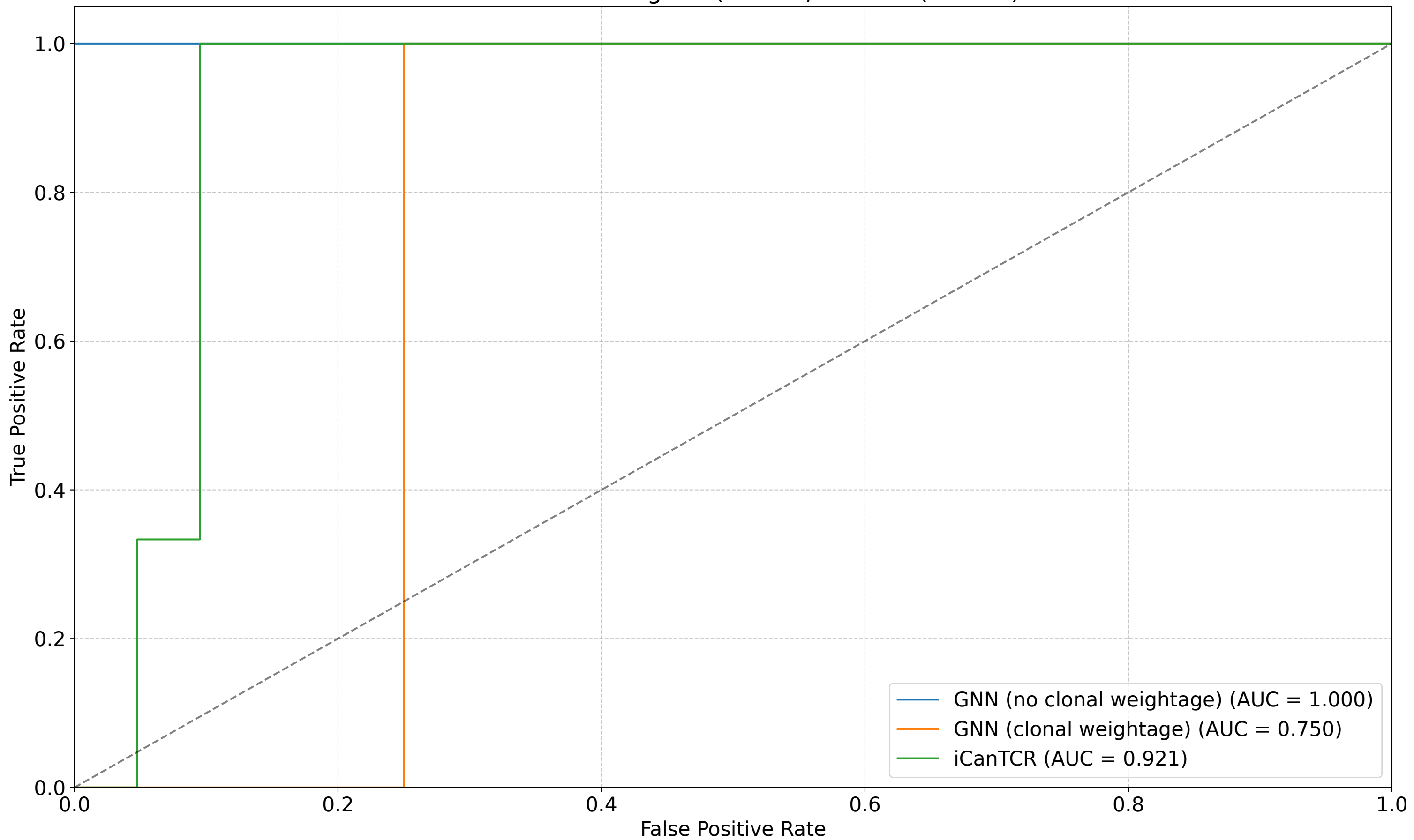
ROC Curve: seekgene (cancer) vs PICA (control)
