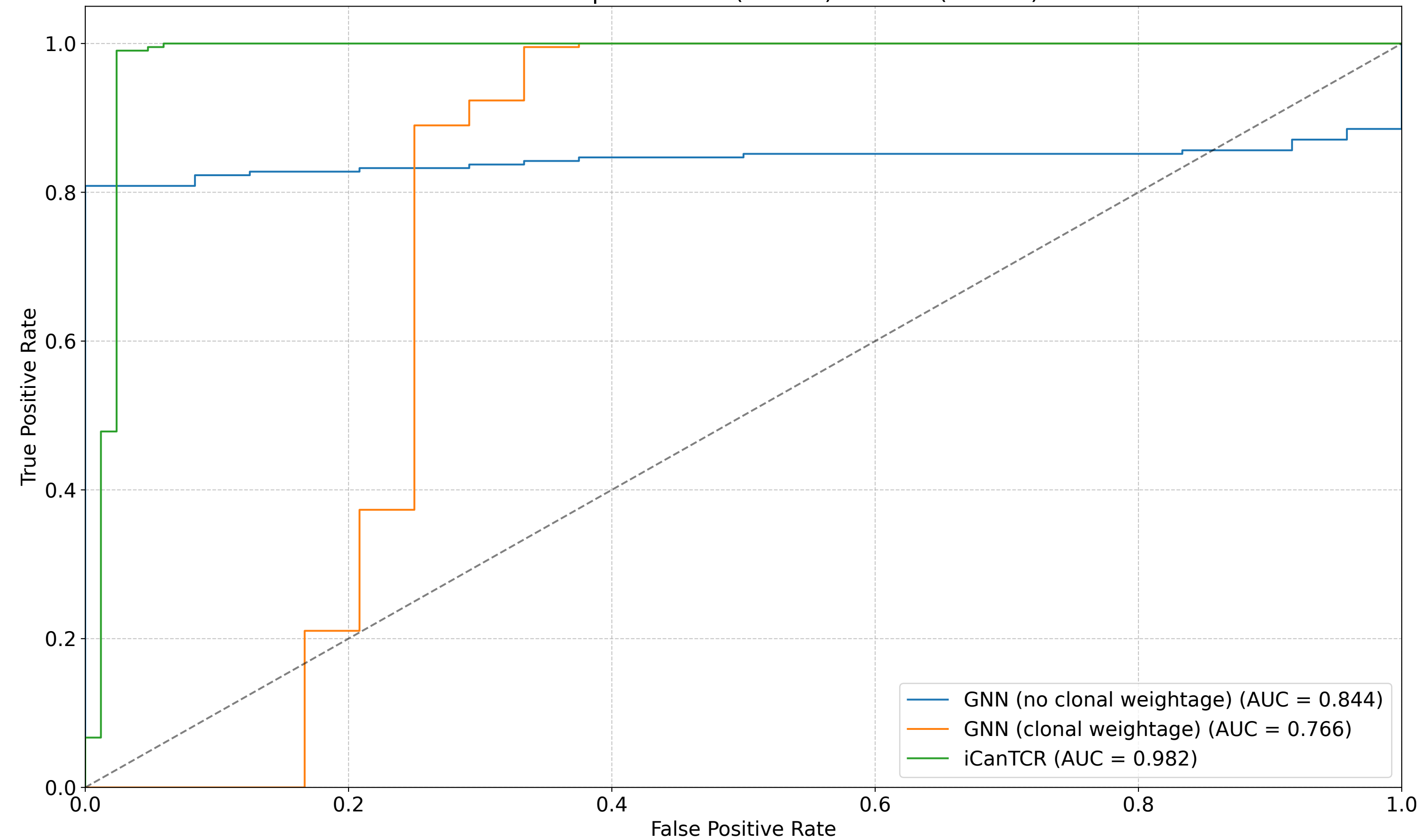
ROC Curve: phs002517 (cancer) vs PICA (control)
