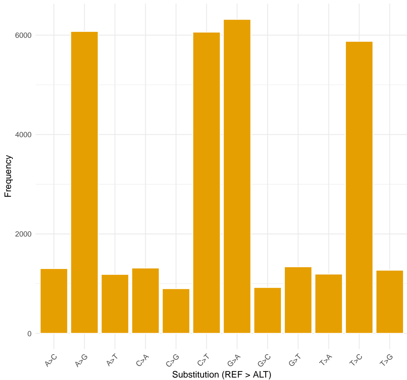
SNP Substitution Spectrum Distribution of observed SNP mutation classes
