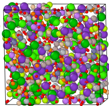
Noisy Sample
