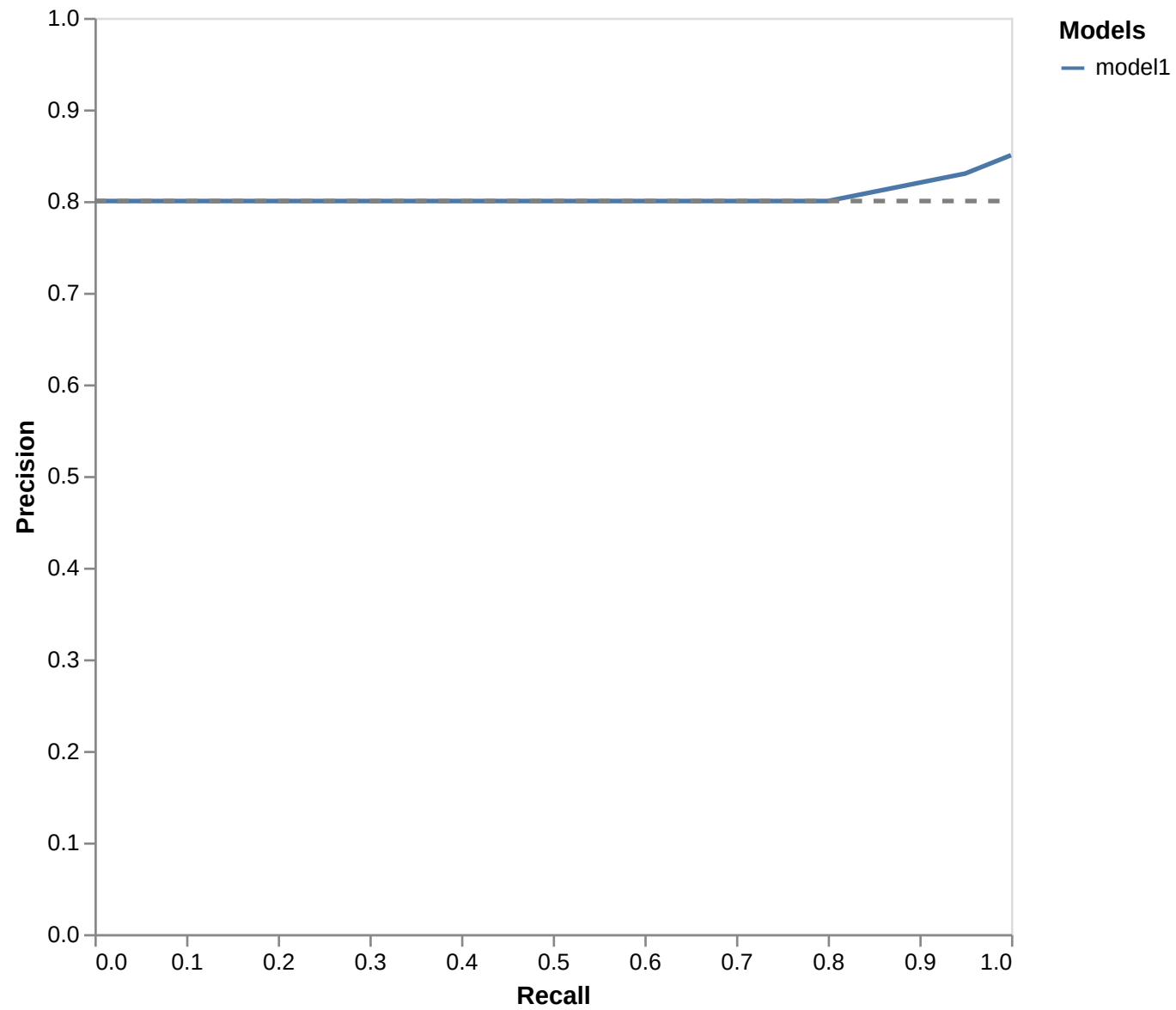
PR Curve
