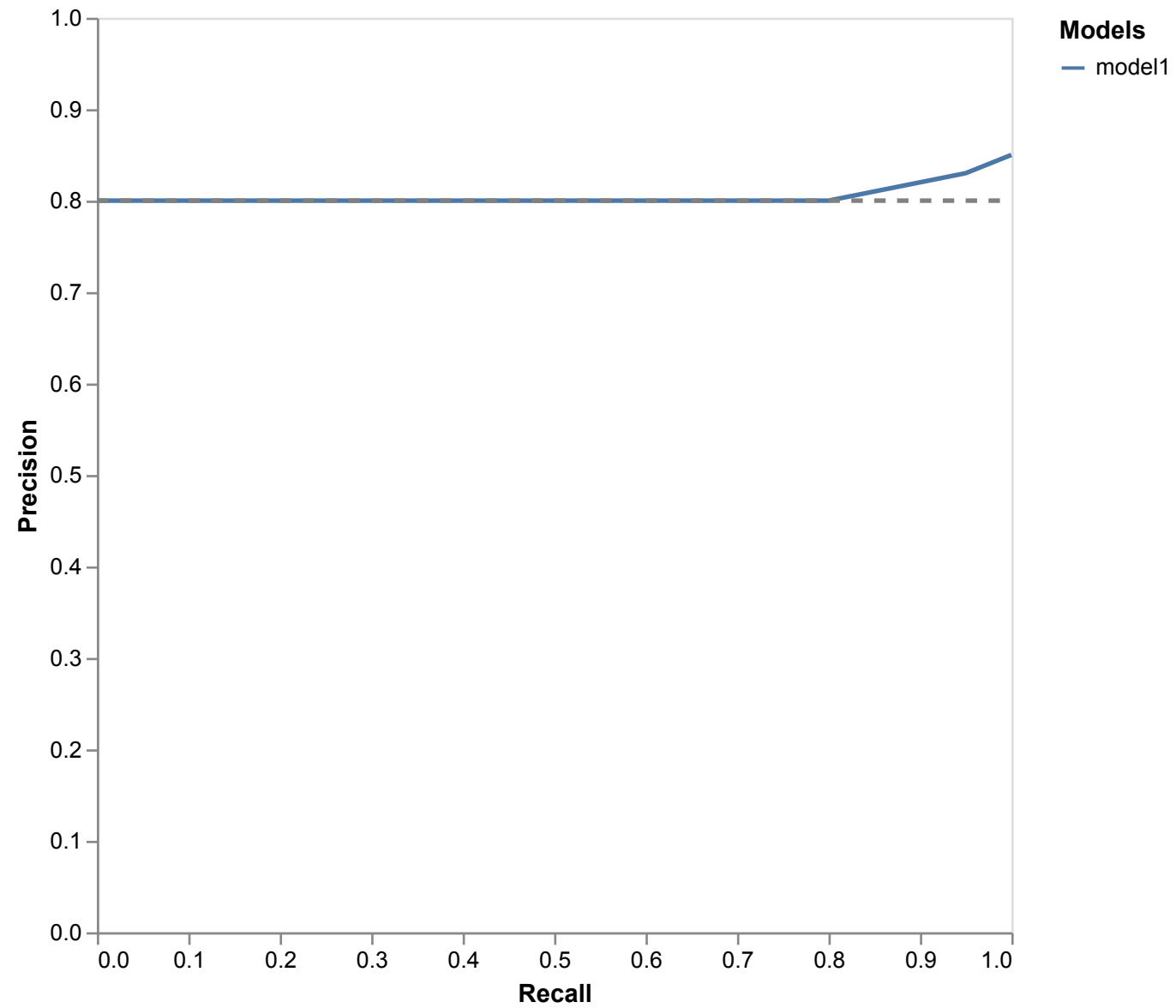
PR Curve
