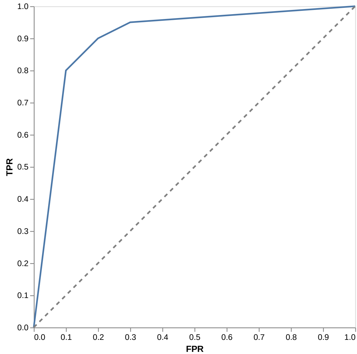
ROC Curve
