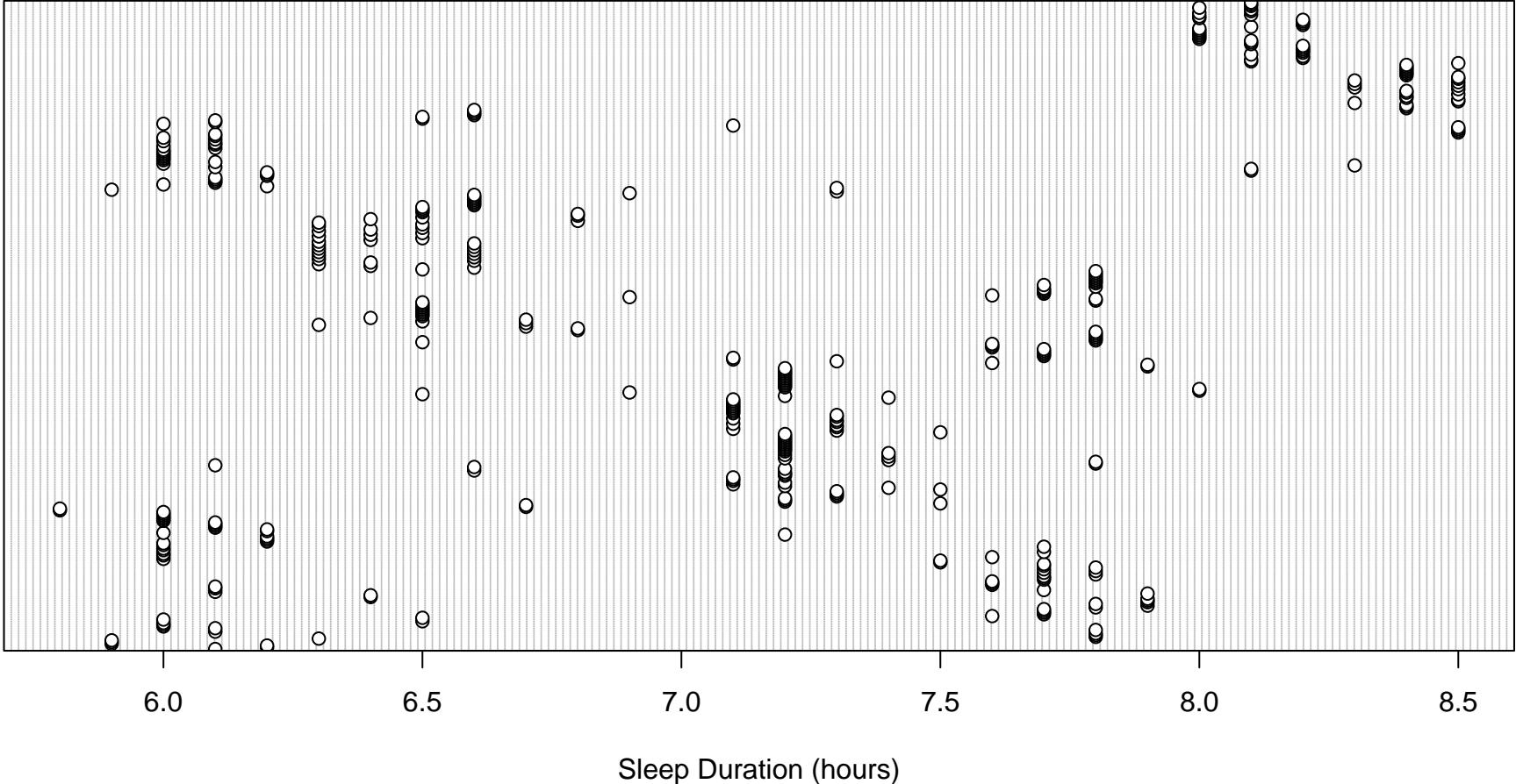
Dotplot of Sleep Duration
