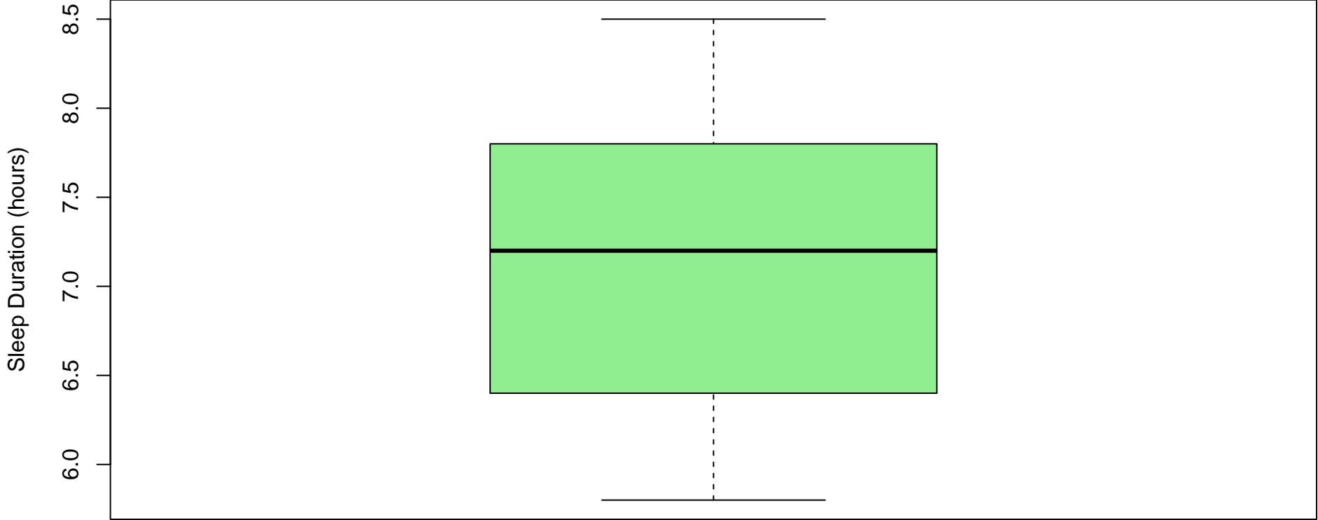
Boxplot of Sleep Duration
