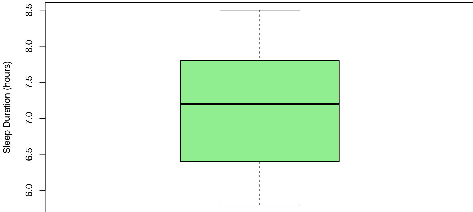
Boxplot of Sleep Duration
