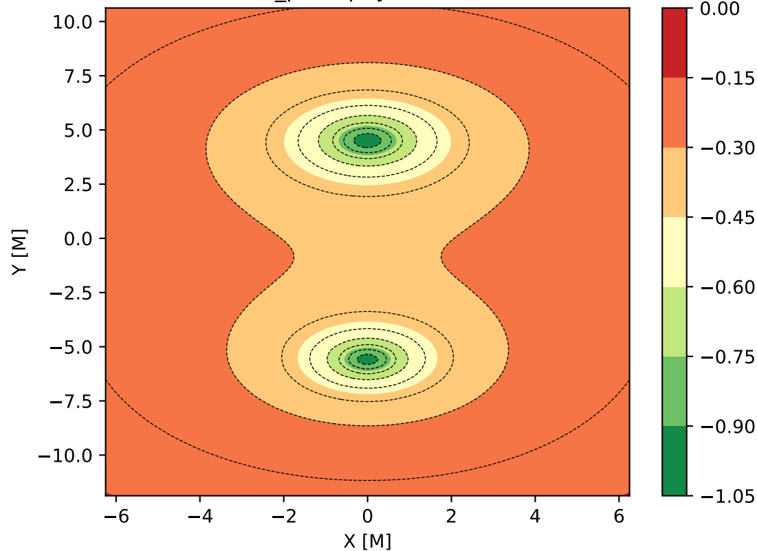
Lev05-00_phi0 physical time = 0.0
