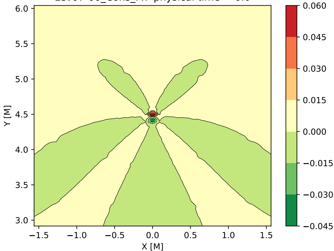
Lev07-00_Cons_Px physical time = 0.0
