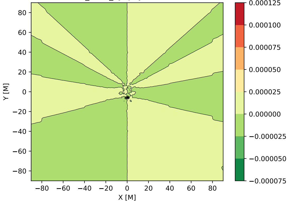
Lev02-00_Cons_Py physical time = 0.0
