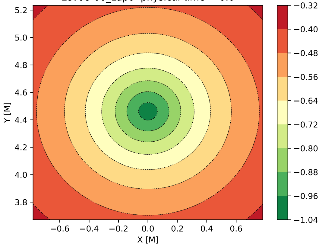
Lev08-00_Lap0 physical time = 0.0
