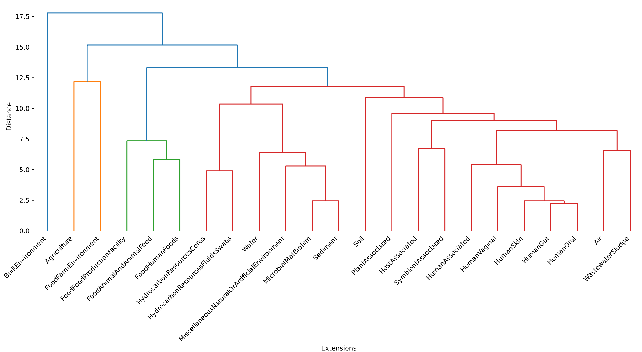
Similarity of MlxS Extensions by Term Usage
