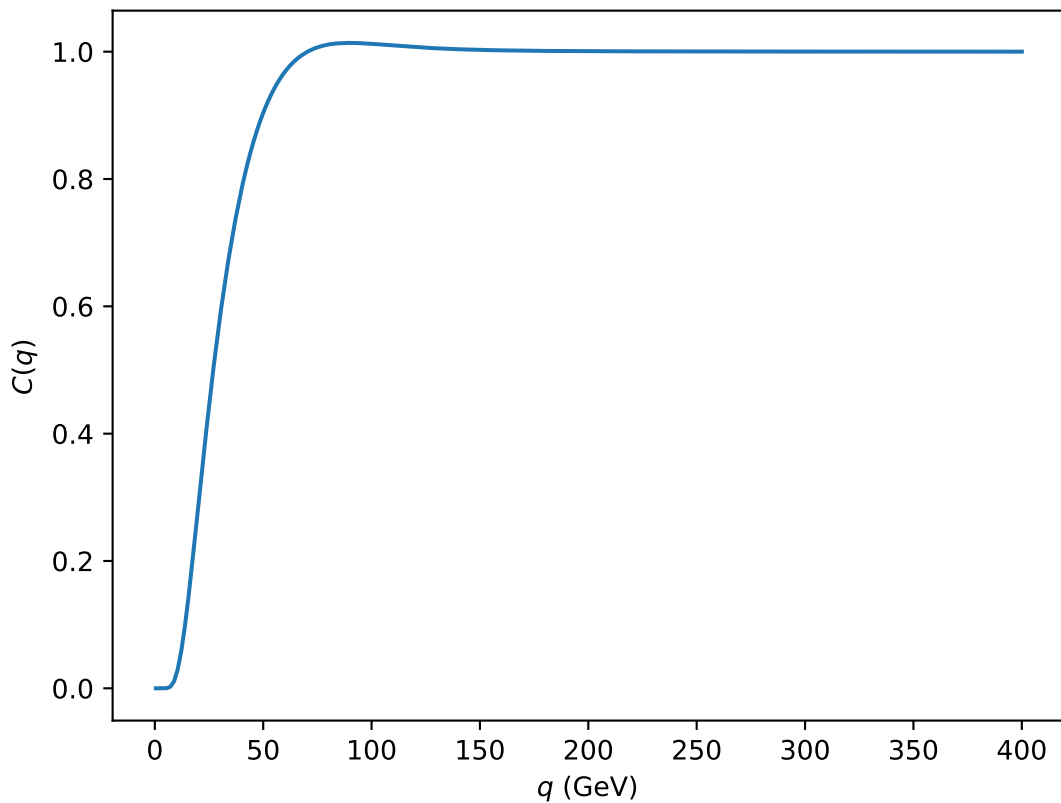
Coulomb Correlation, Gaussian source R=5.0 fm
