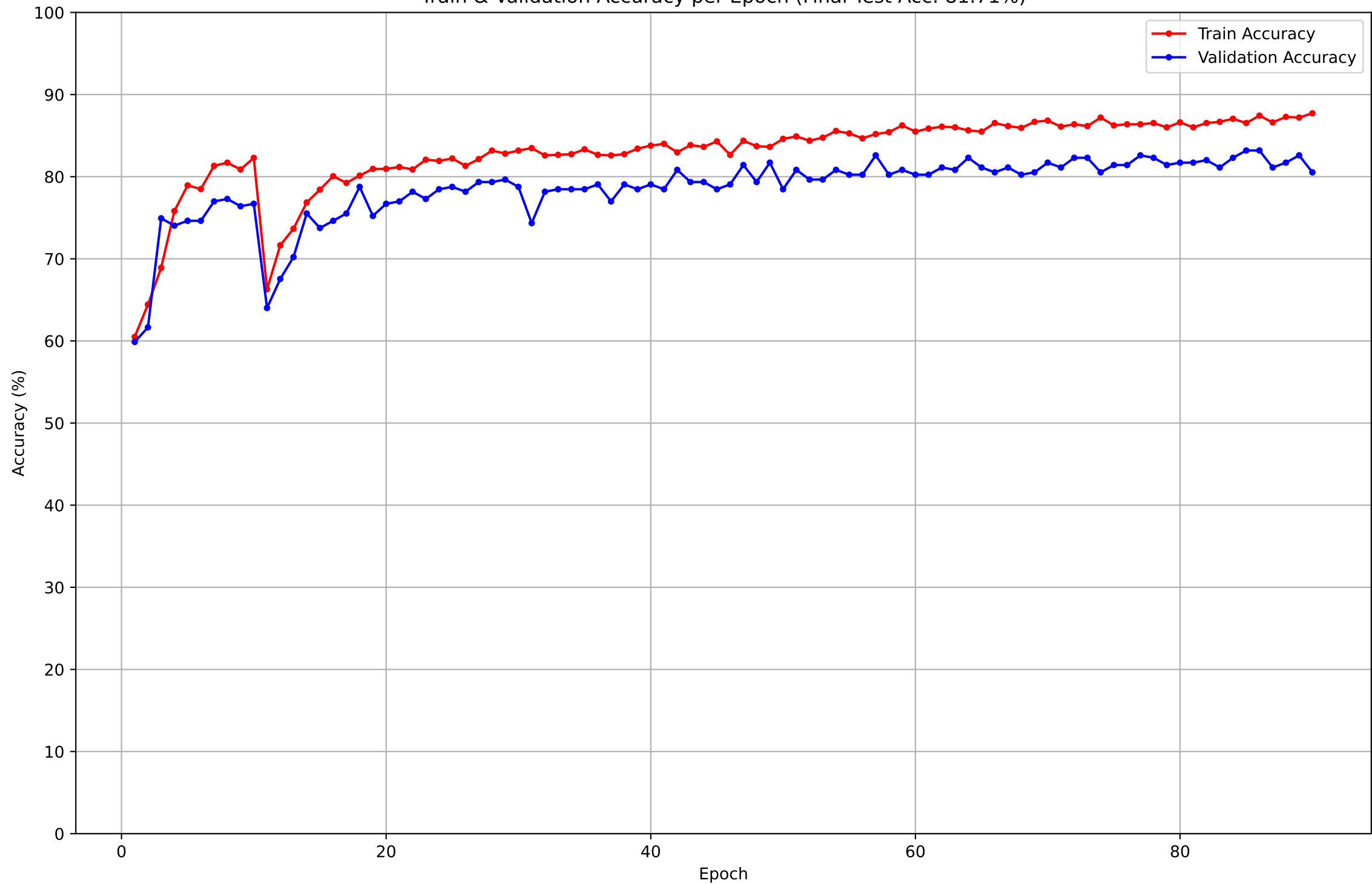
Train & Validation Accuracy per Epoch (Final Test Acc: 81.71%)
