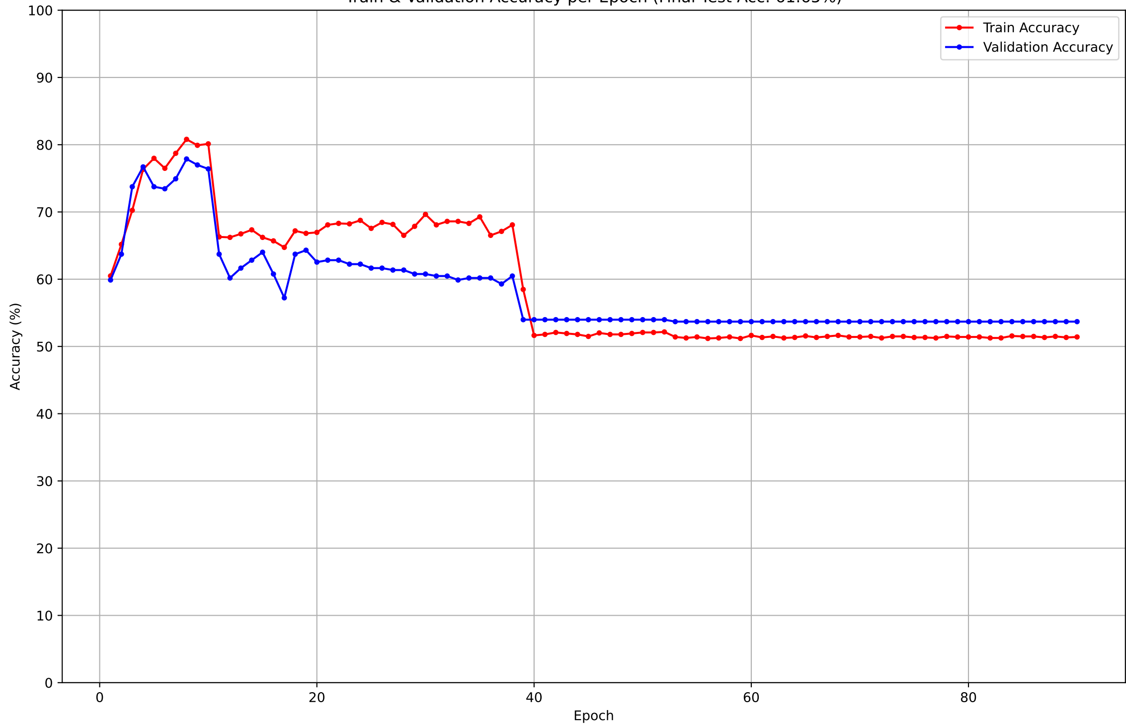
Train & Validation Accuracy per Epoch (Final Test Acc: 61.65%)
