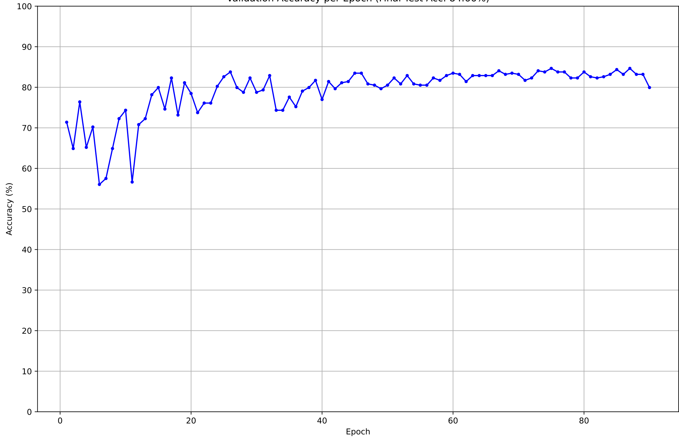
Validation Accuracy per Epoch (Final Test Acc: 84.66%)
