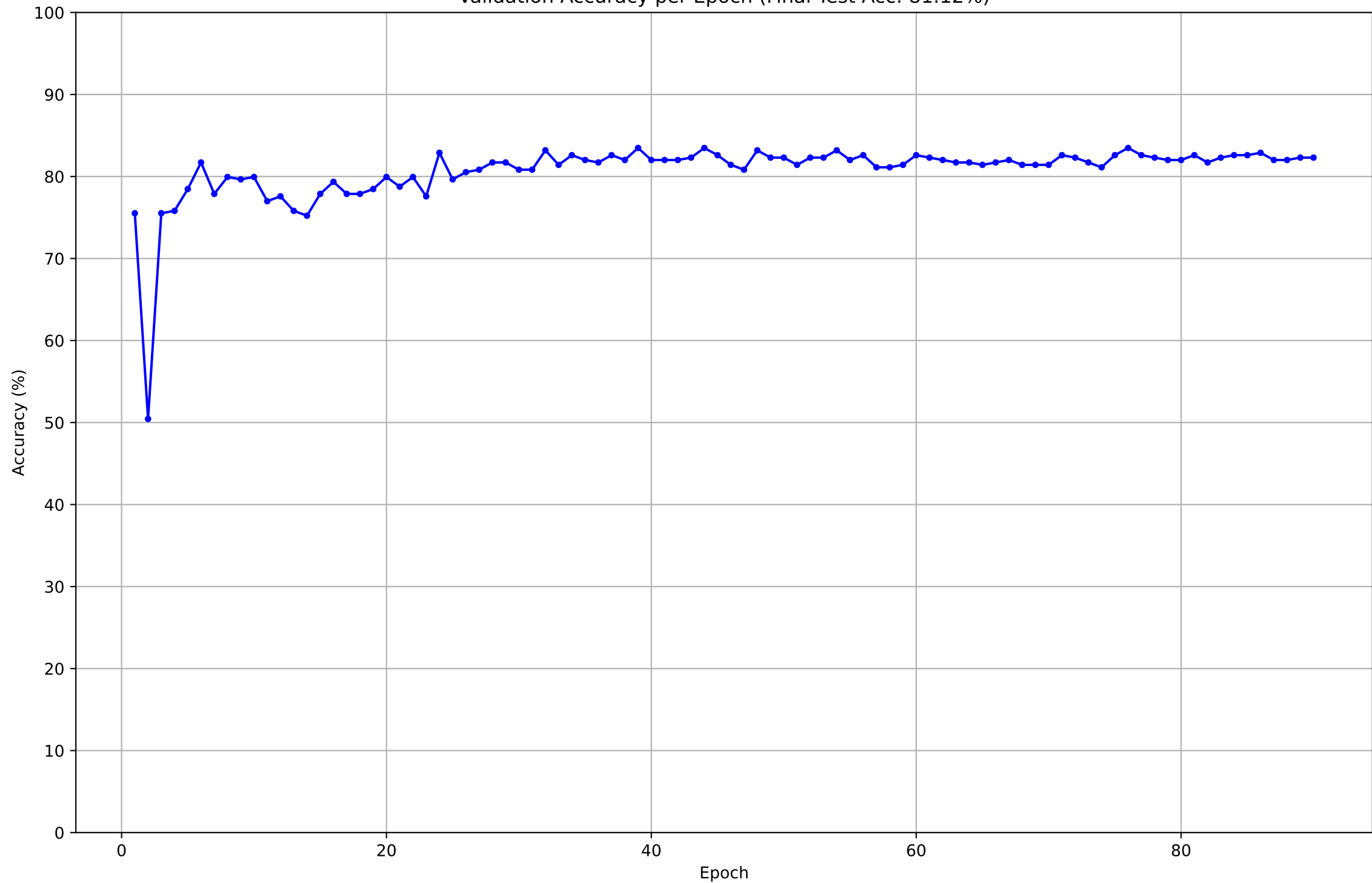
Validation Accuracy per Epoch (Final Test Acc: 81.12%)
