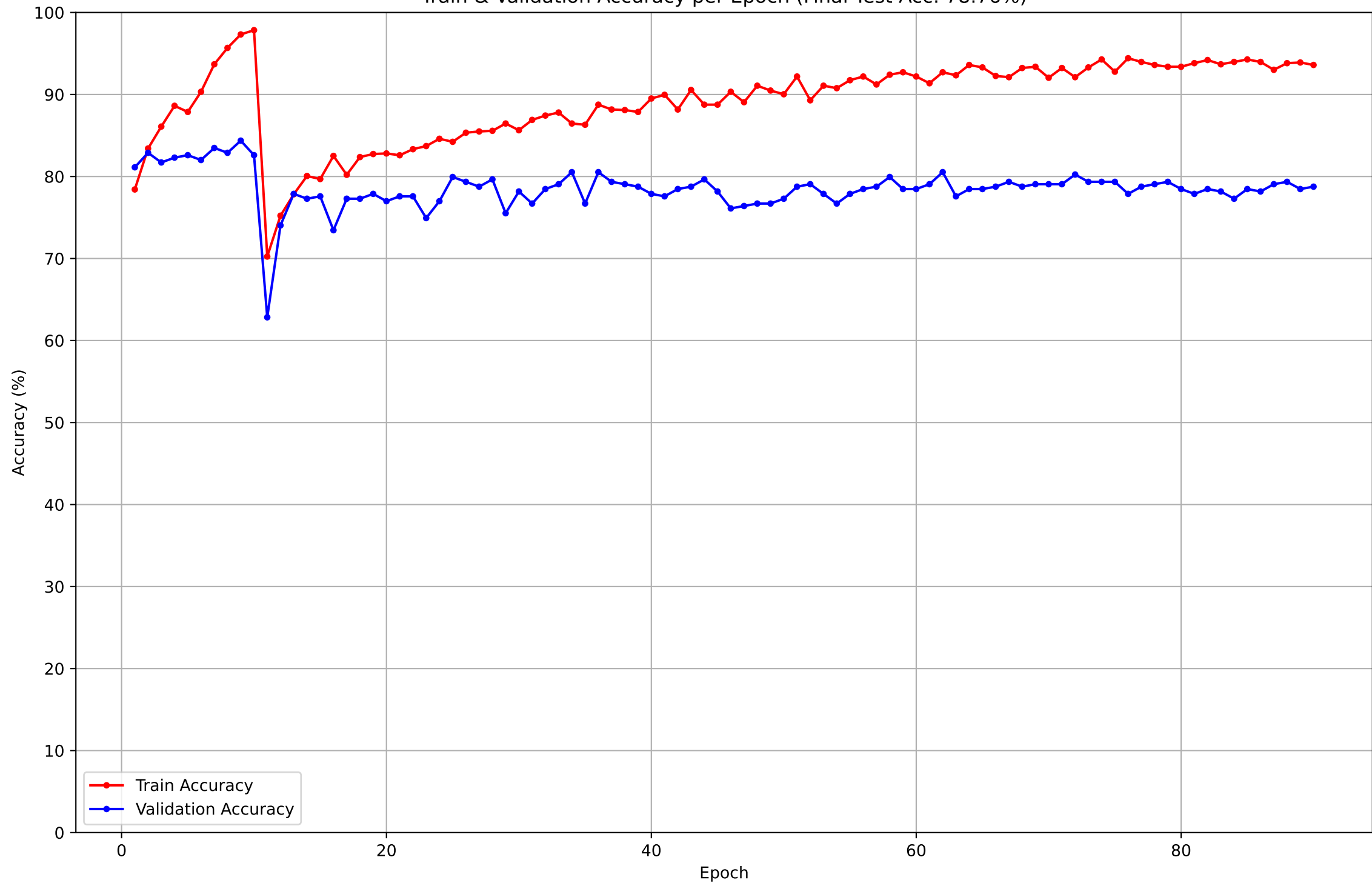
Train & Validation Accuracy per Epoch (Final Test Acc: 78.76%)
