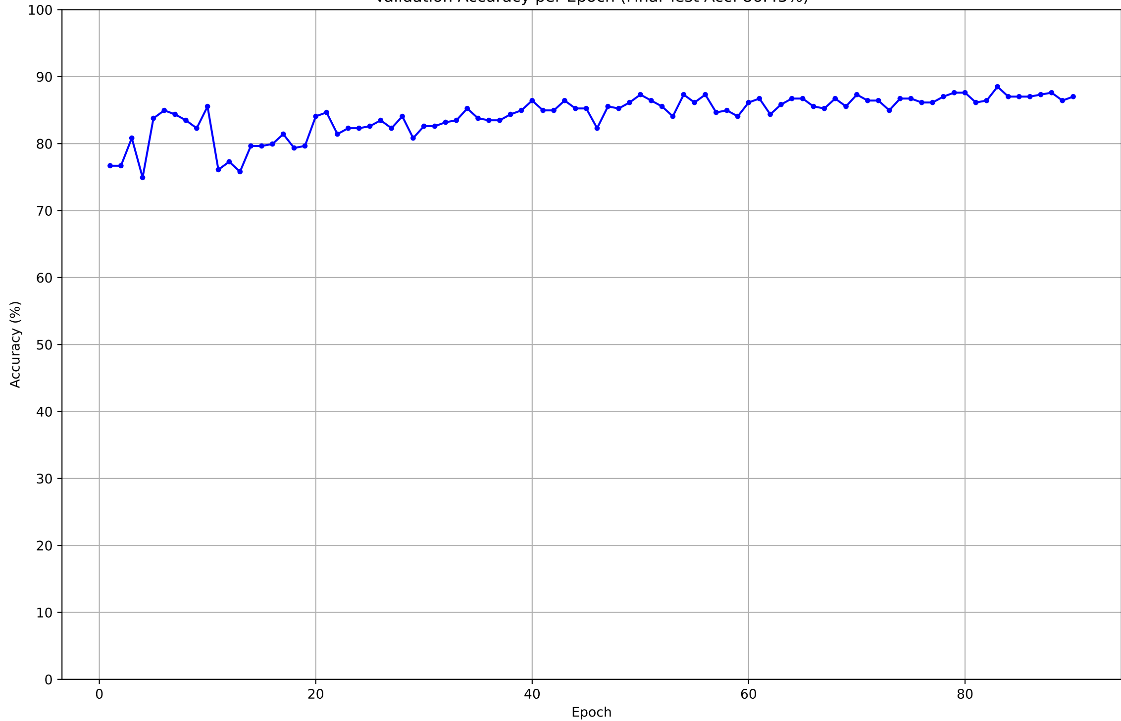
Validation Accuracy per Epoch (Final Test Acc: 86.43%)
