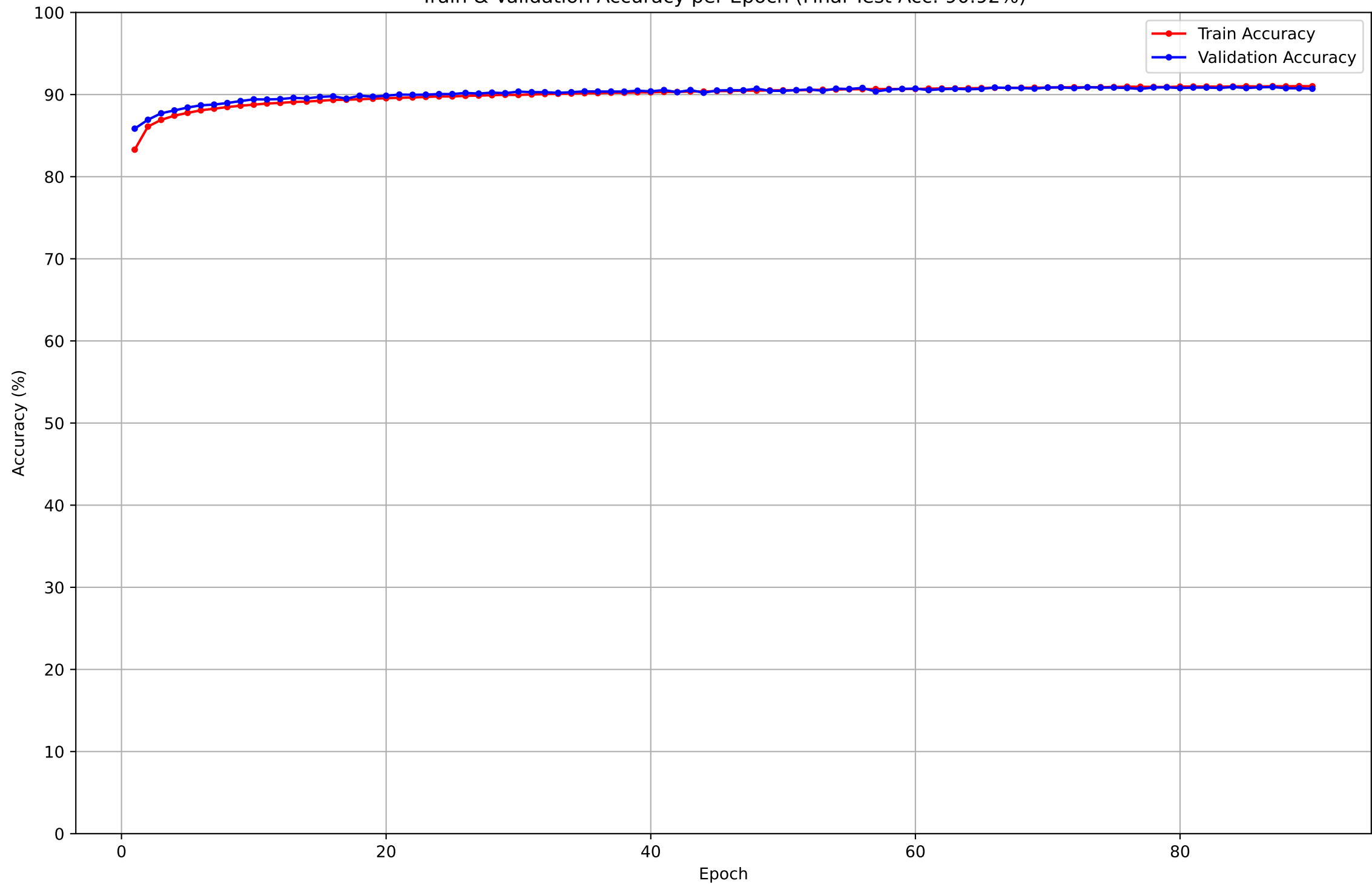
Train & Validation Accuracy per Epoch (Final Test Acc: 90.92%)
