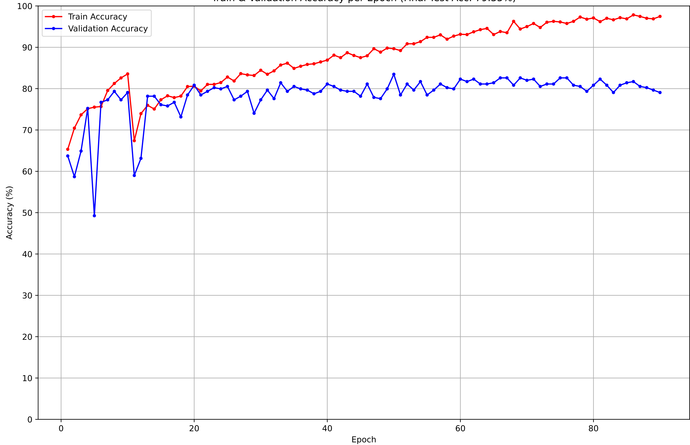
Train & Validation Accuracy per Epoch (Final Test Acc: 79.35%)
