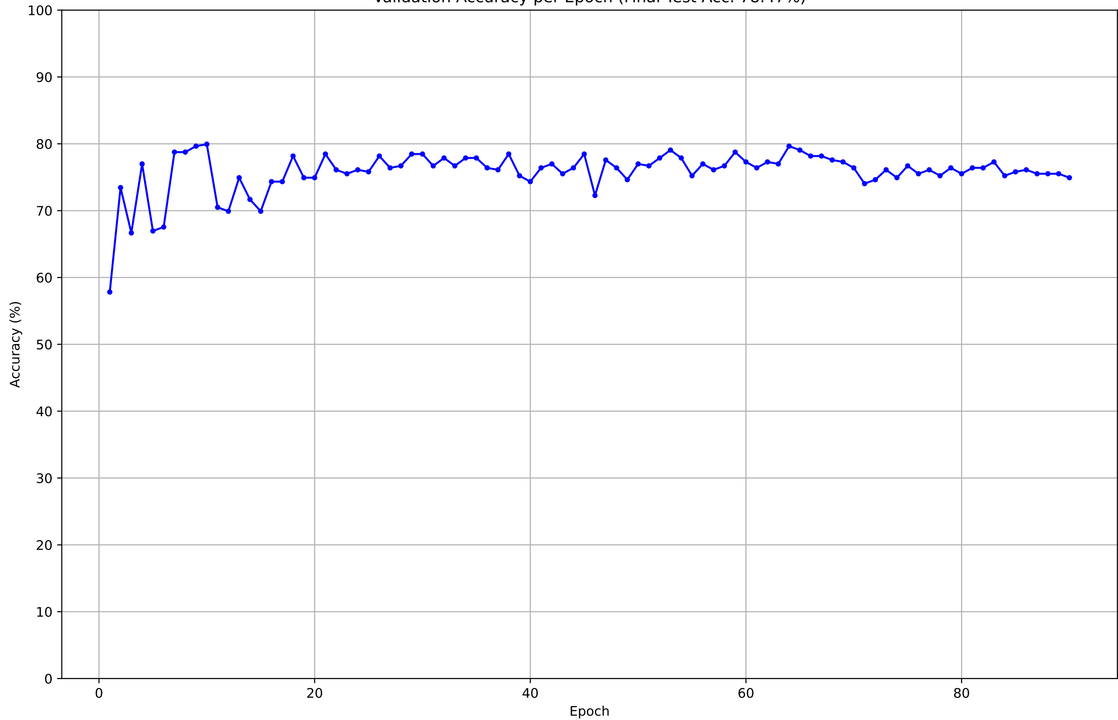
Validation Accuracy per Epoch (Final Test Acc: 78.47%)
