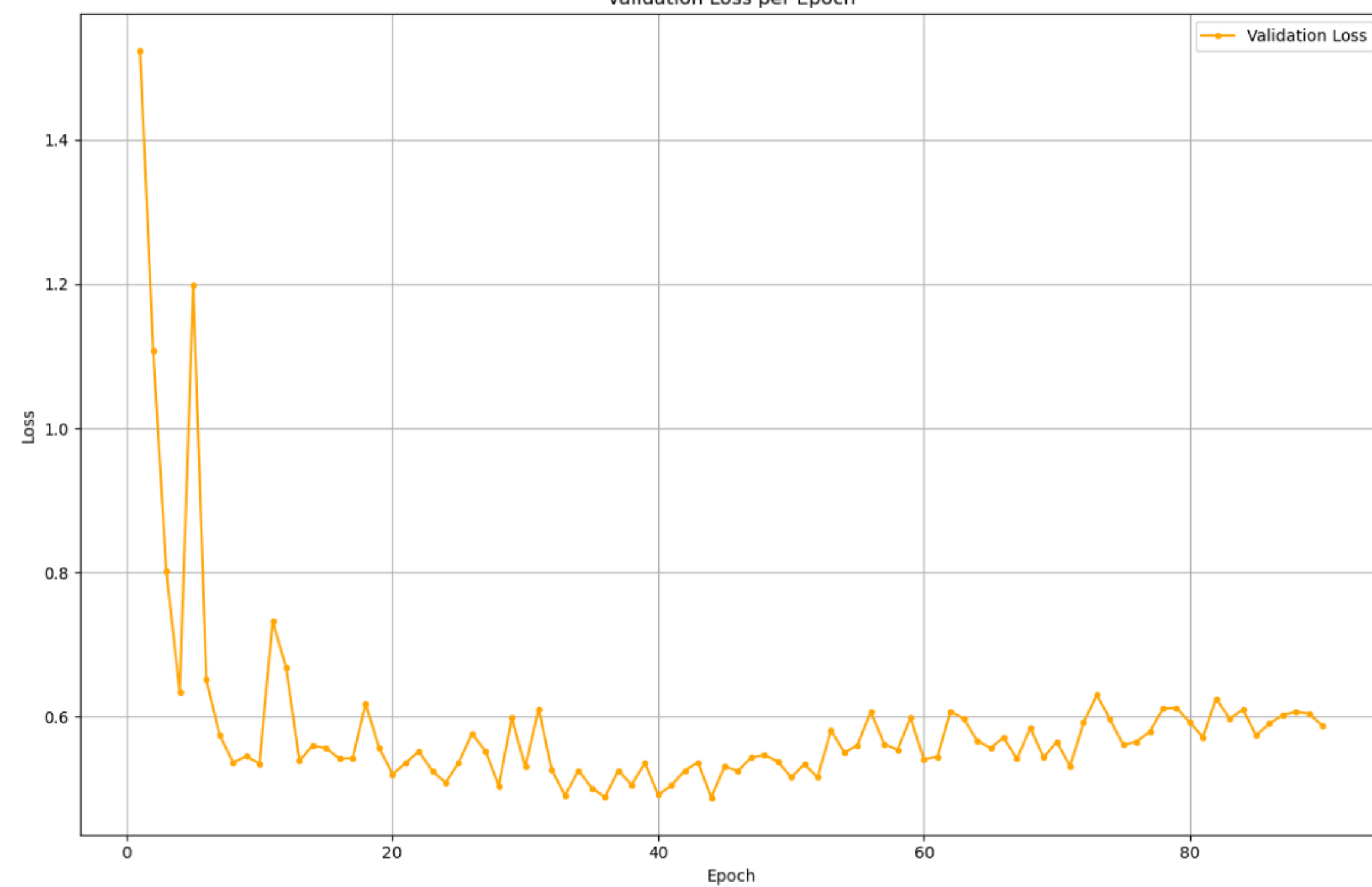
Validation Loss
