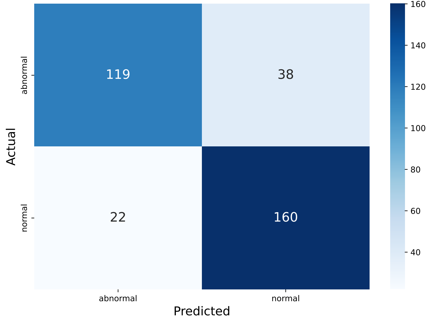
Confusion Matrix
