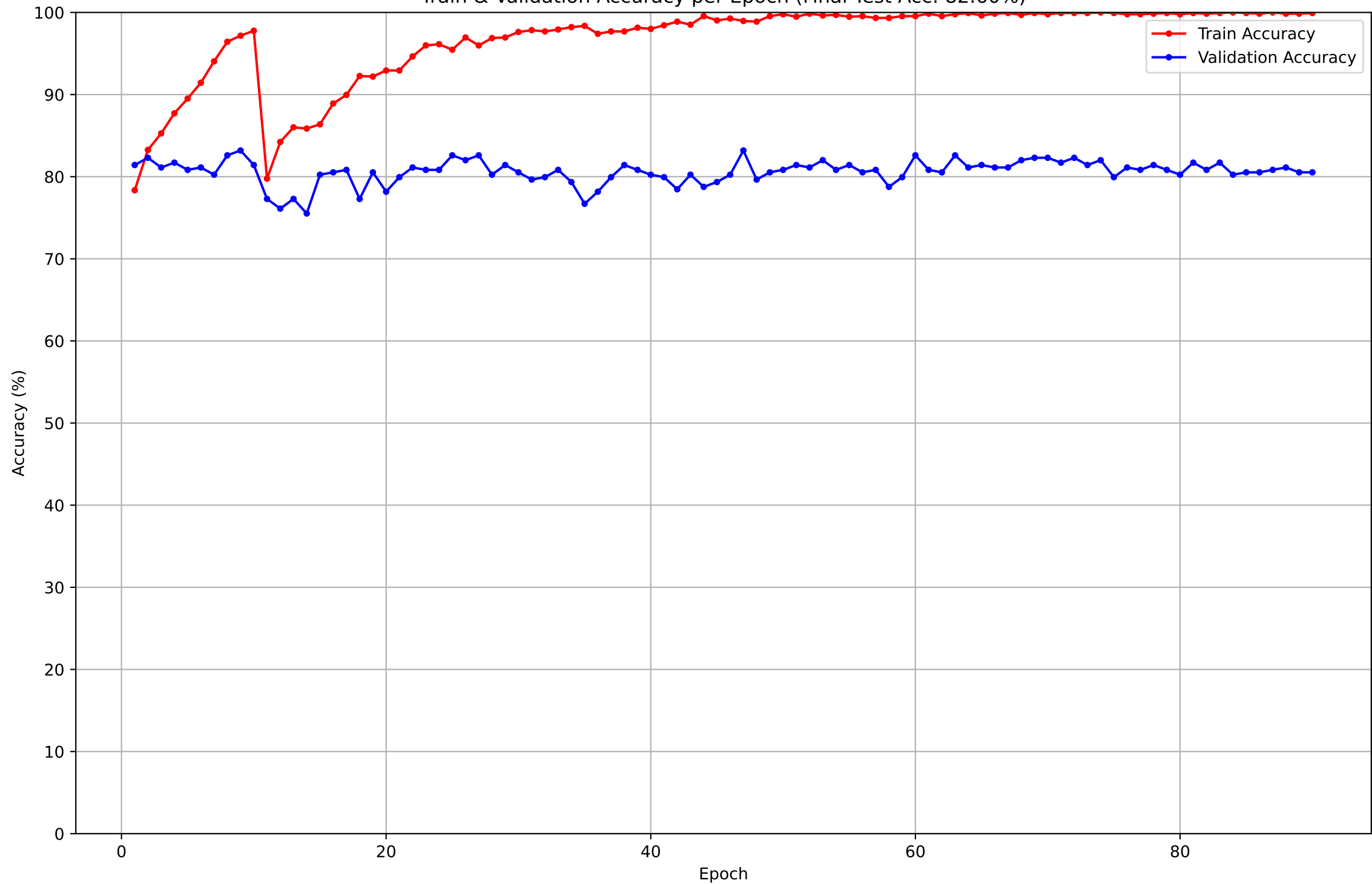
Train & Validation Accuracy per Epoch (Final Test Acc: 82.60%)
