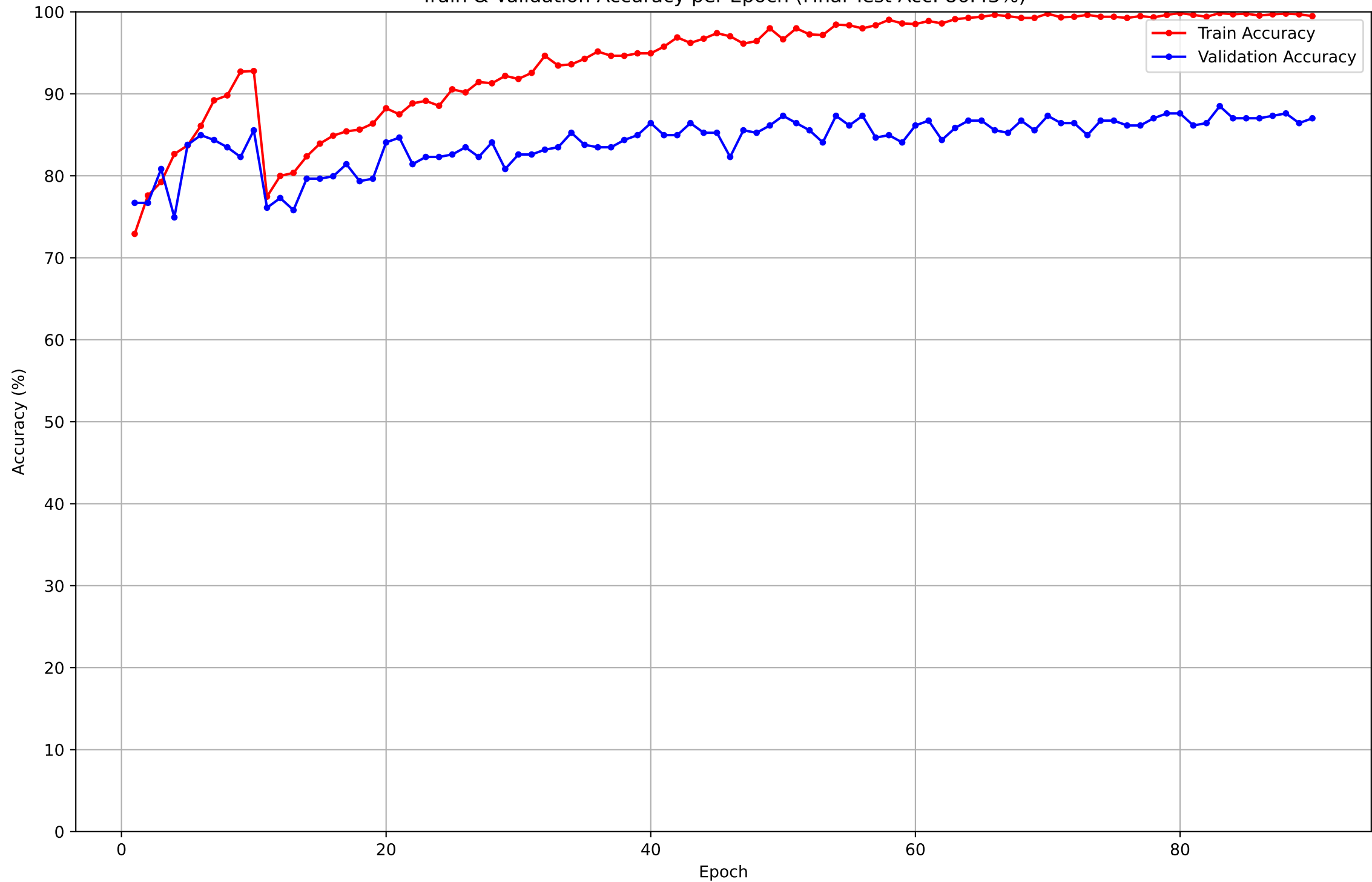
Train & Validation Accuracy per Epoch (Final Test Acc: 86.43%)
