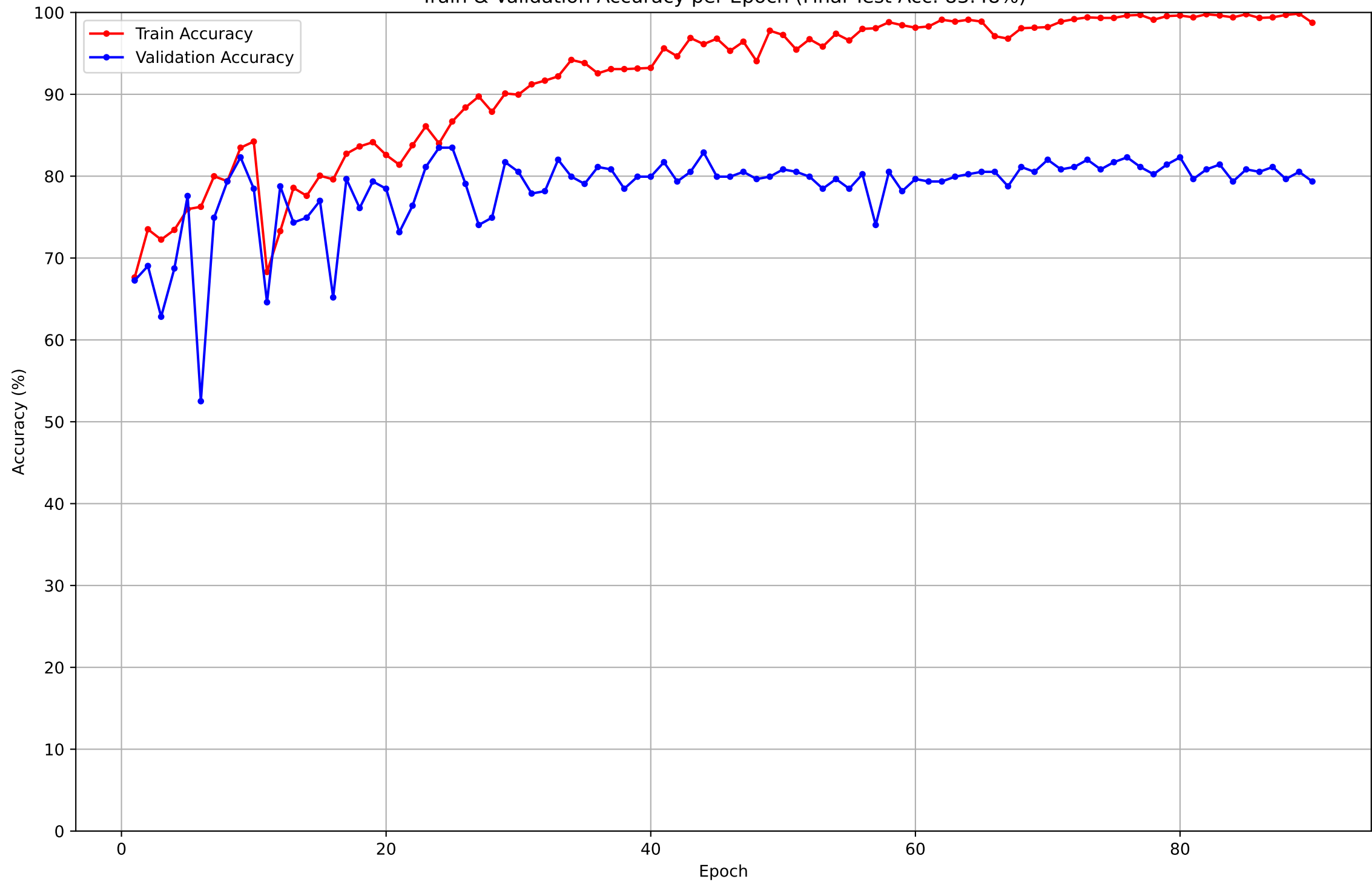
Train & Validation Accuracy per Epoch (Final Test Acc: 83.48%)
