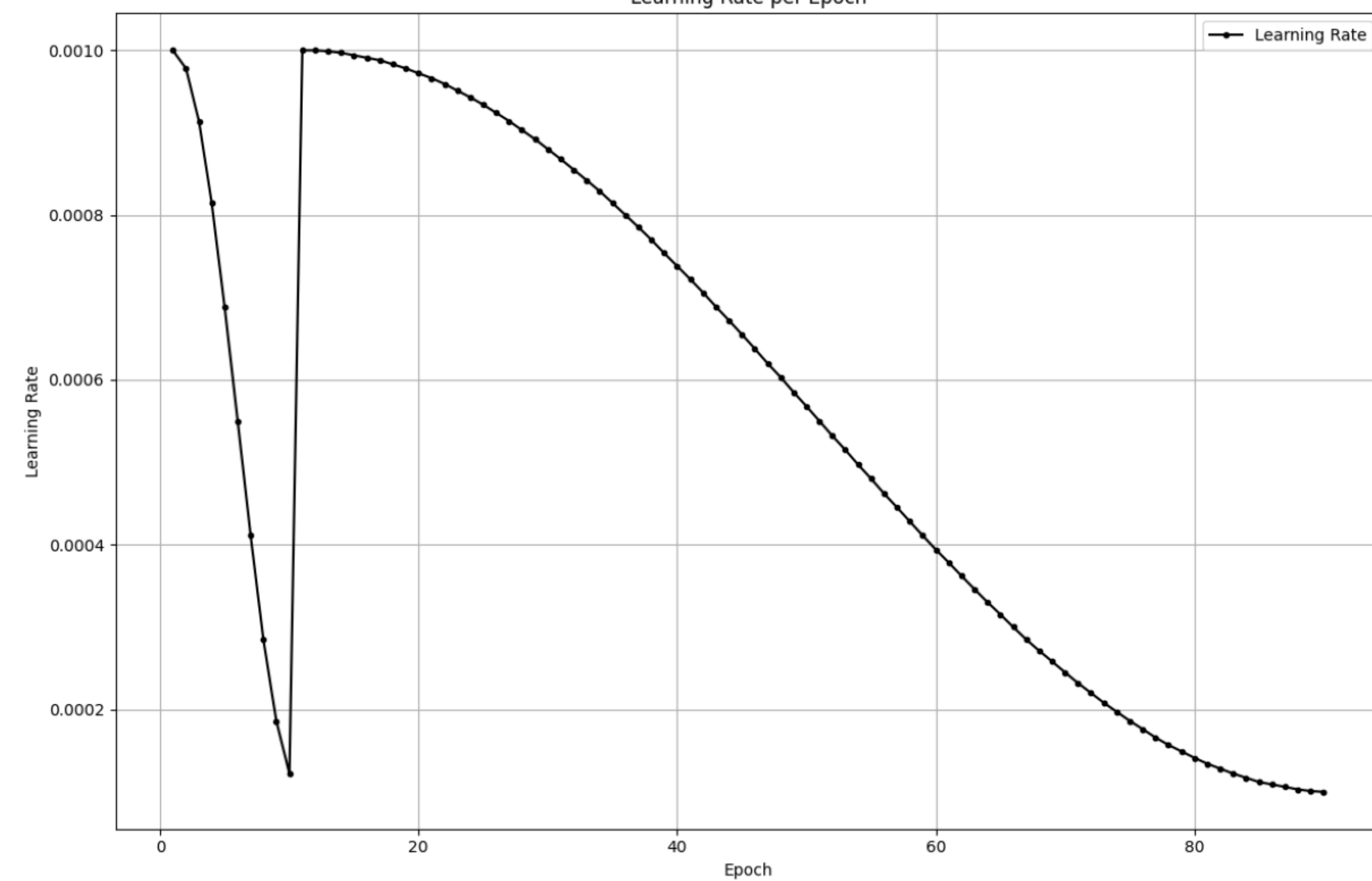
Learning Rate
