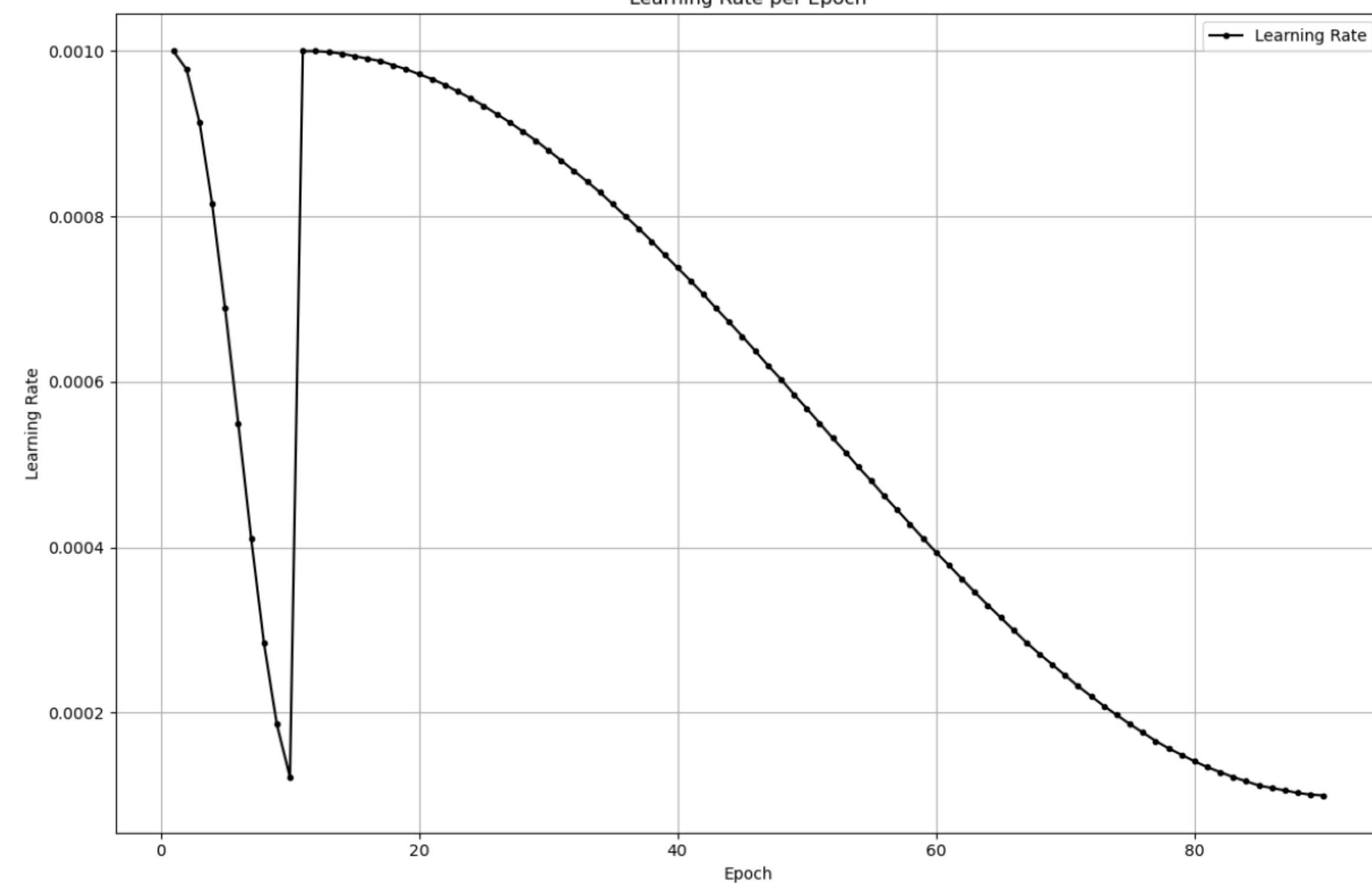
Learning Rate
