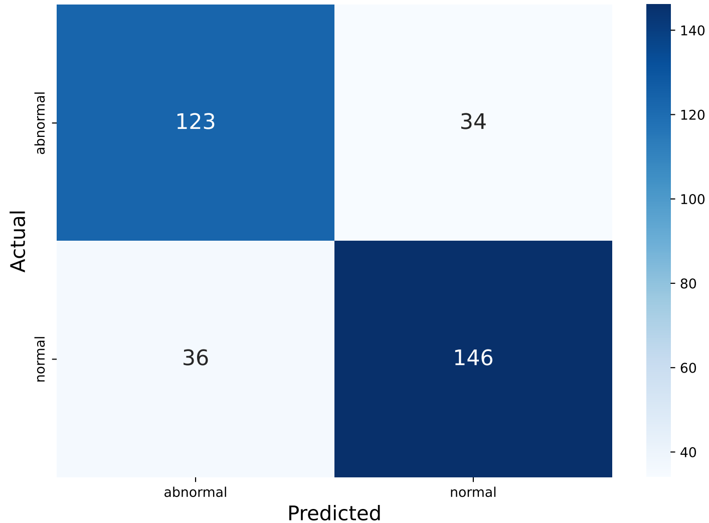
Confusion Matrix
