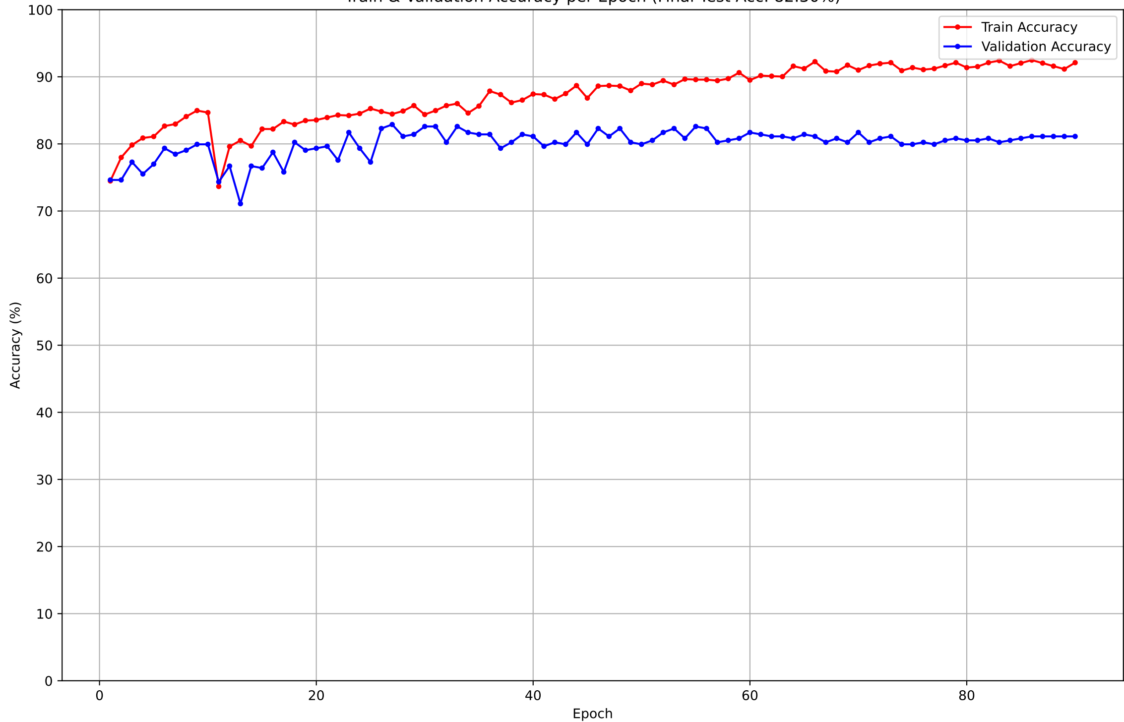
Train & Validation Accuracy per Epoch (Final Test Acc: 82.30%)
