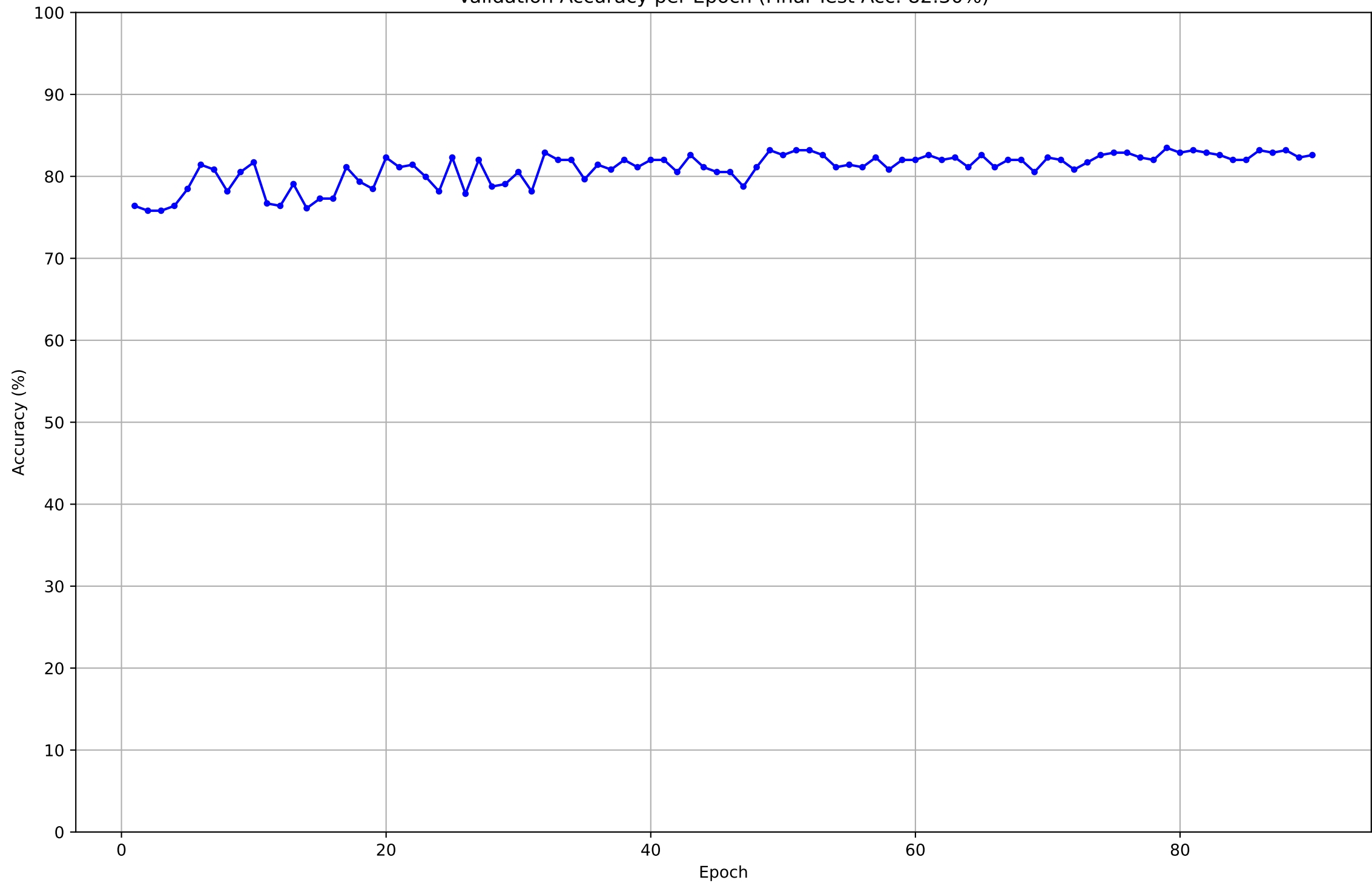
Validation Accuracy per Epoch (Final Test Acc: 82.30%)
