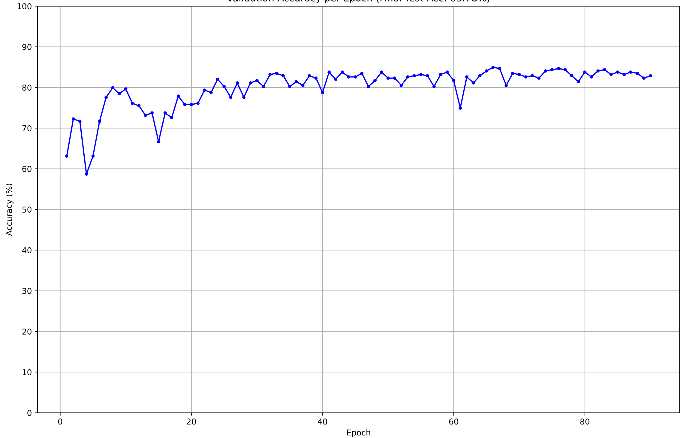
Validation Accuracy per Epoch (Final Test Acc: 83.78%)
