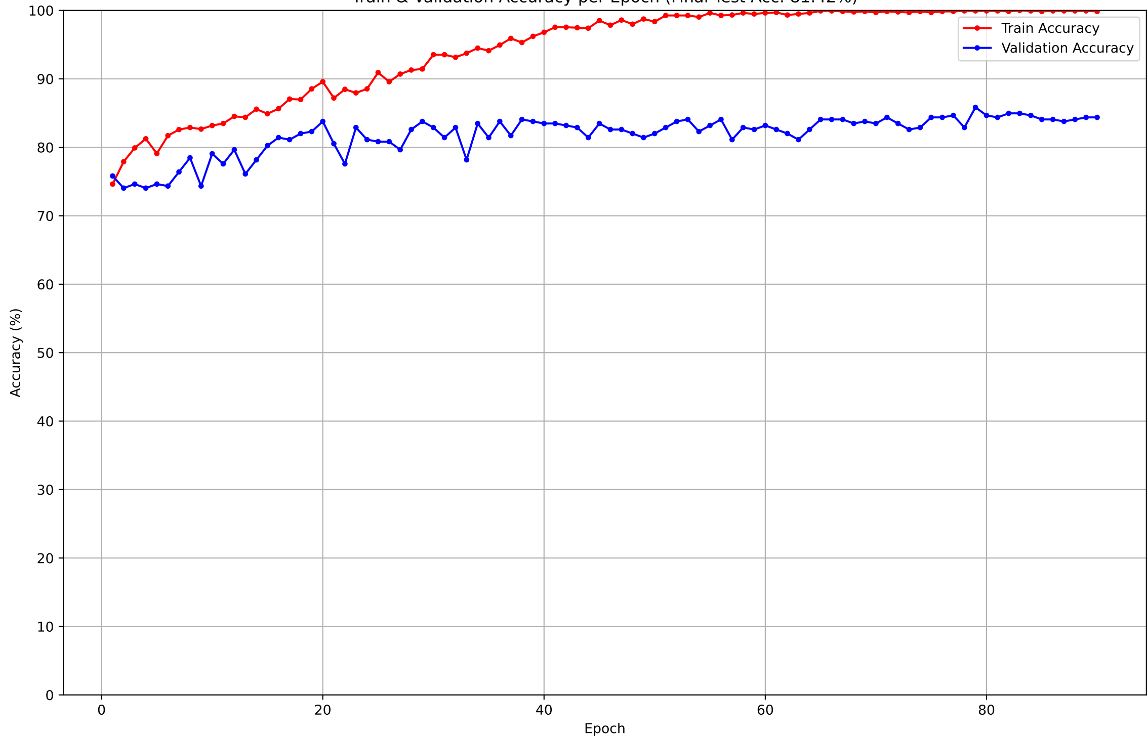
Train & Validation Accuracy per Epoch (Final Test Acc: 81.42%)
