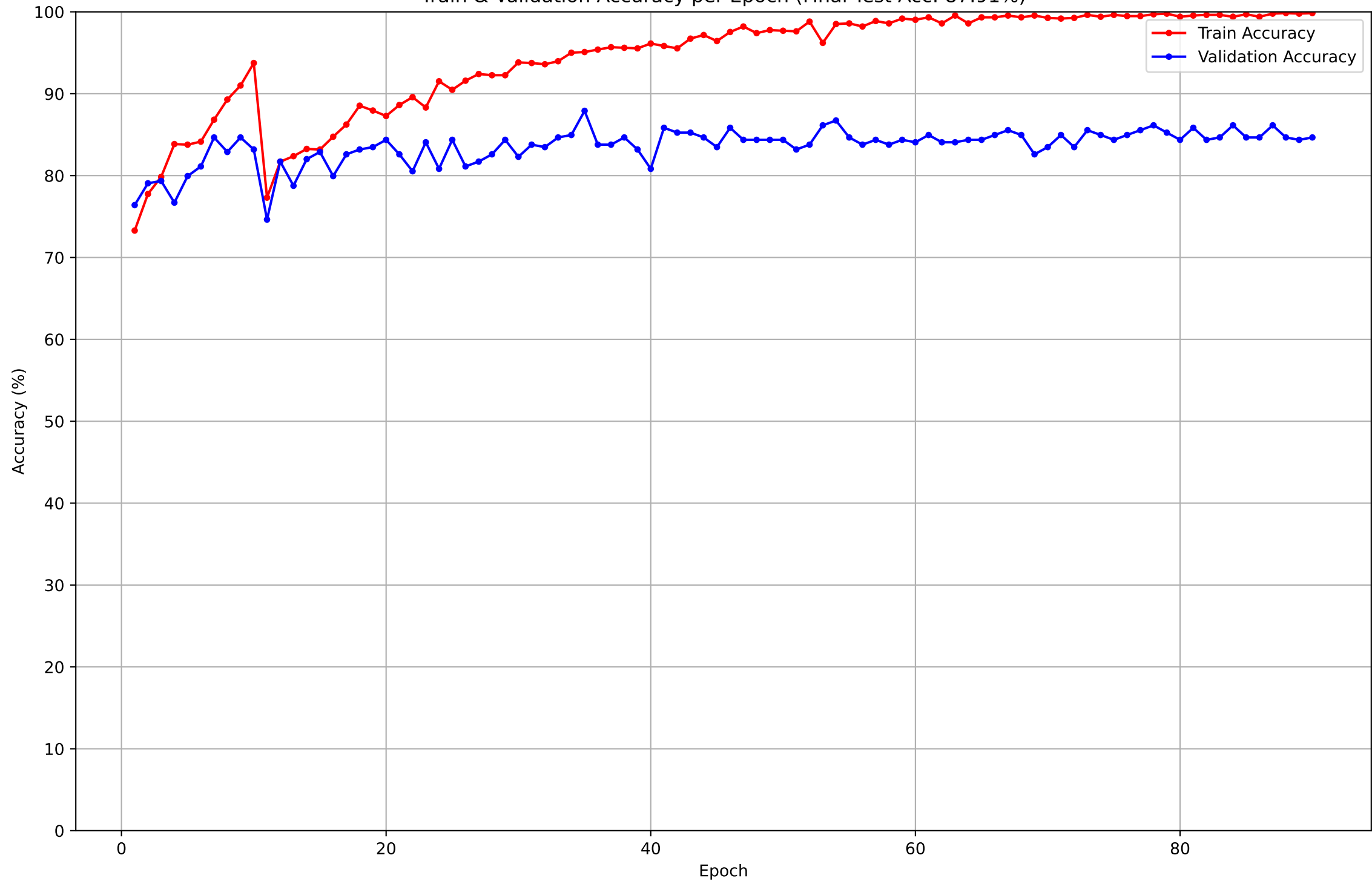
Train & Validation Accuracy per Epoch (Final Test Acc: 87.91%)
