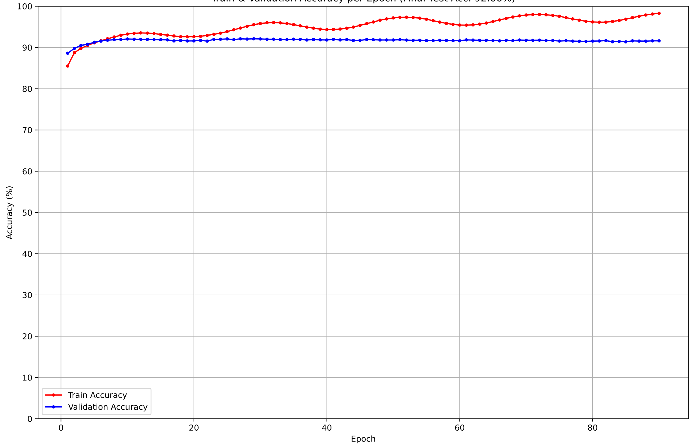
Train & Validation Accuracy per Epoch (Final Test Acc: 92.06%)
