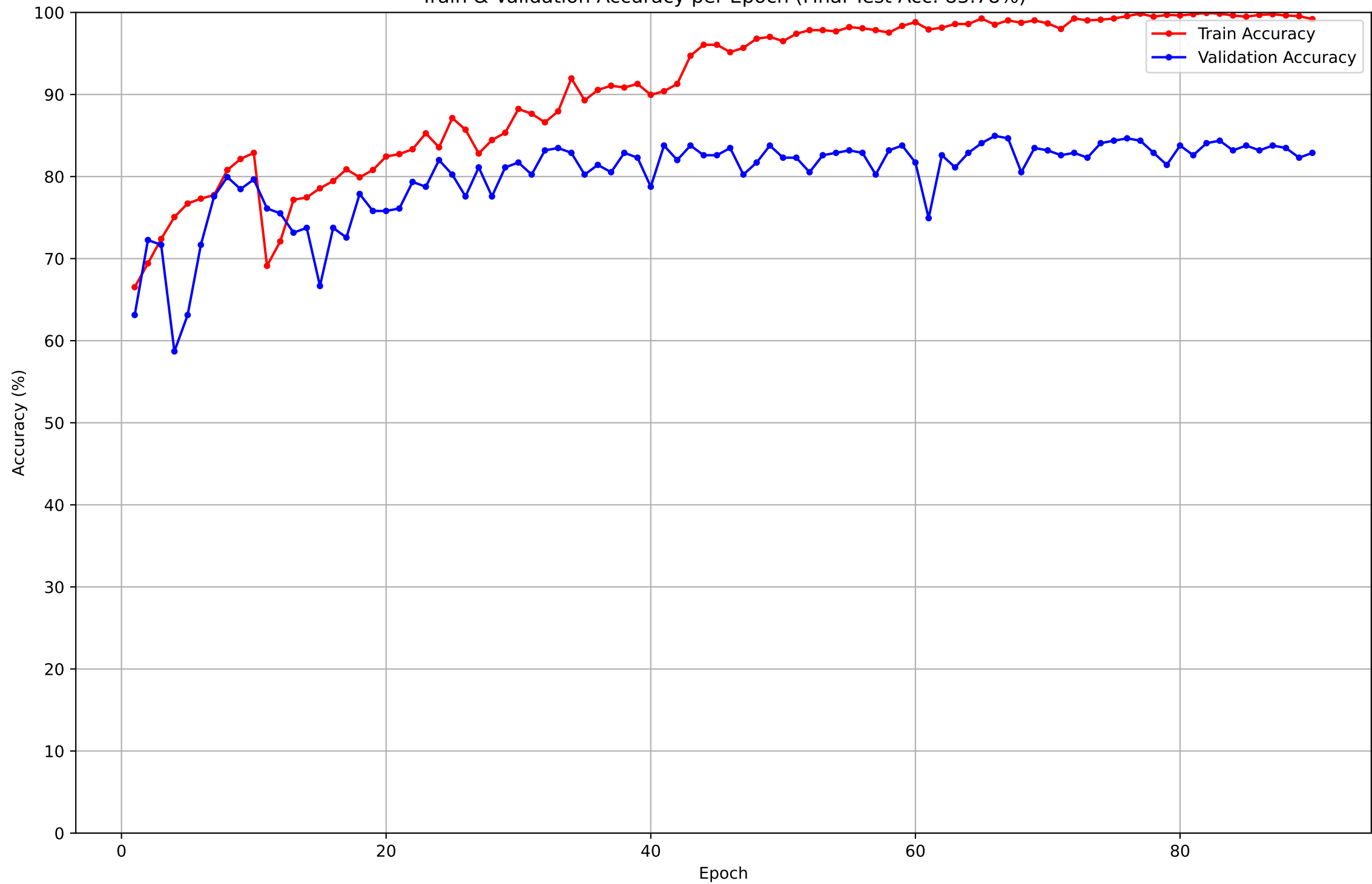
Train & Validation Accuracy per Epoch (Final Test Acc: 83.78%)
