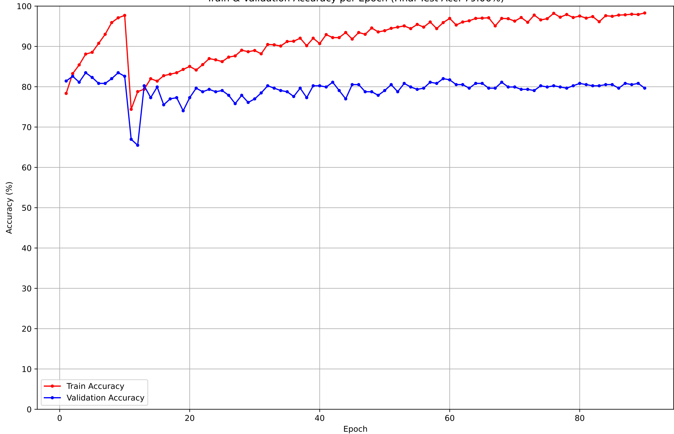
Train & Validation Accuracy per Epoch (Final Test Acc: 79.06%)
