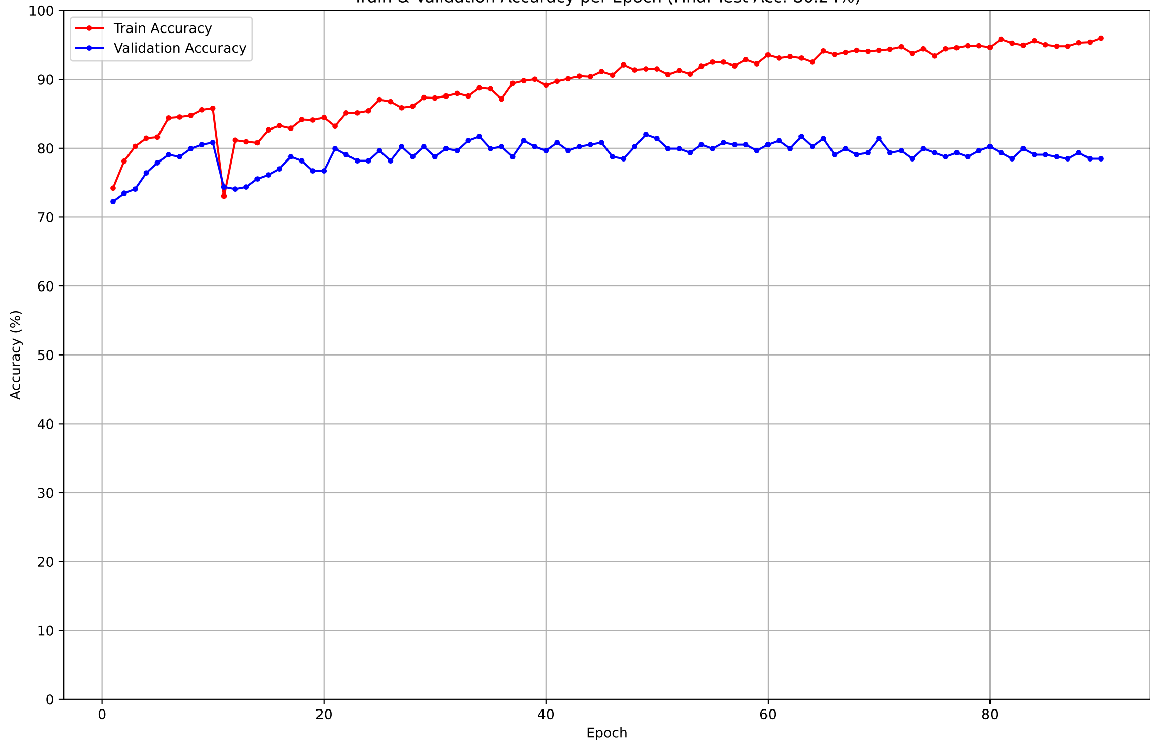
Train & Validation Accuracy per Epoch (Final Test Acc: 80.24%)
