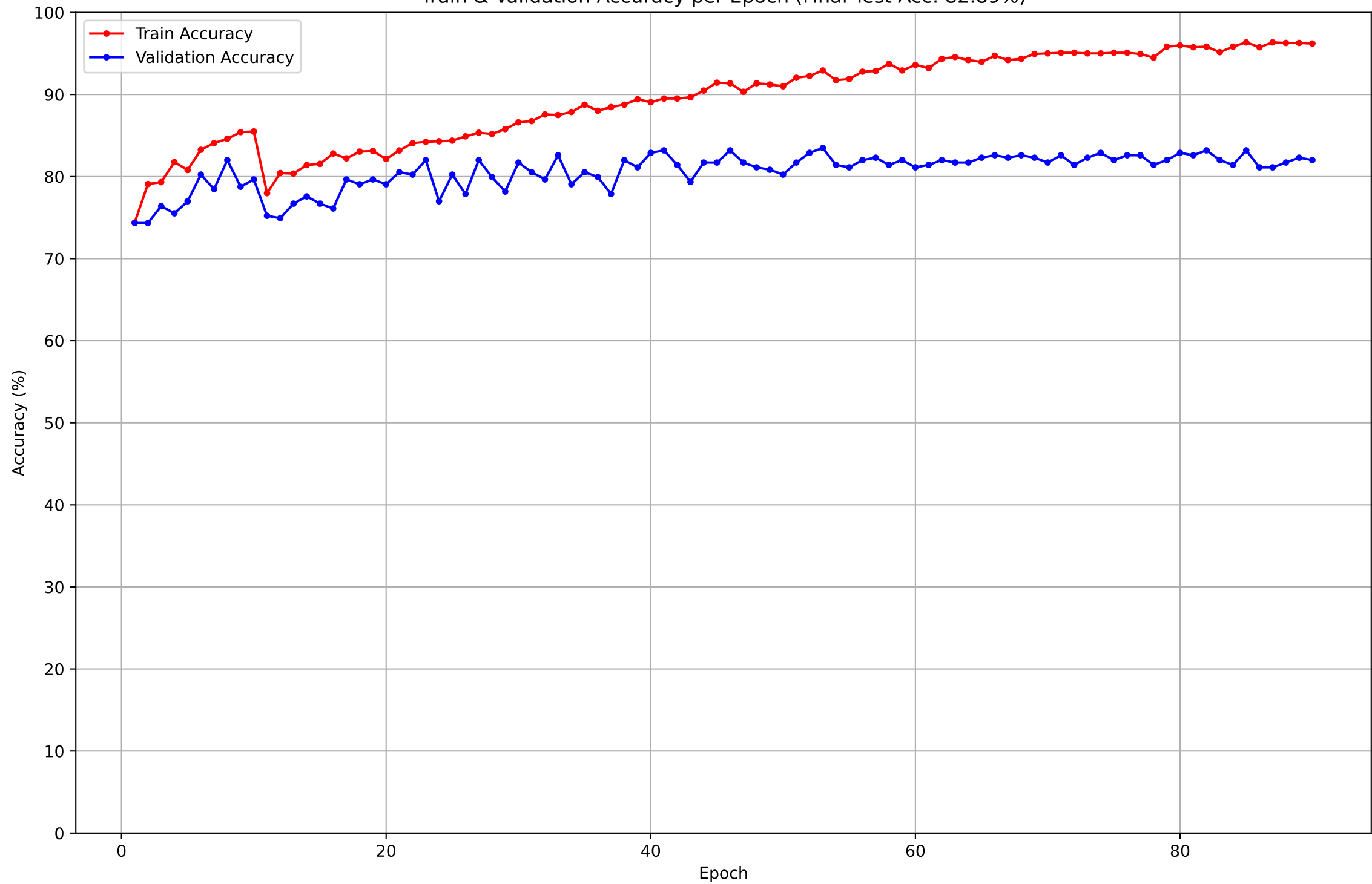
Train & Validation Accuracy per Epoch (Final Test Acc: 82.89%)
