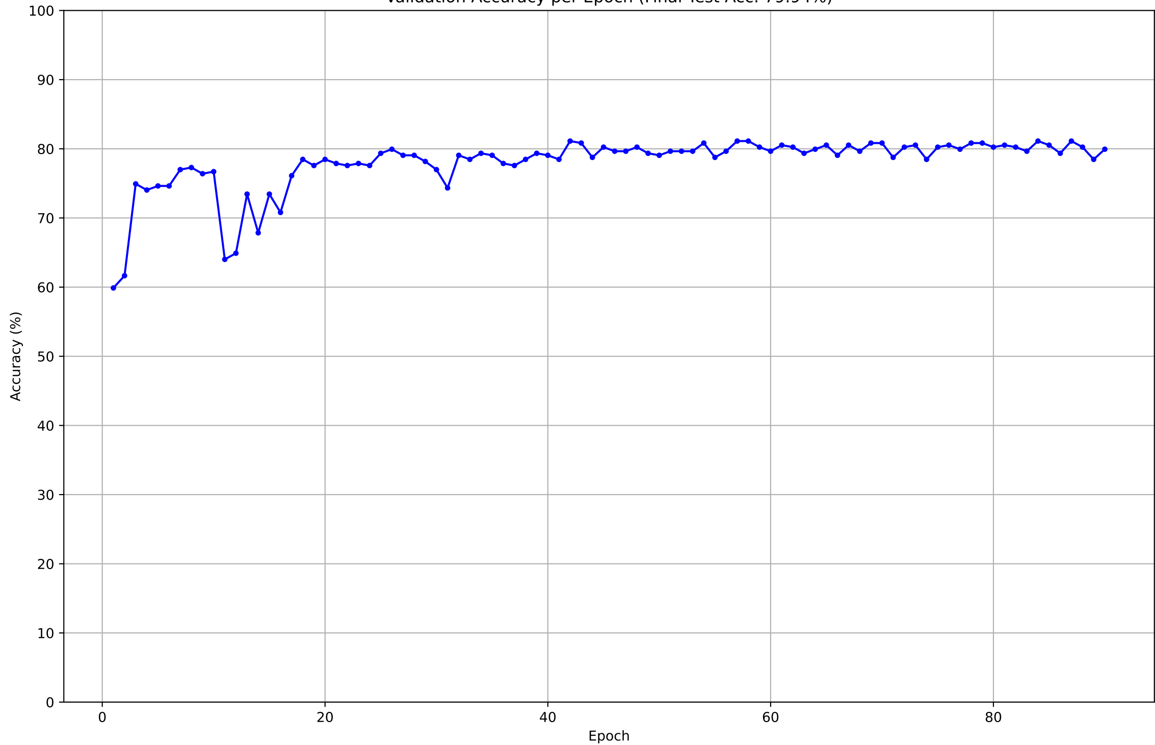
Validation Accuracy per Epoch (Final Test Acc: 79.94%)
