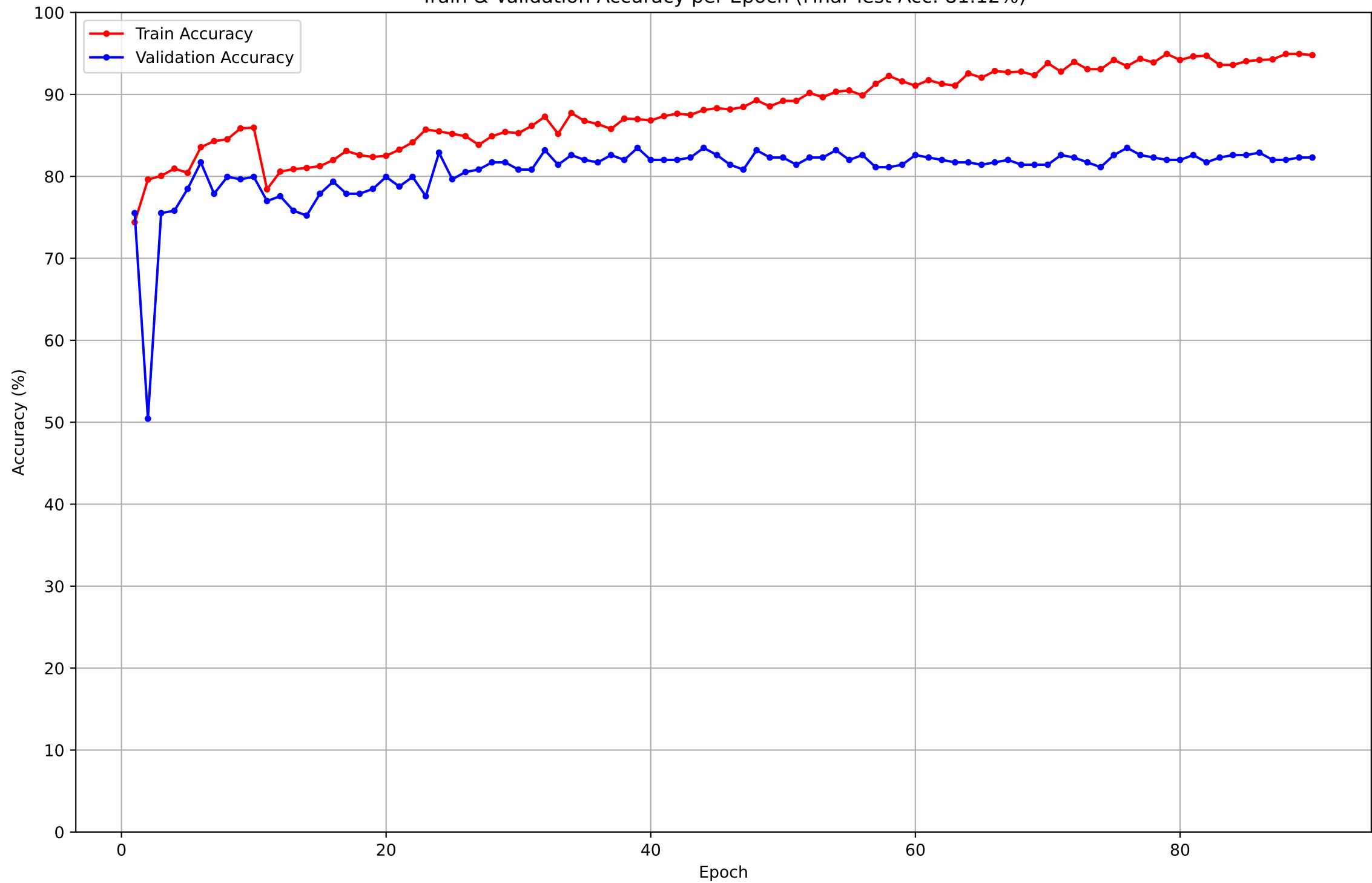
Train & Validation Accuracy per Epoch (Final Test Acc: 81.12%)
