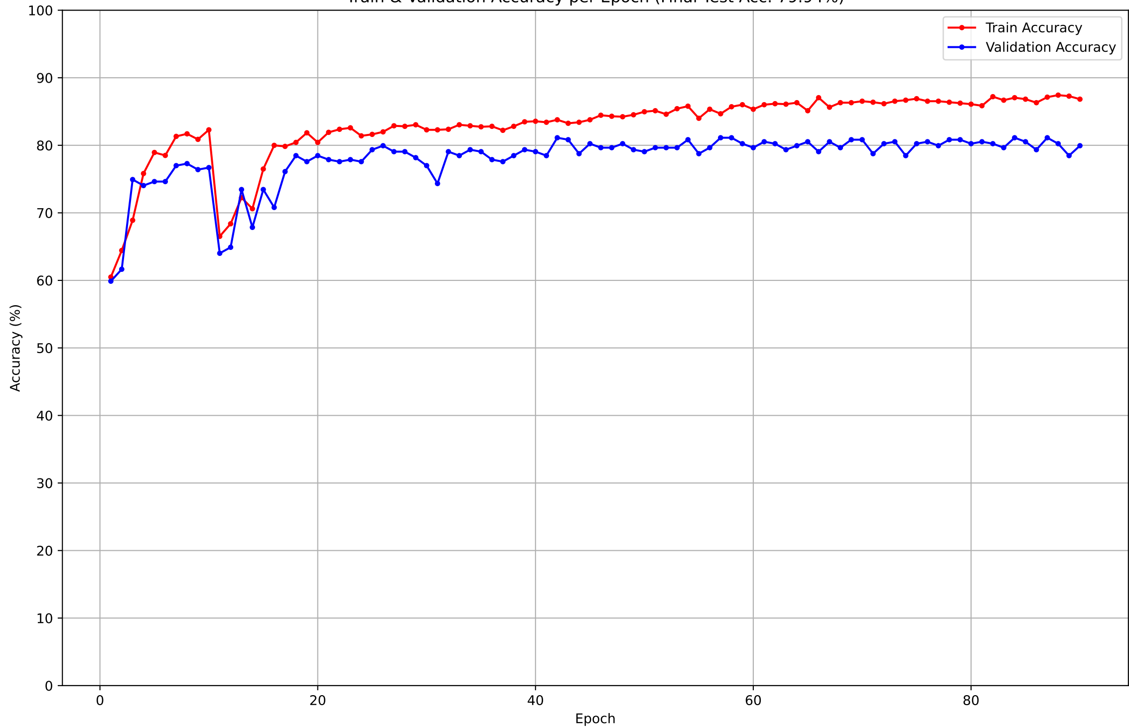
Train & Validation Accuracy per Epoch (Final Test Acc: 79.94%)
