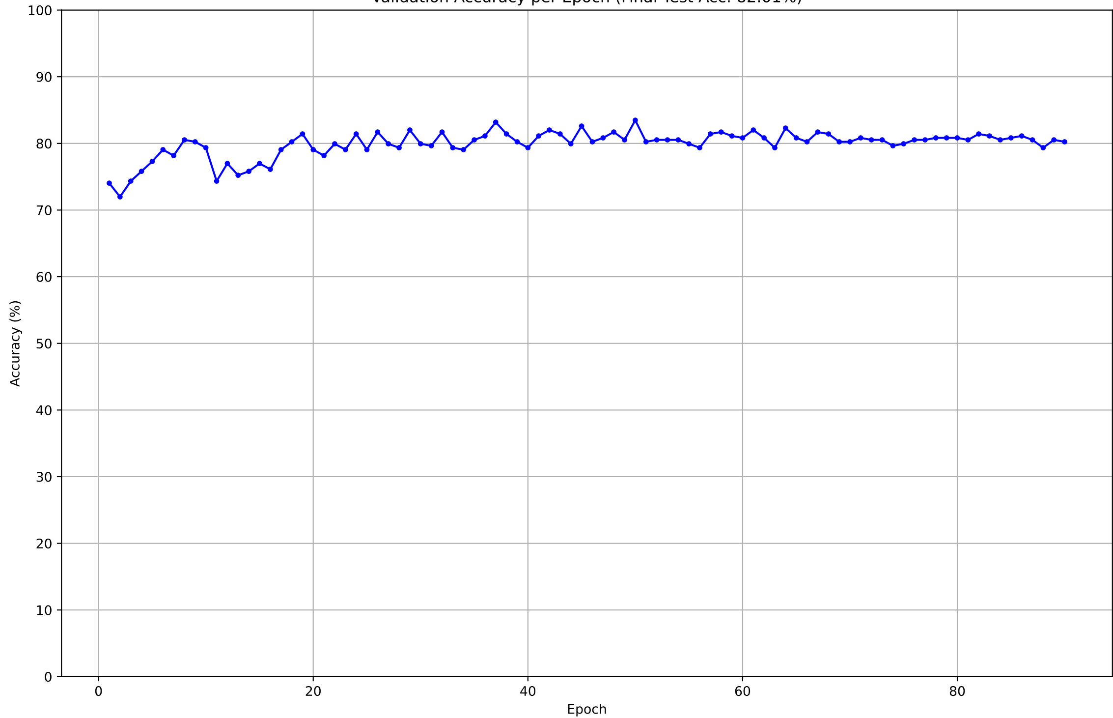
Validation Accuracy per Epoch (Final Test Acc: 82.01%)
