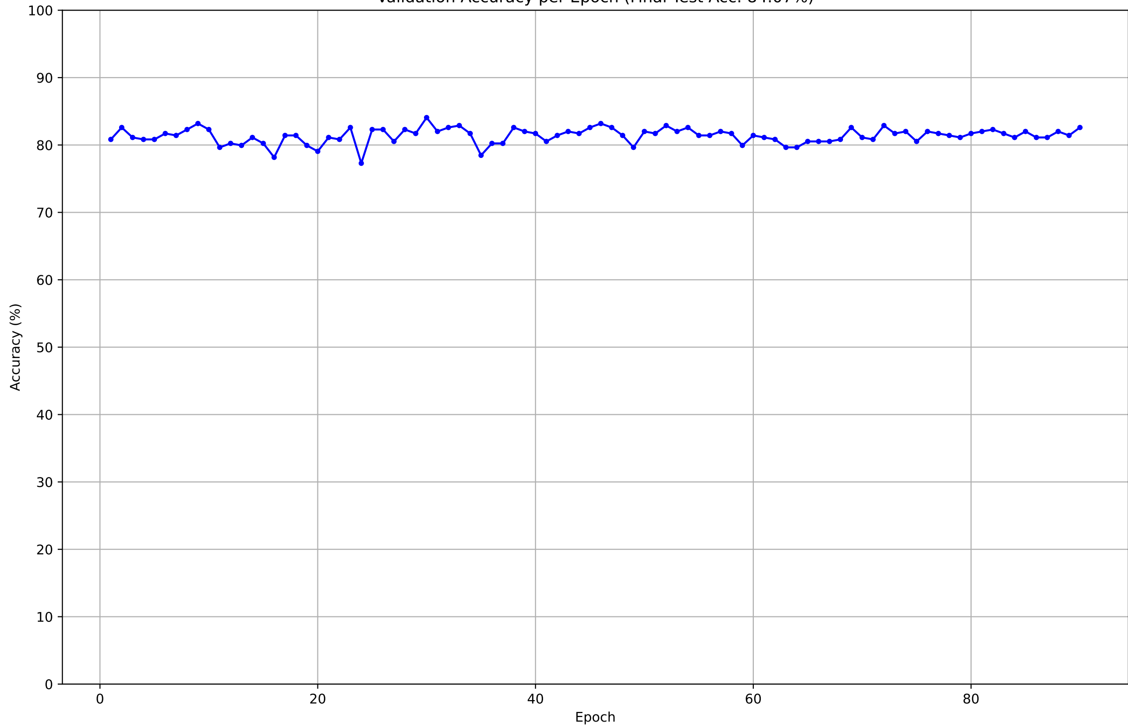
Validation Accuracy per Epoch (Final Test Acc: 84.07%)
