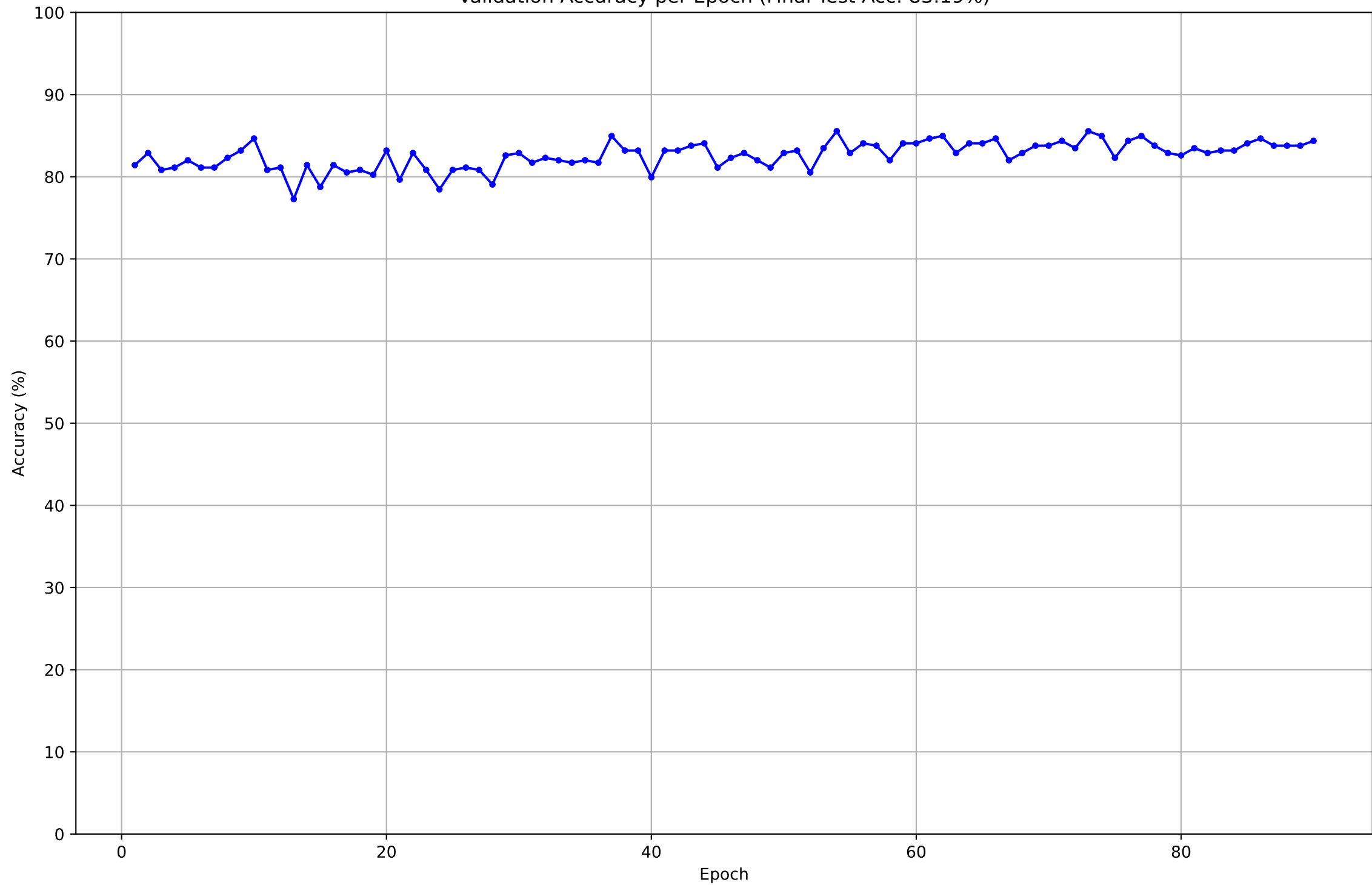
Validation Accuracy per Epoch (Final Test Acc: 83.19%)
