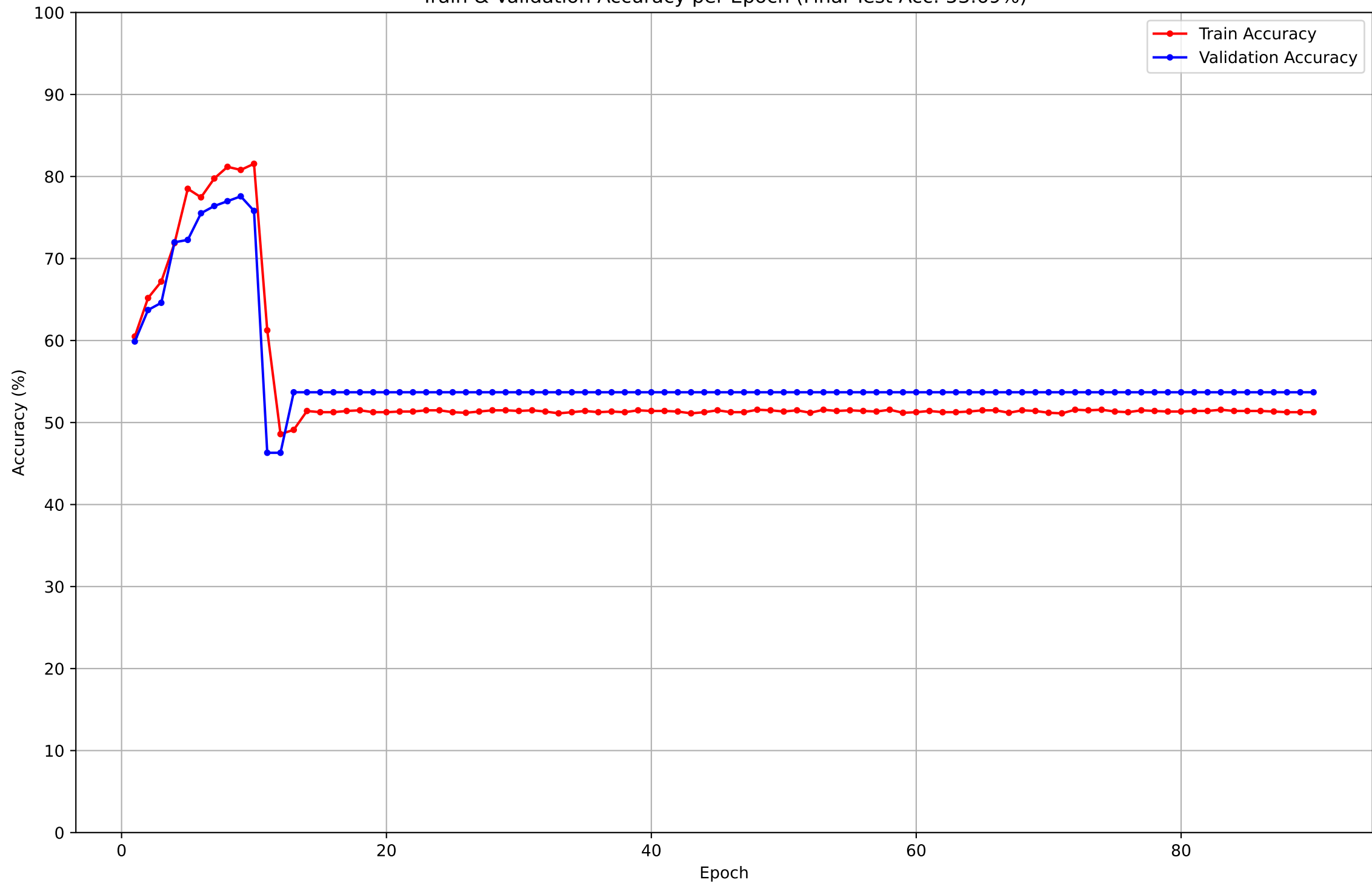
Train & Validation Accuracy per Epoch (Final Test Acc: 53.69%)
