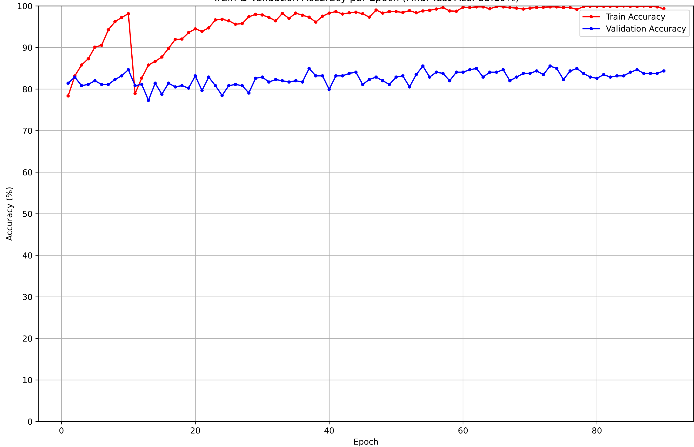
Train & Validation Accuracy per Epoch (Final Test Acc: 83.19%)
