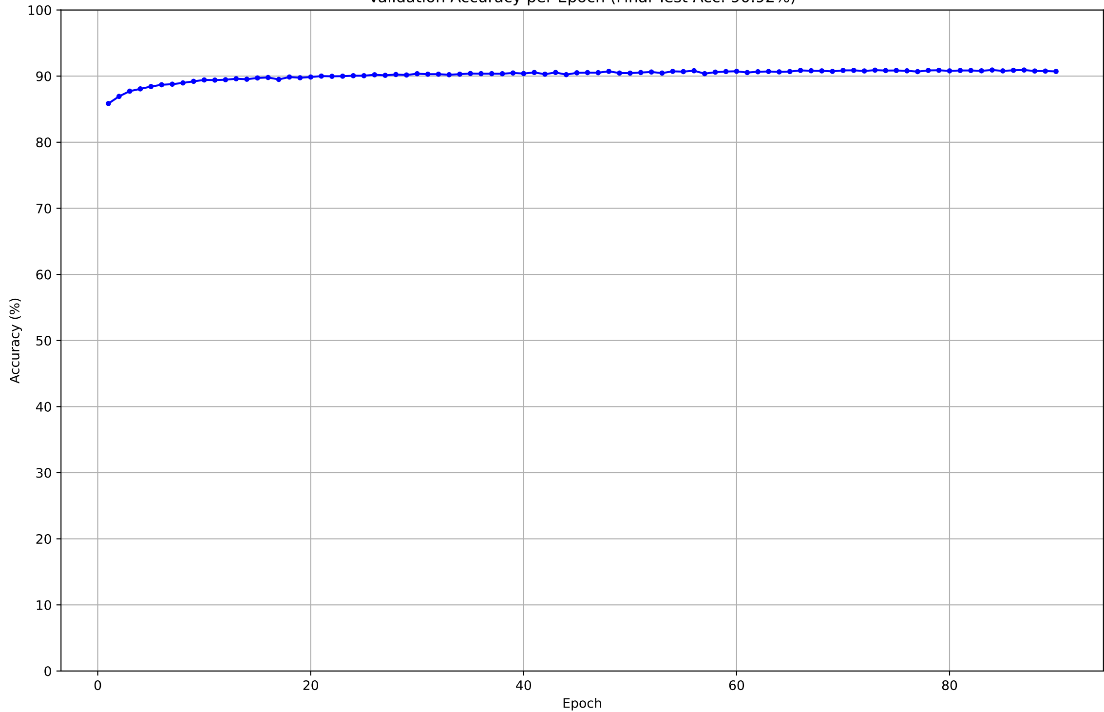
Validation Accuracy per Epoch (Final Test Acc: 90.92%)
