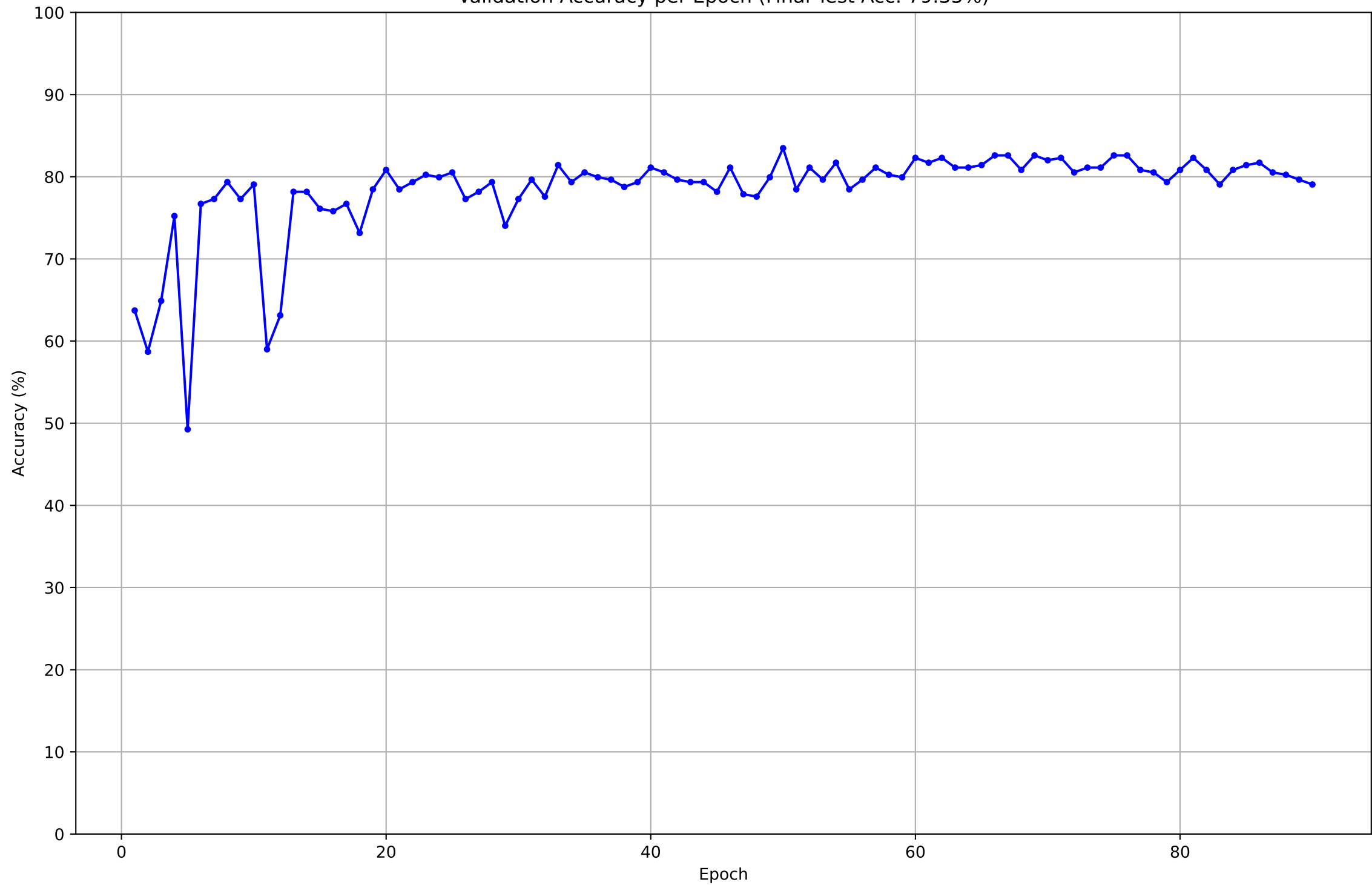
Validation Accuracy per Epoch (Final Test Acc: 79.35%)
