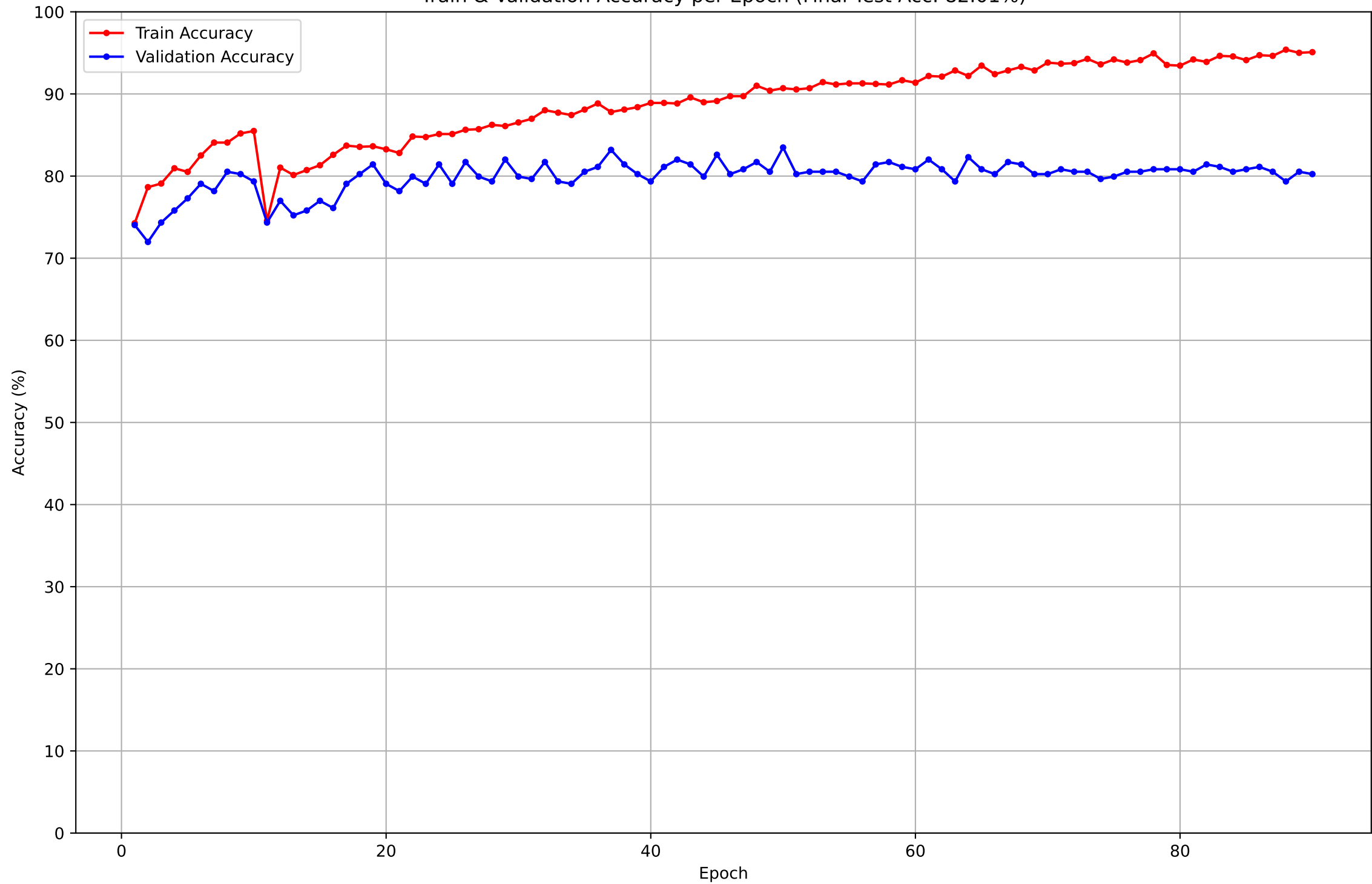
Train & Validation Accuracy per Epoch (Final Test Acc: 82.01%)
