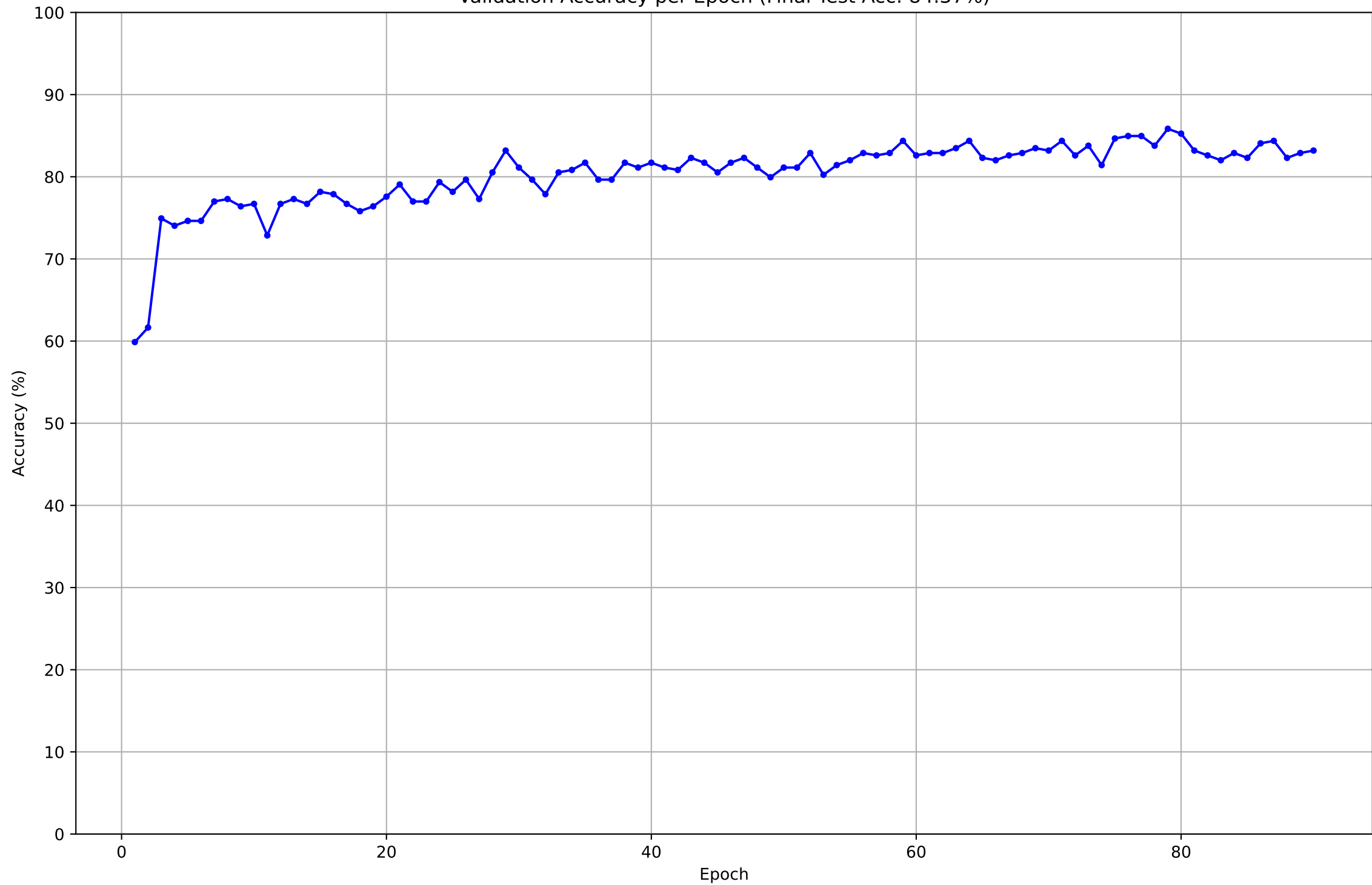
Validation Accuracy per Epoch (Final Test Acc: 84.37%)
