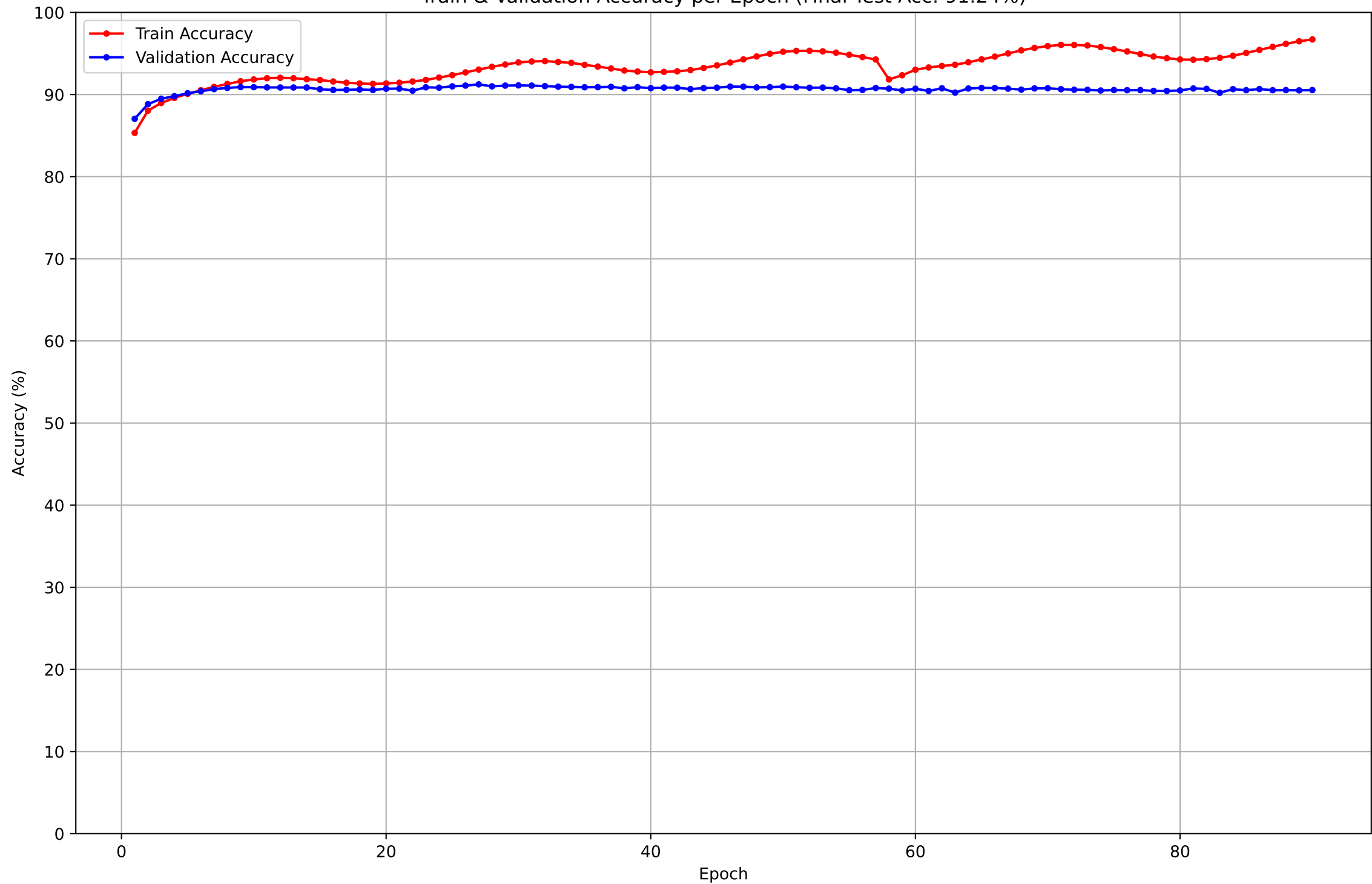
Train & Validation Accuracy per Epoch (Final Test Acc: 91.24%)
