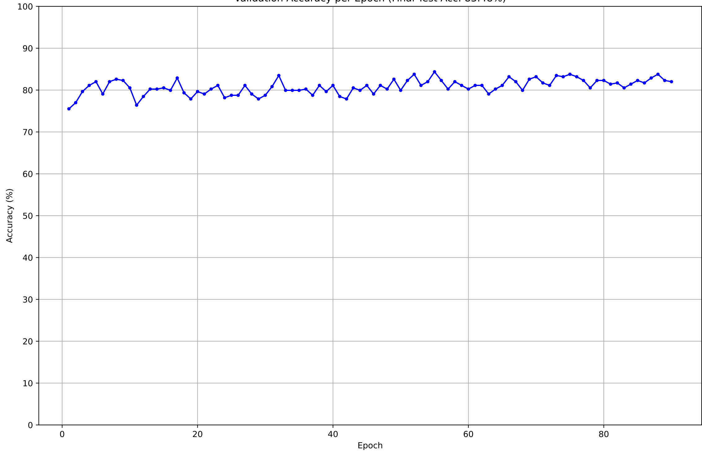
Validation Accuracy per Epoch (Final Test Acc: 83.48%)
