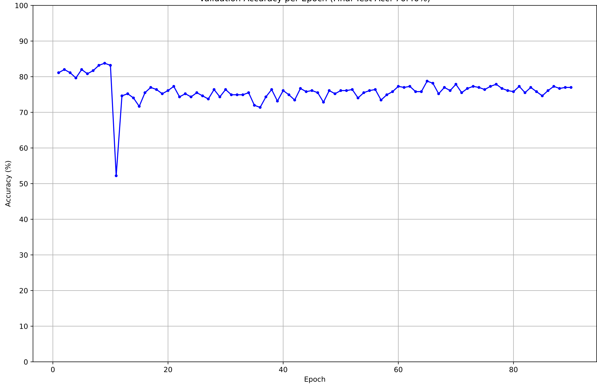
Validation Accuracy per Epoch (Final Test Acc: 76.40%)
