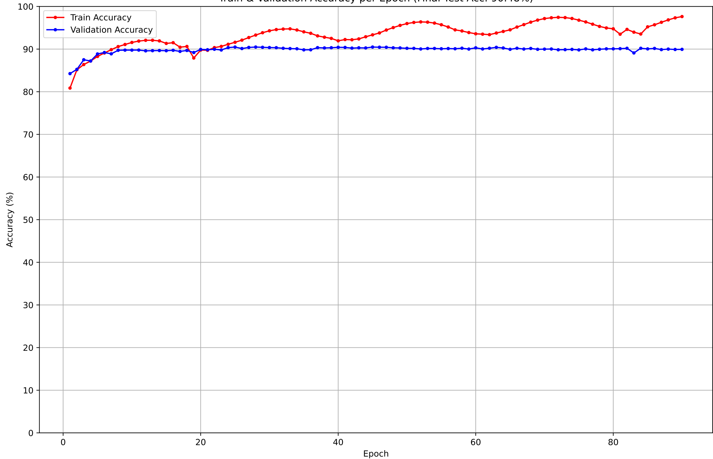
Train & Validation Accuracy per Epoch (Final Test Acc: 90.48%)
