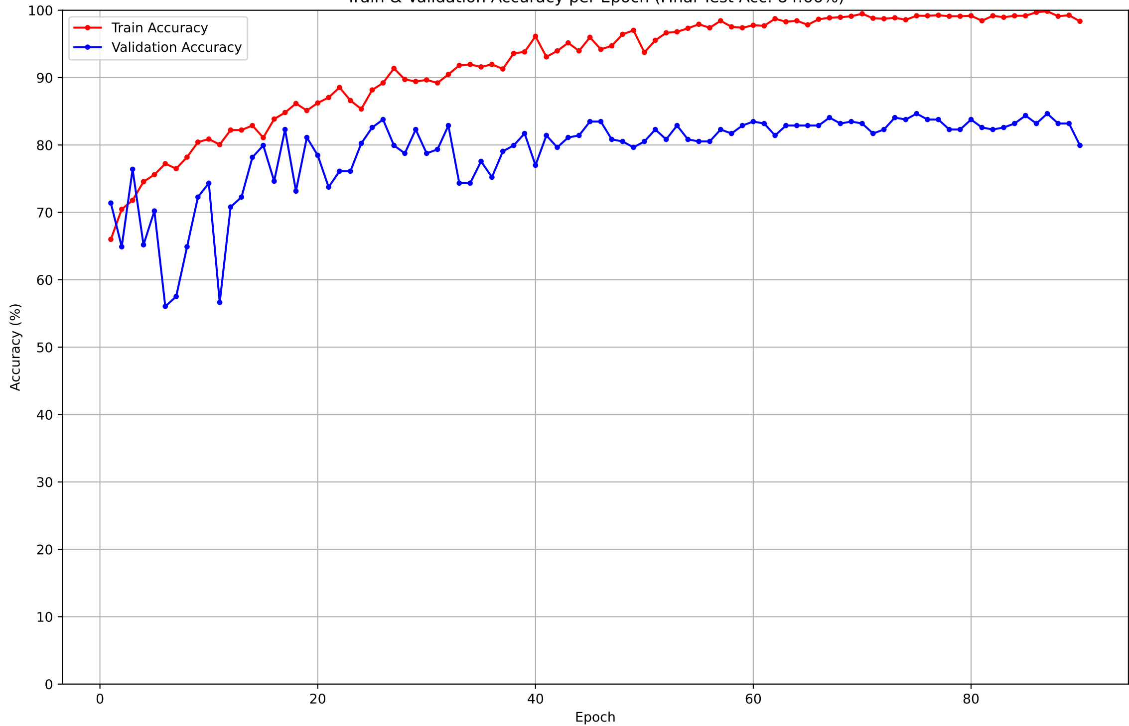
Train & Validation Accuracy per Epoch (Final Test Acc: 84.66%)
