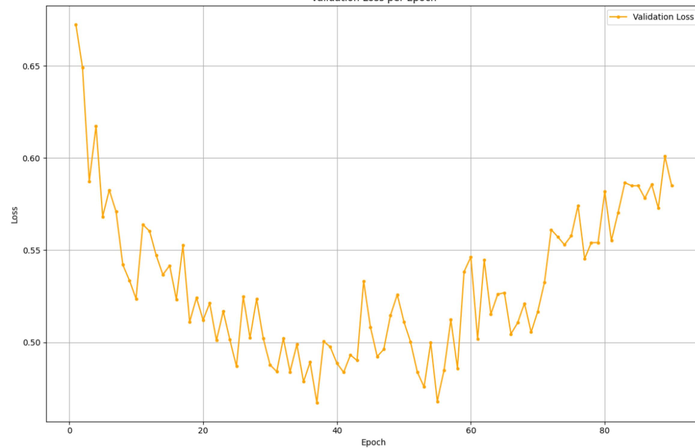
Validation Loss
