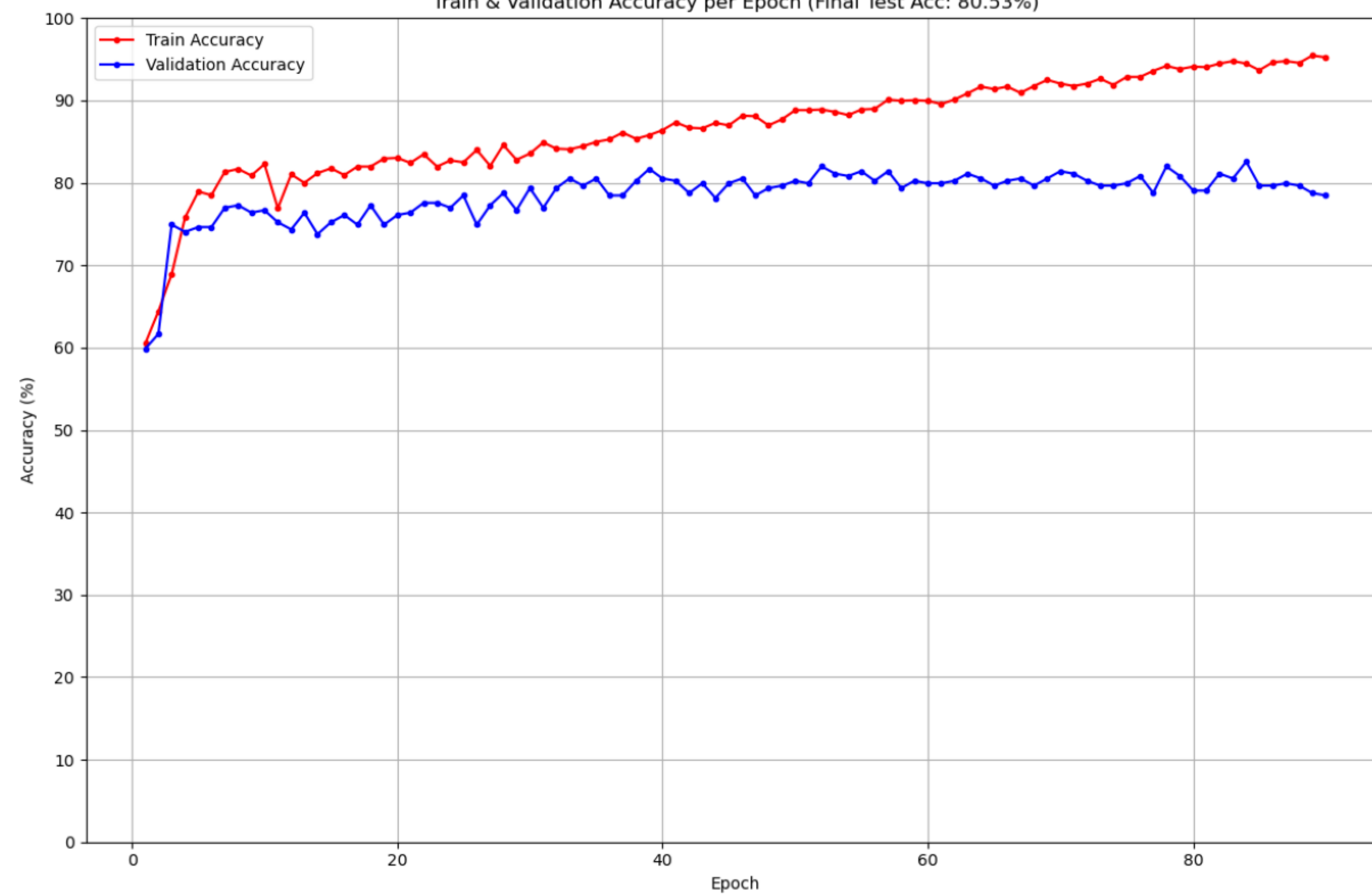
Train/Validation Accuracy
