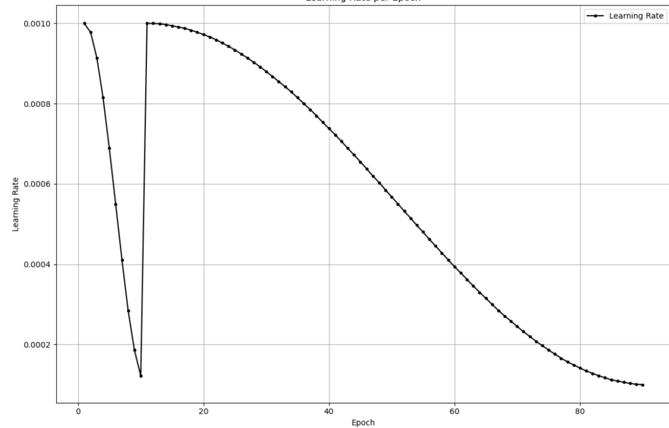
Learning Rate
