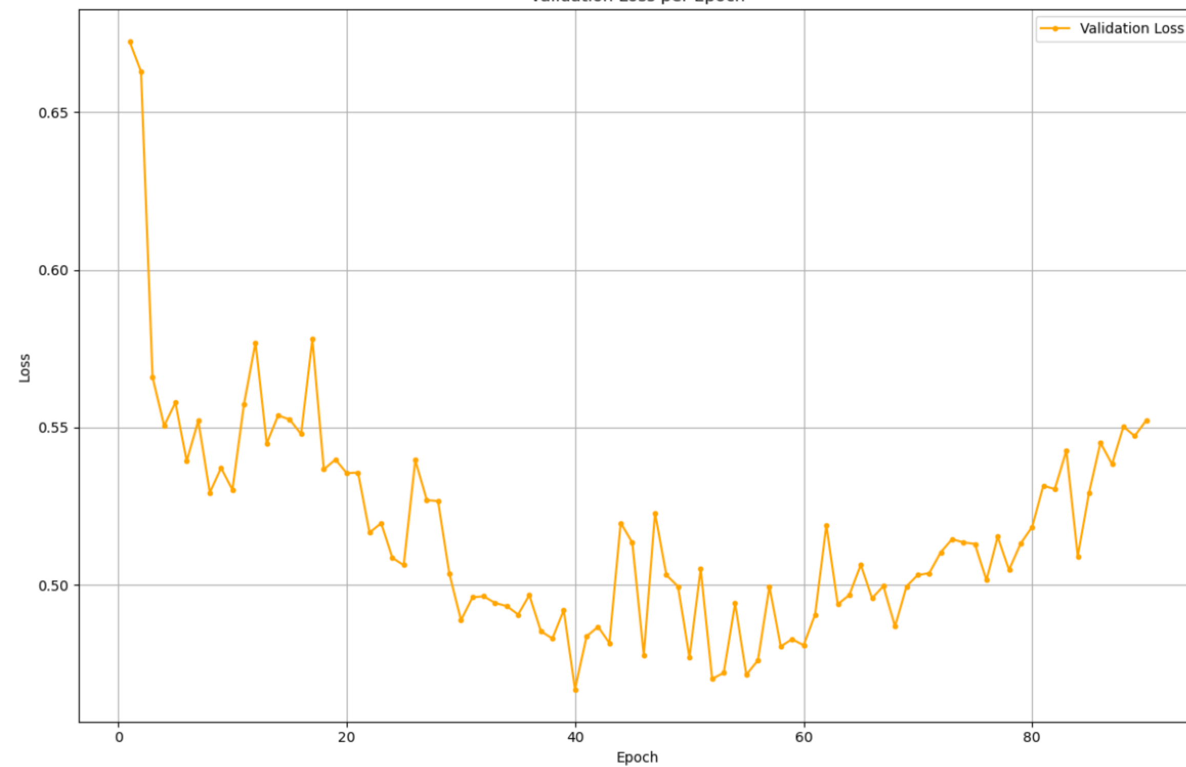
Validation Loss
