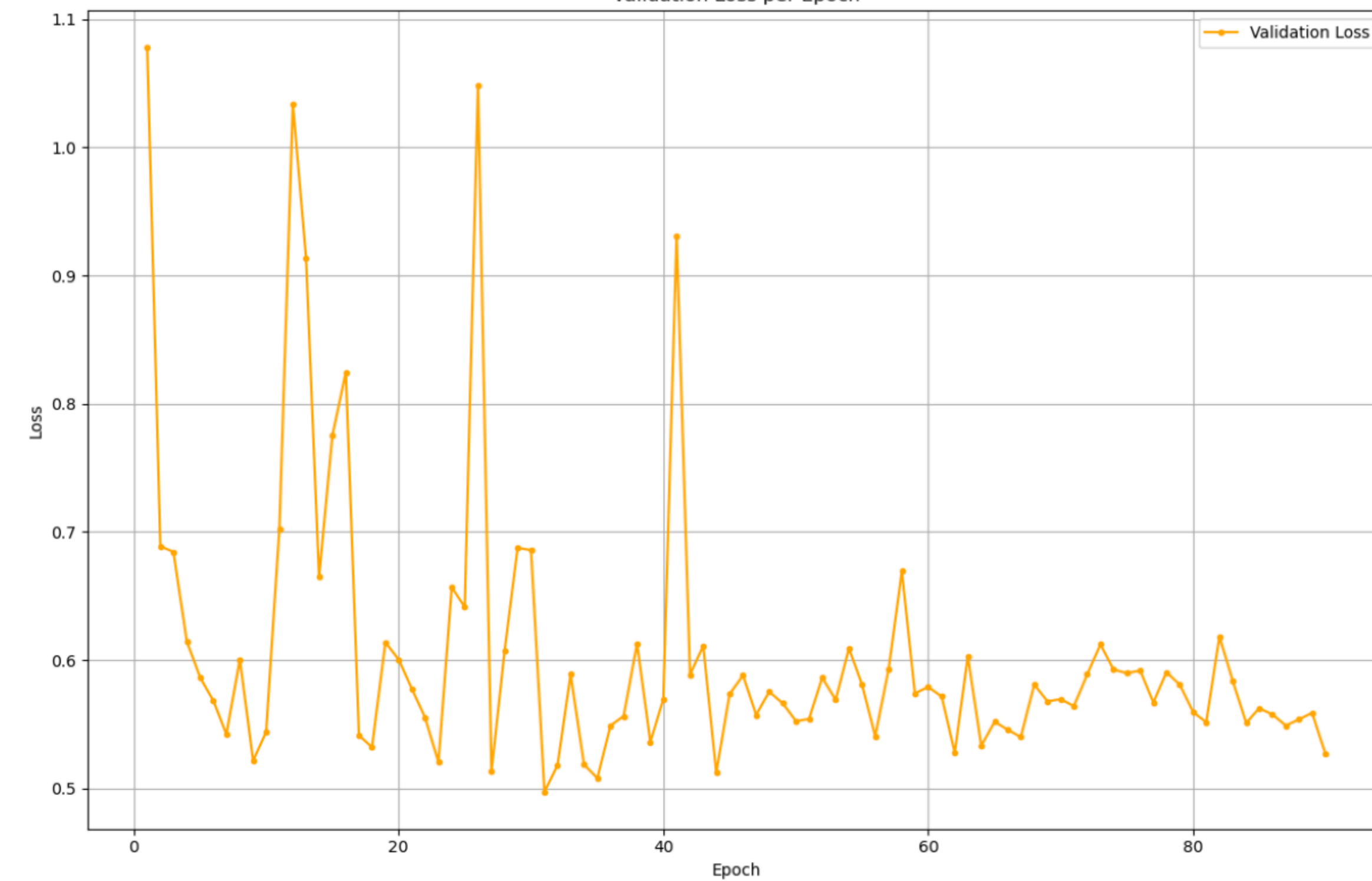
Validation Loss
