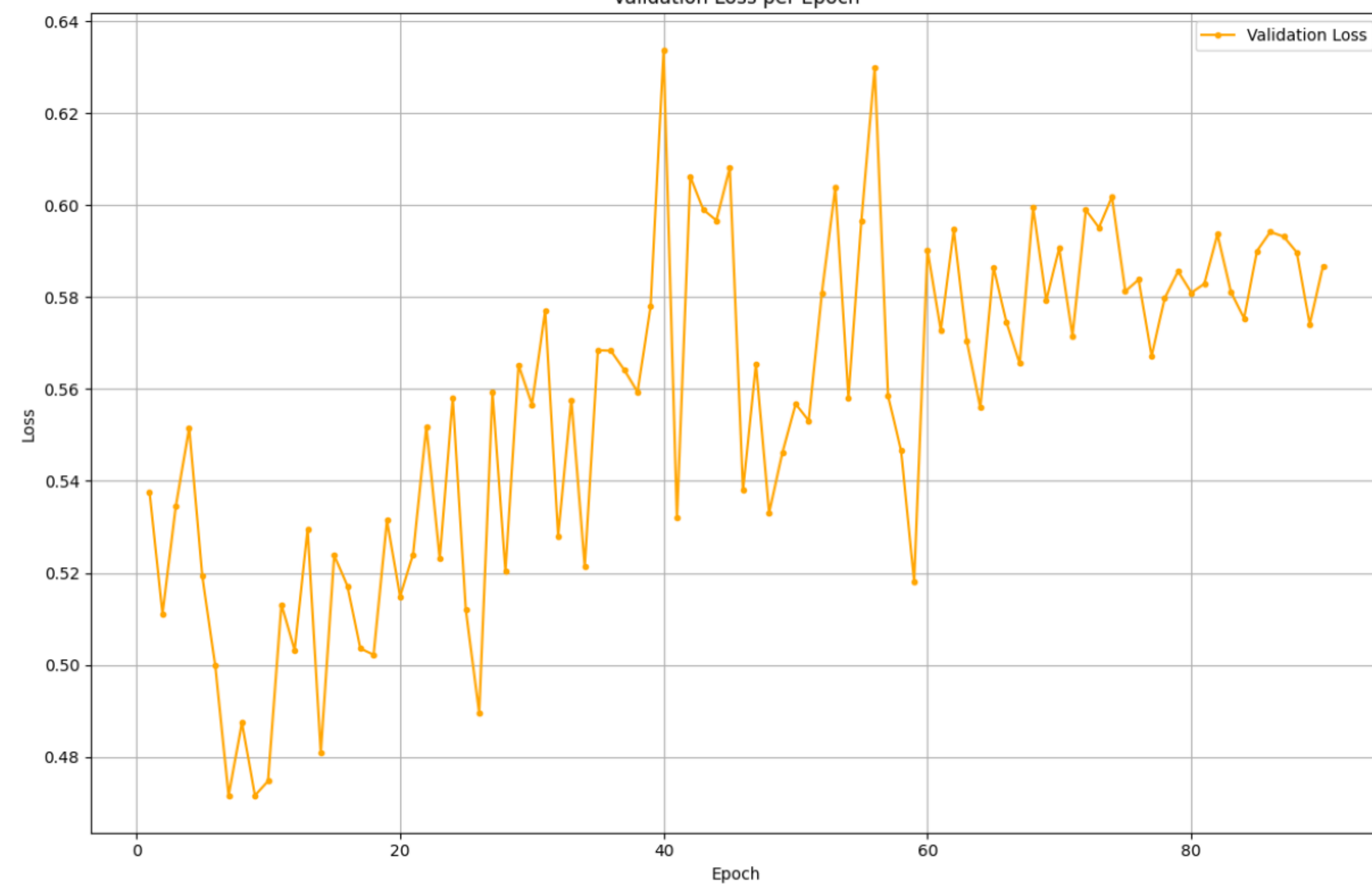
Validation Loss
