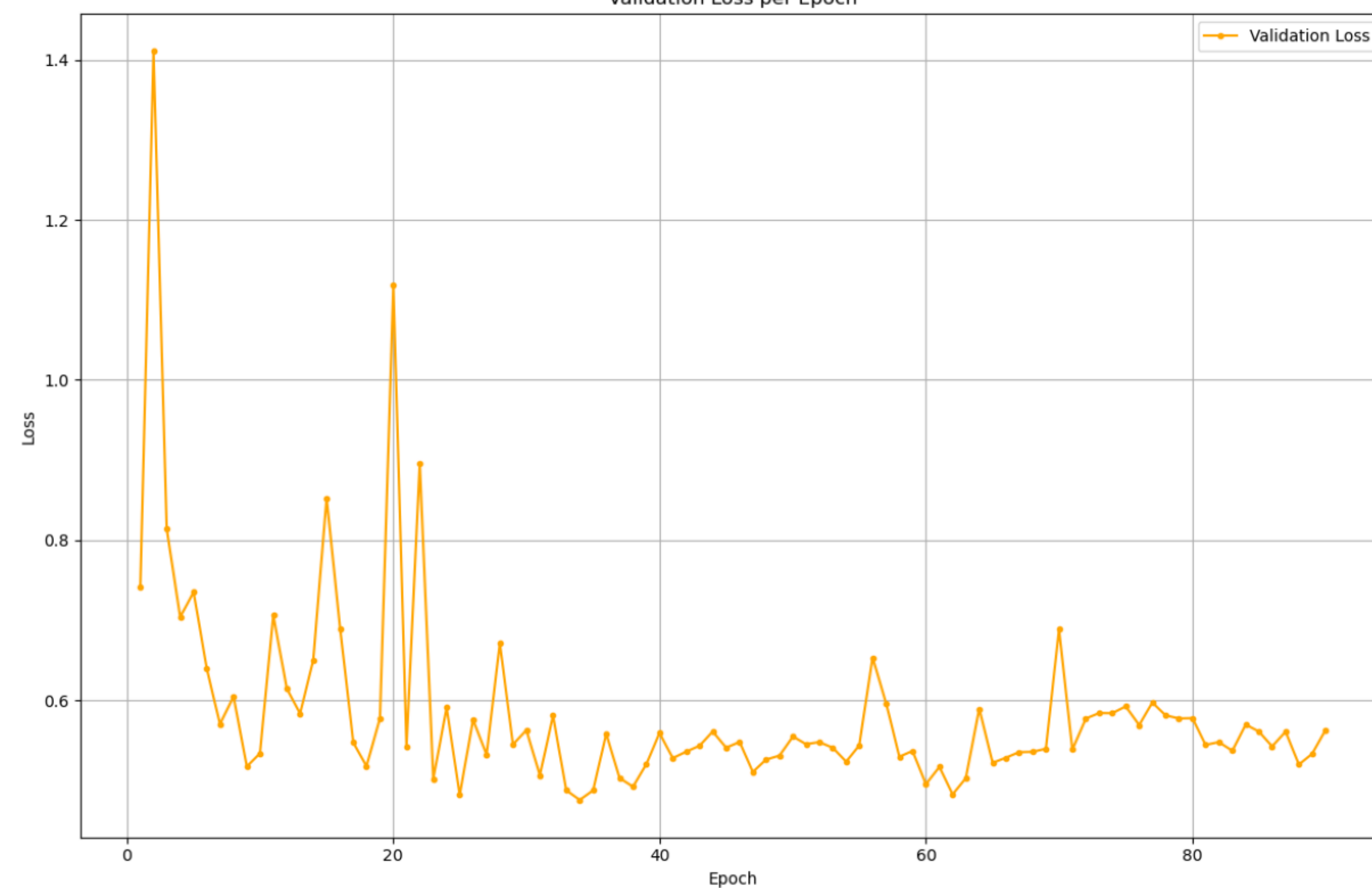
Validation Loss
