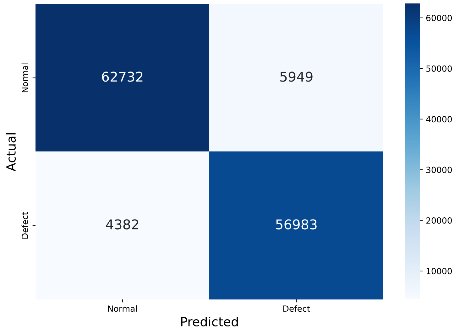
Confusion Matrix
