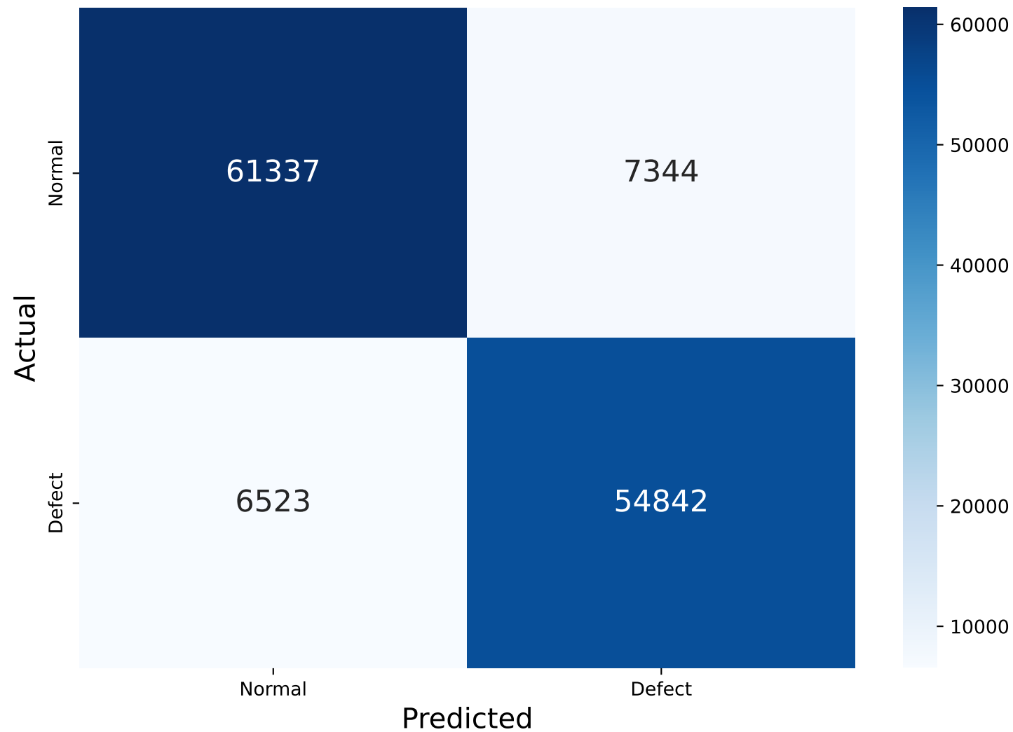
Confusion Matrix
