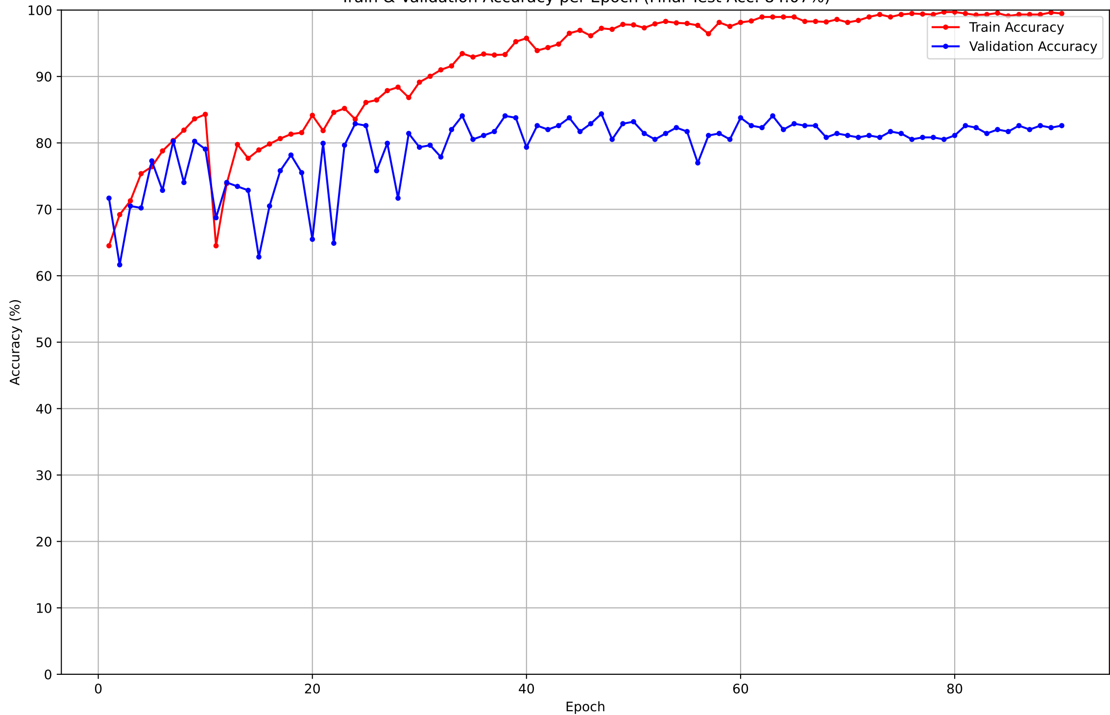
Train & Validation Accuracy per Epoch (Final Test Acc: 84.07%)
