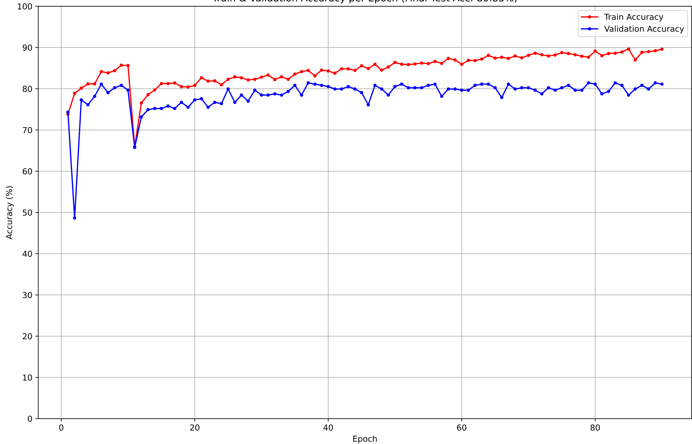
Train & Validation Accuracy per Epoch (Final Test Acc: 80.83%)
