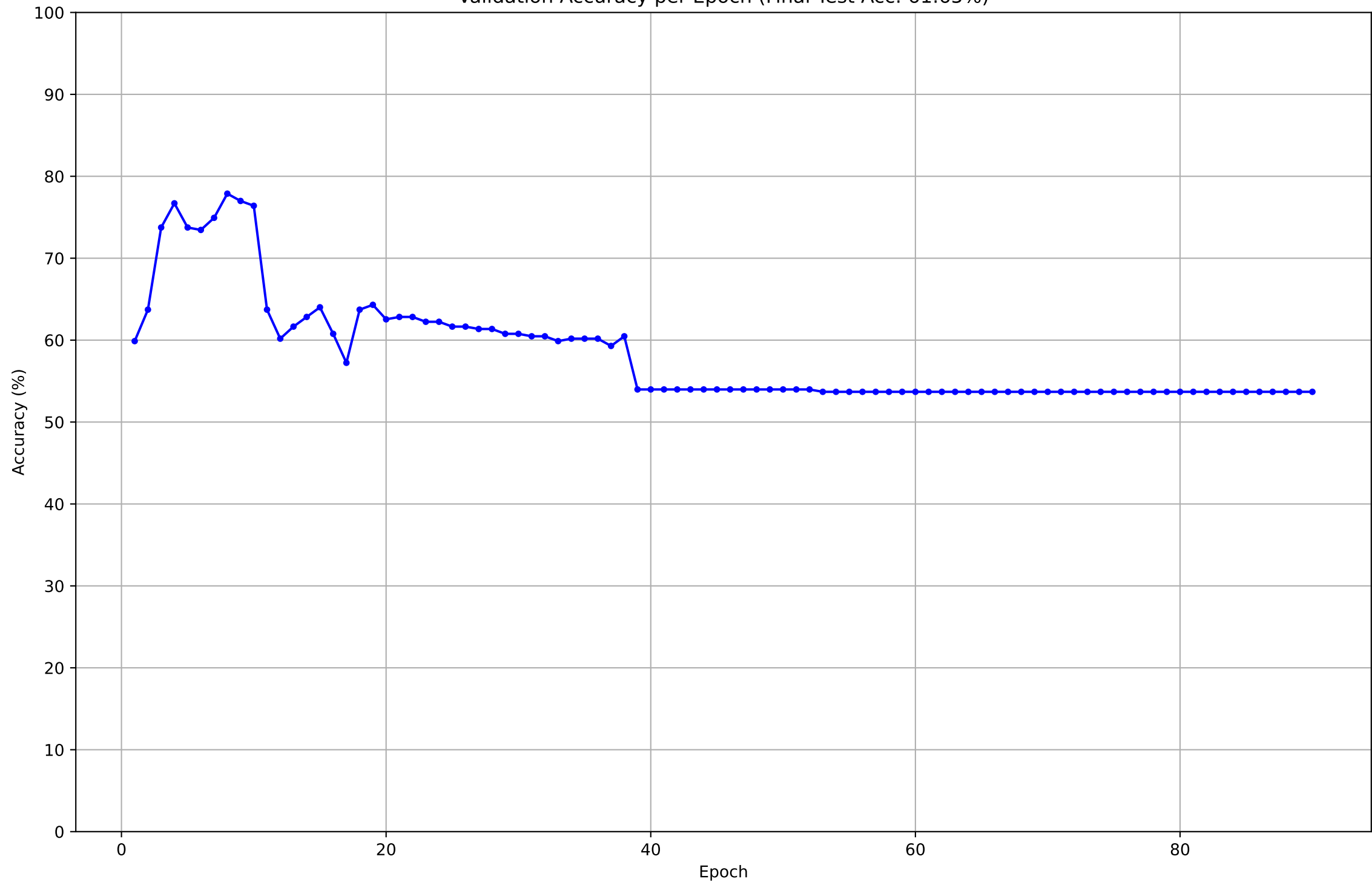
Validation Accuracy per Epoch (Final Test Acc: 61.65%)
