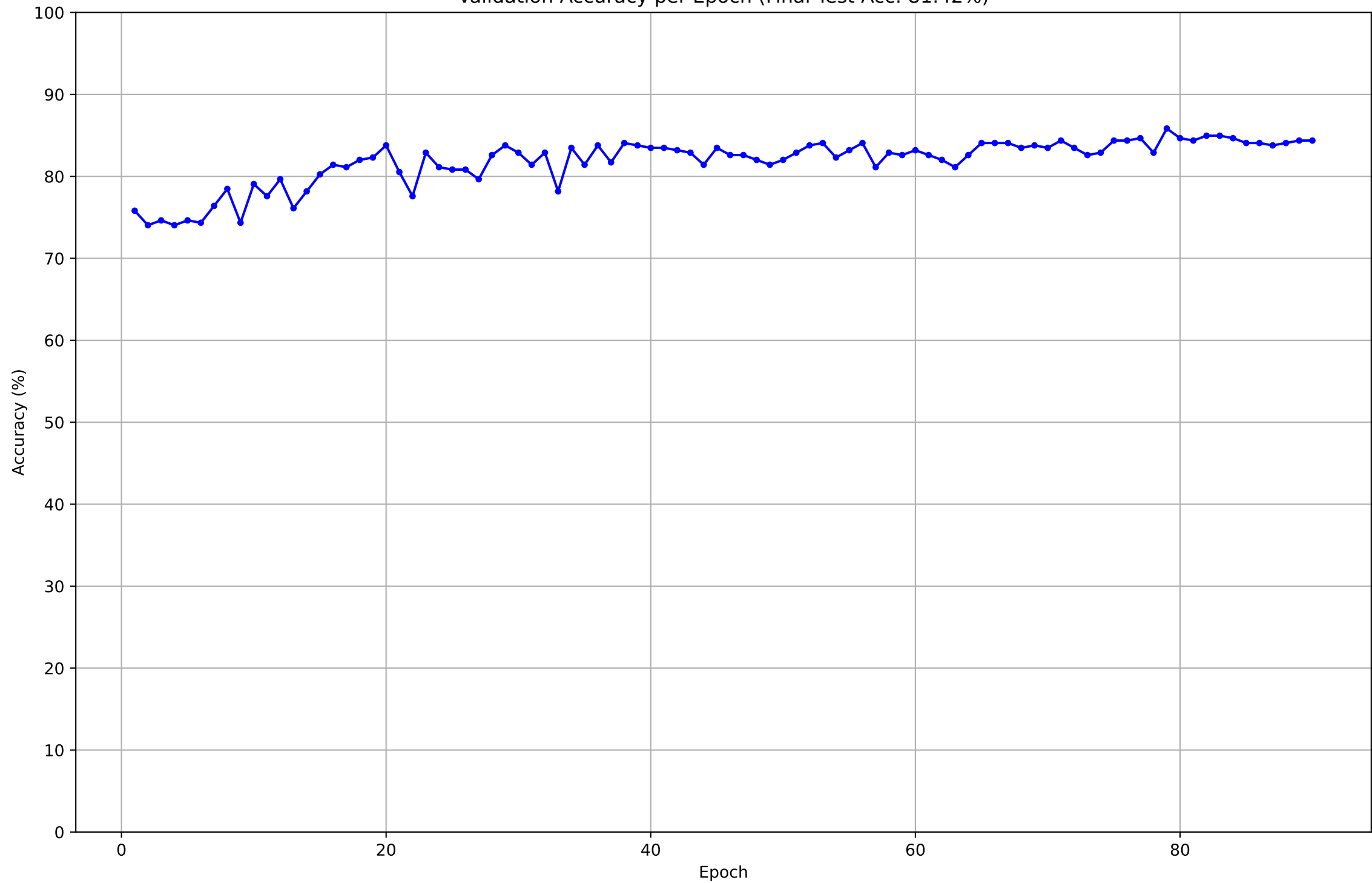
Validation Accuracy per Epoch (Final Test Acc: 81.42%)
