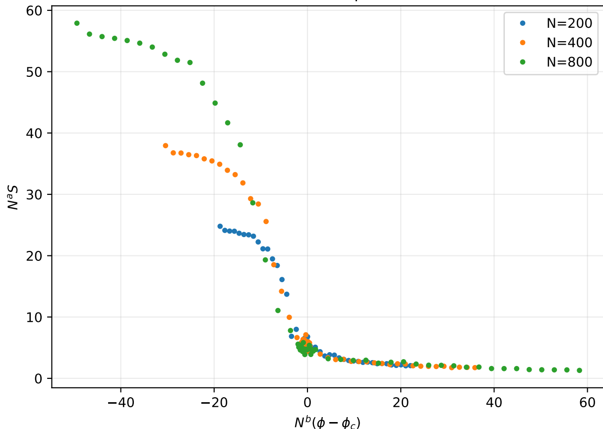
Data collapse
