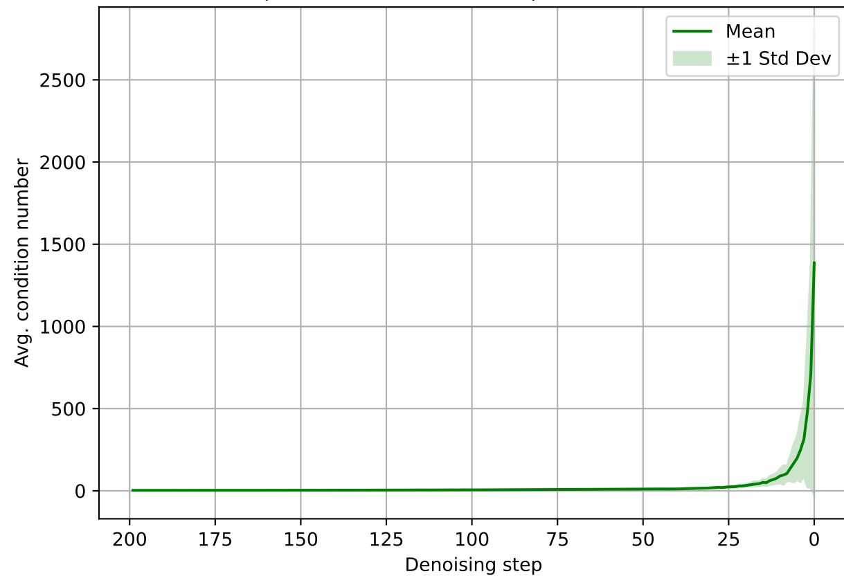
Avg. condition numbers of unit vectors pointing from a noised sample to their predicted denoised sample over 5 trials: letter
