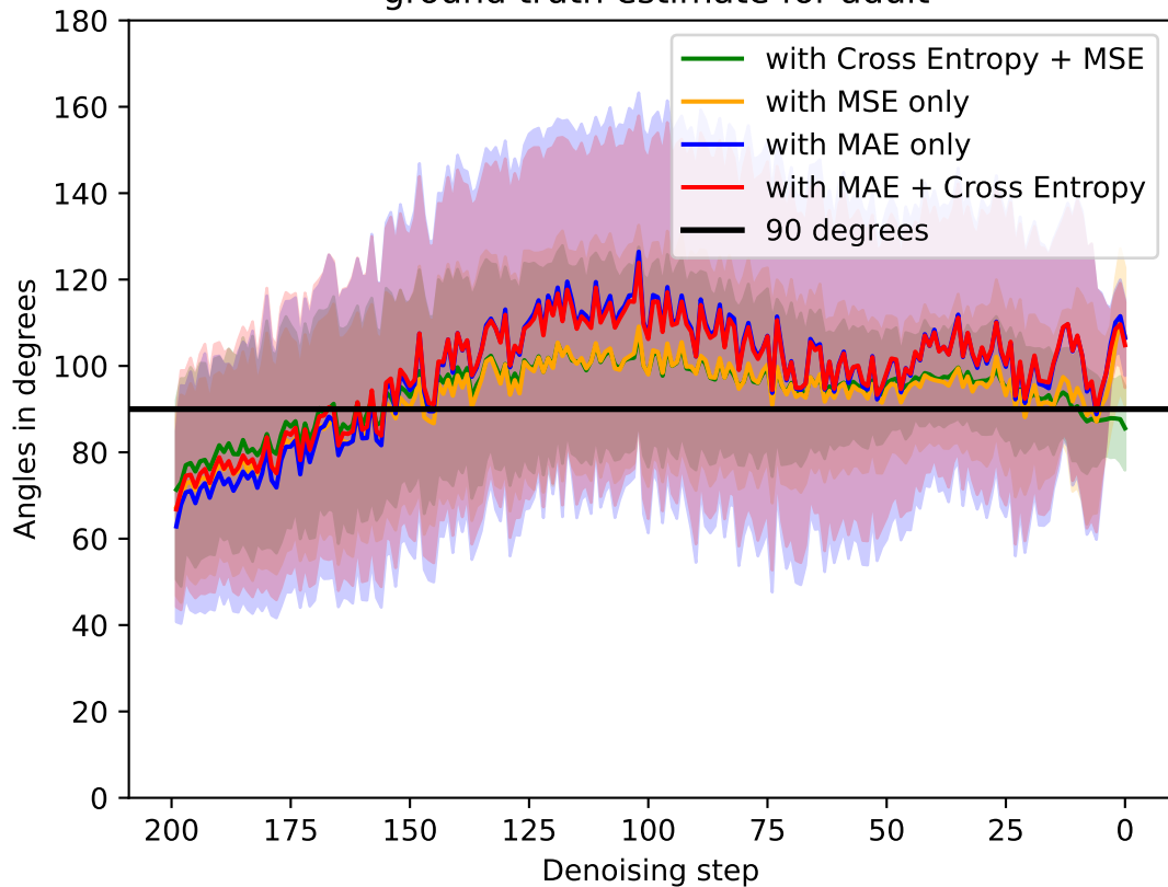
Avg. angles between gradients and denoiser's ground truth estimate for adult
