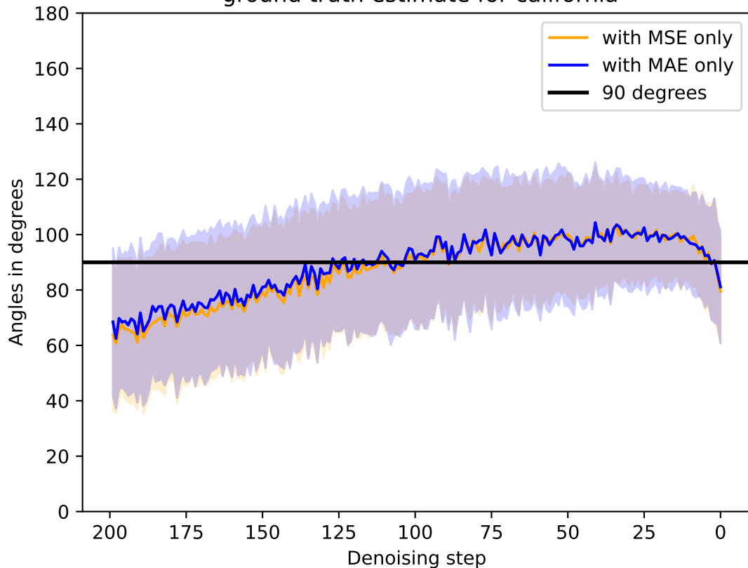
Avg. angles between gradients and denoiser's ground truth estimate for california
