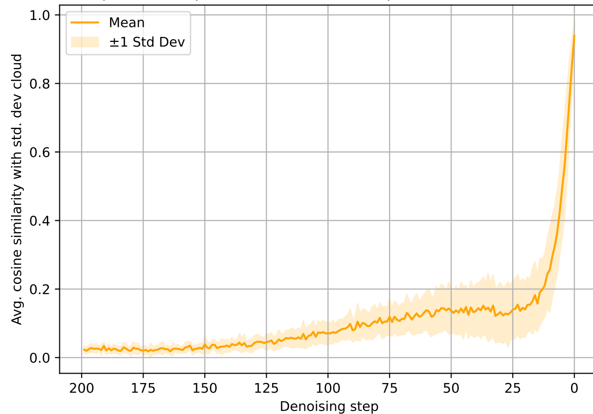
Avg. cosine similarities of unit vectors pointing from a noised sample to their predicted denoised sample over 5 trials: california
