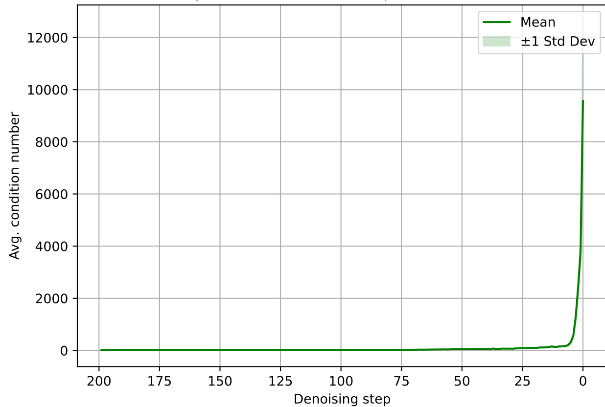
Avg. condition numbers of unit vectors pointing from a noised sample to their predicted denoised sample over 5 trials: adult
