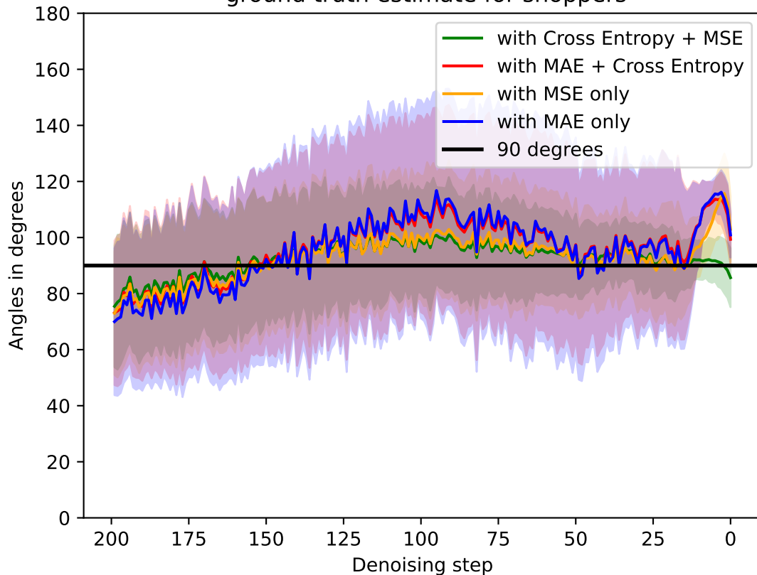
Avg. angles between gradients and denoiser's ground truth estimate for shoppers
