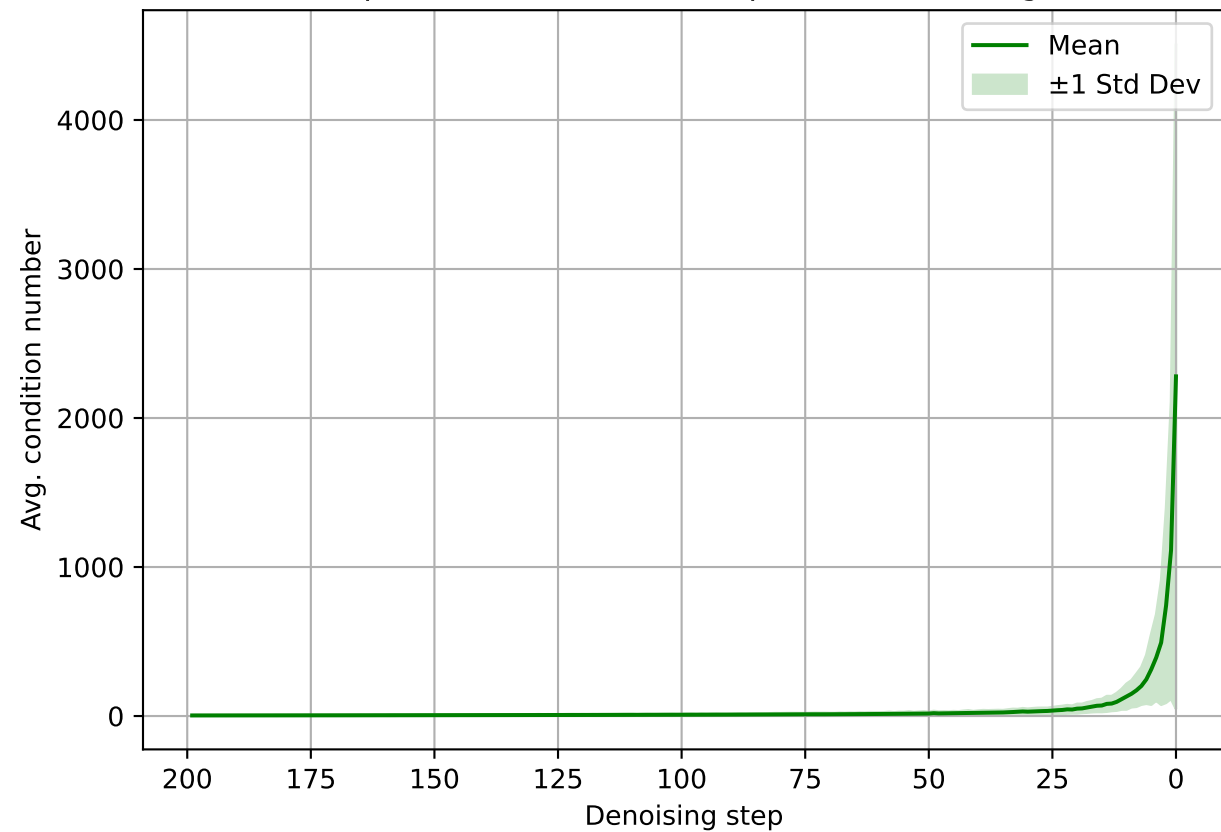
Avg. condition numbers of unit vectors pointing from a noised sample to their predicted denoised sample over 5 trials: gesture
