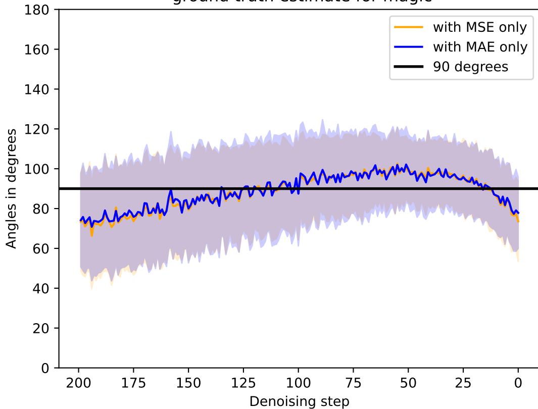
Avg. angles between gradients and denoiser's ground truth estimate for magic
