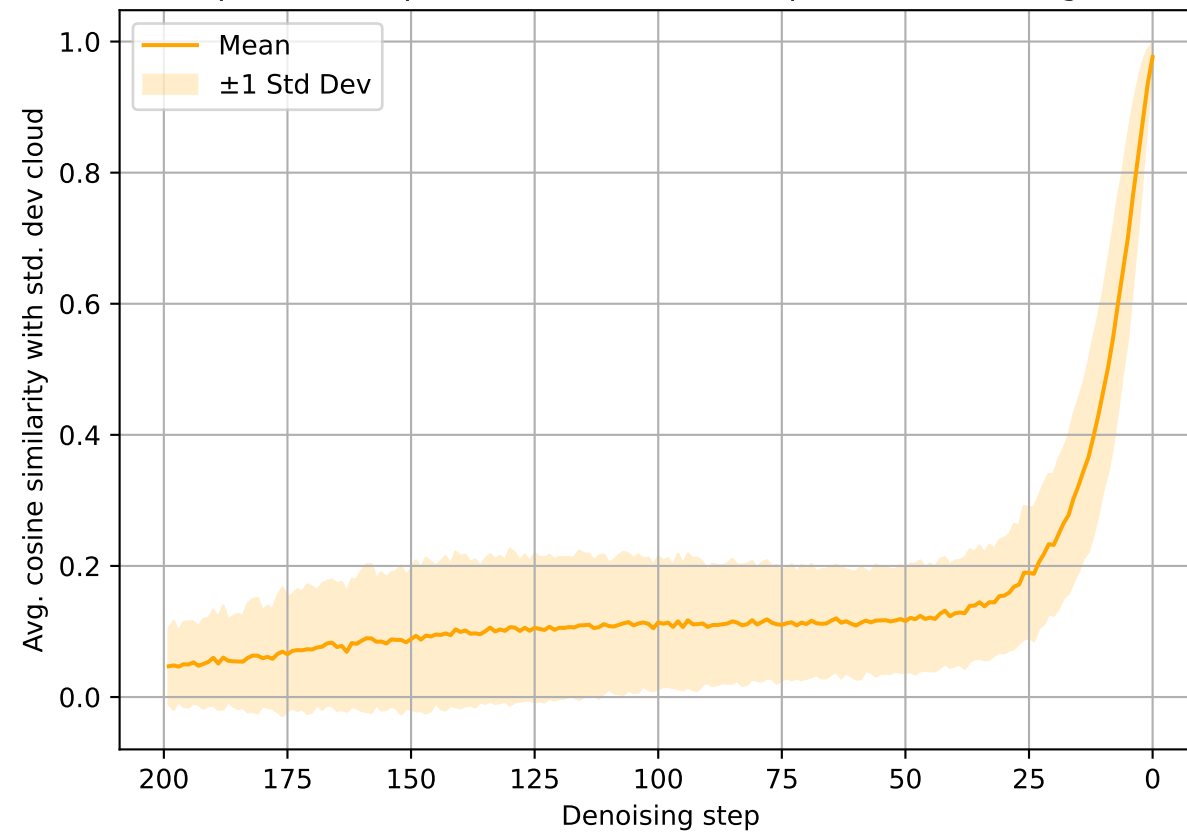
Avg. cosine similarities of unit vectors pointing from a noised sample to their predicted denoised sample over 5 trials: gesture
