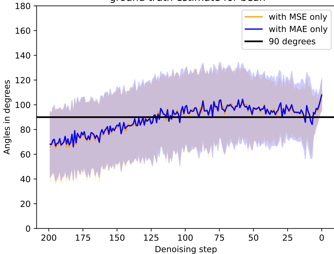
Avg. angles between gradients and denoiser's ground truth estimate for bean
