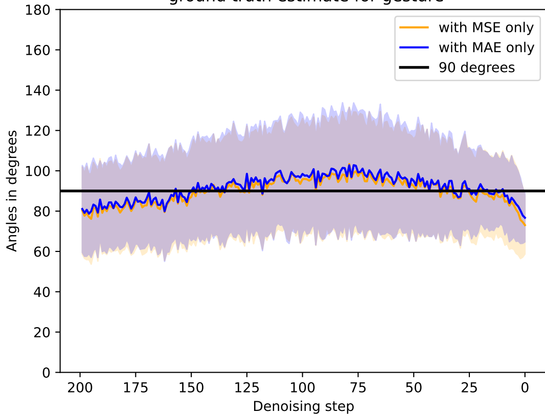
Avg. angles between gradients and denoiser's ground truth estimate for gesture
