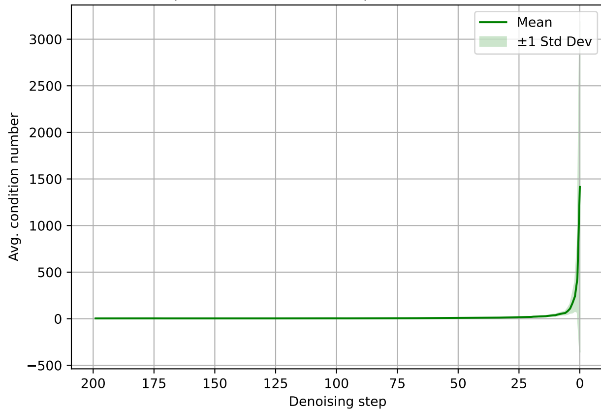
Avg. condition numbers of unit vectors pointing from a noised sample to their predicted denoised sample over 5 trials: california
