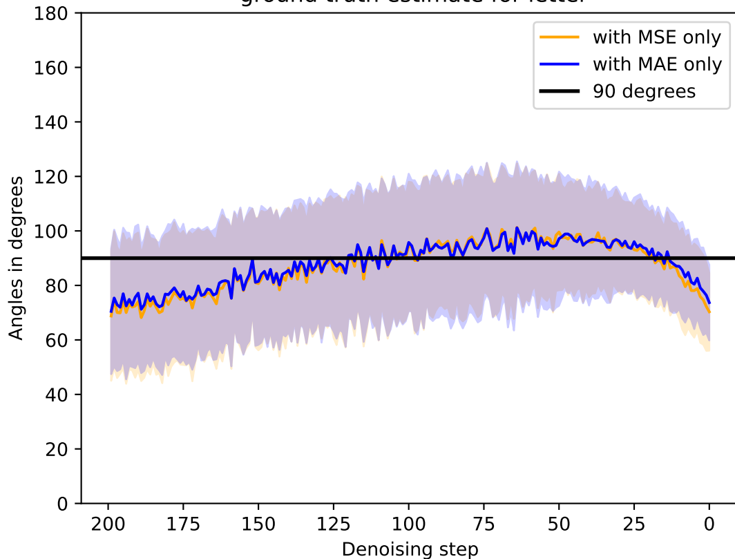
Avg. angles between gradients and denoiser's ground truth estimate for letter
