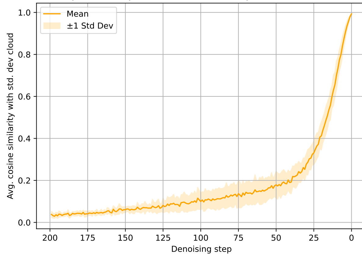
Avg. cosine similarities of unit vectors pointing from a noised sample to their predicted denoised sample over 5 trials: letter
