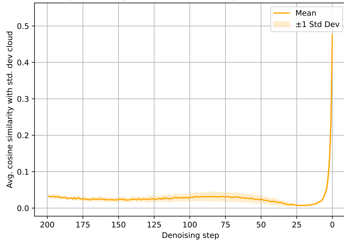
Avg. cosine similarities of unit vectors pointing from a noised sample to their predicted denoised sample over 5 trials: adult
