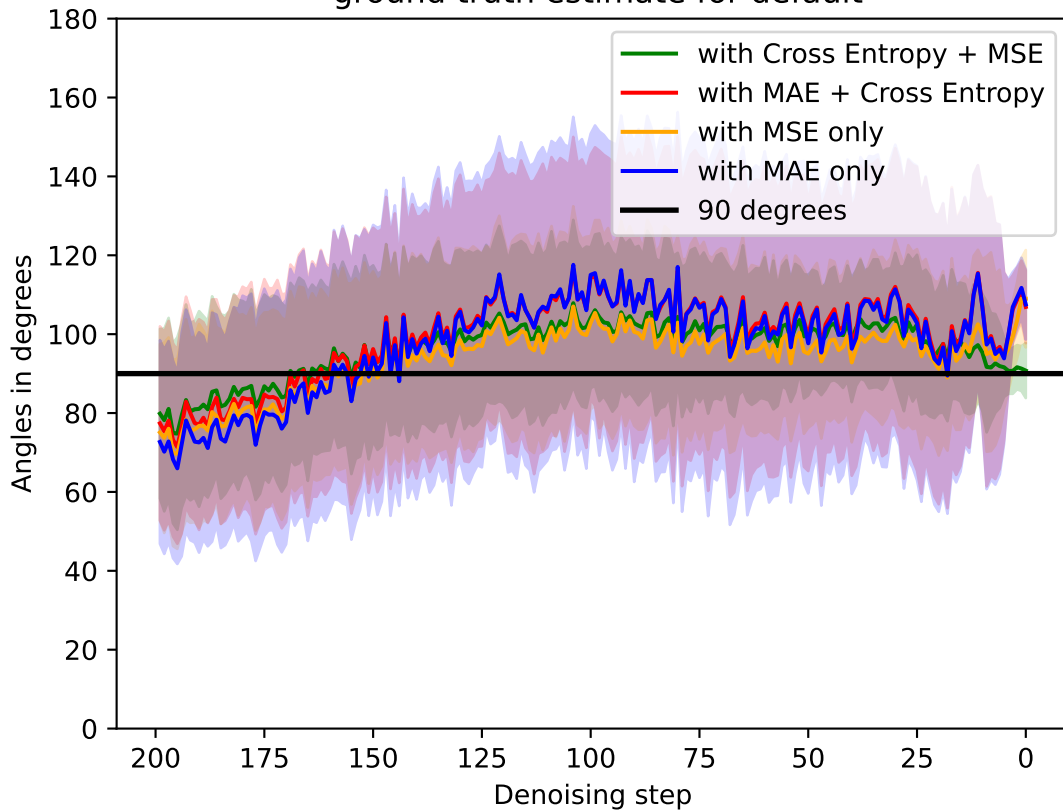
Avg. angles between gradients and denoiser's ground truth estimate for default
