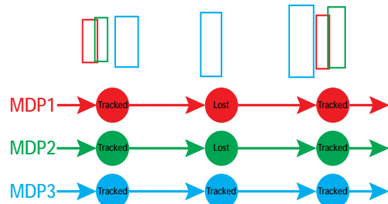
Figure 1. We formulate the online multi-object tracking problem as decision making in a Markov Decision Process (MDP) framework.
