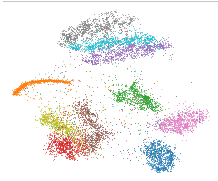
DensMAP \lambda=0.1
