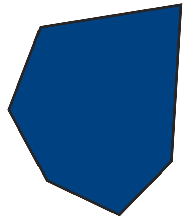
irregular hexagon
