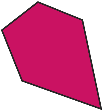
irregular pentagon
