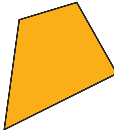
irregular quadrilateral
