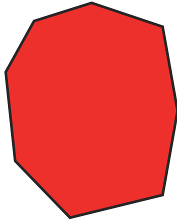
irregular octagon
