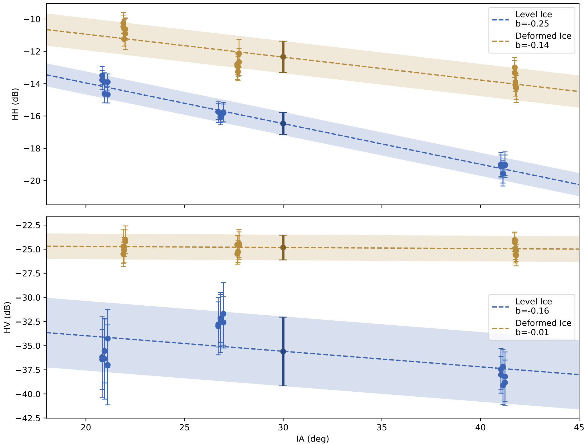
Sentinel-1 fastice backscatter ( \sigma_0 ) in Oct 2024
