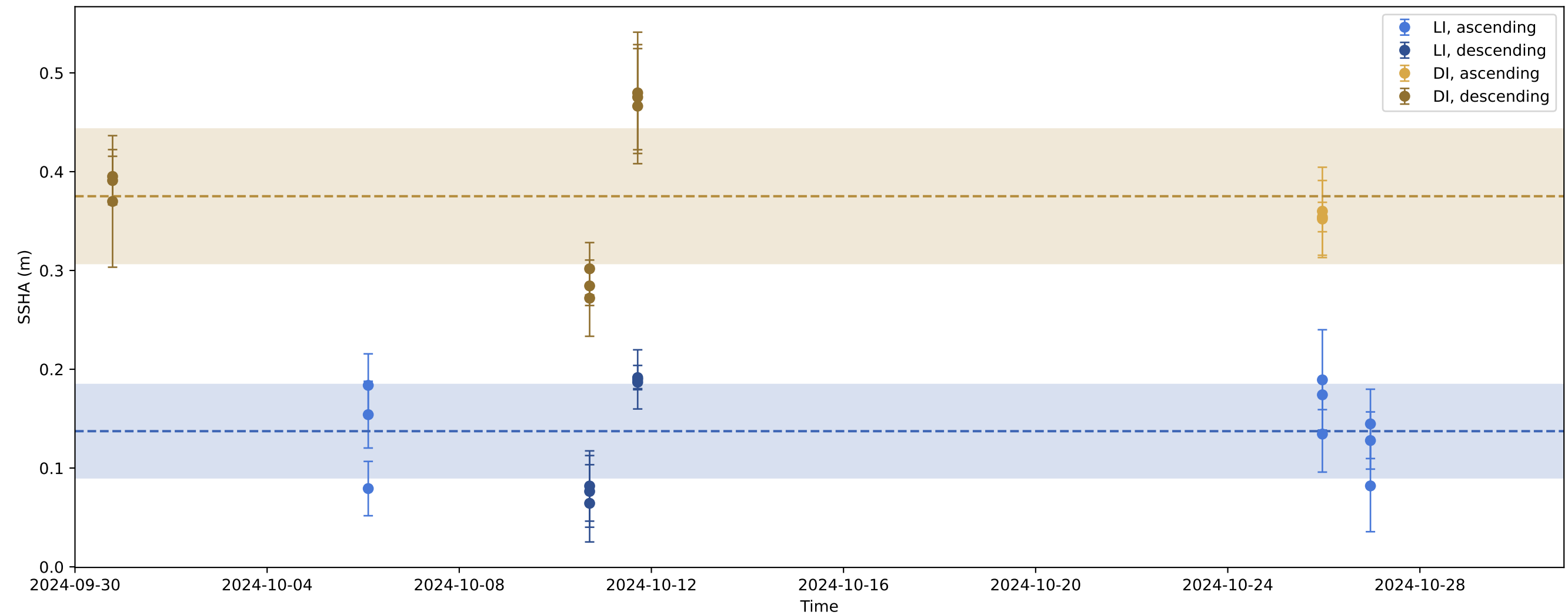
Fastice SSHA in Oct 2024
