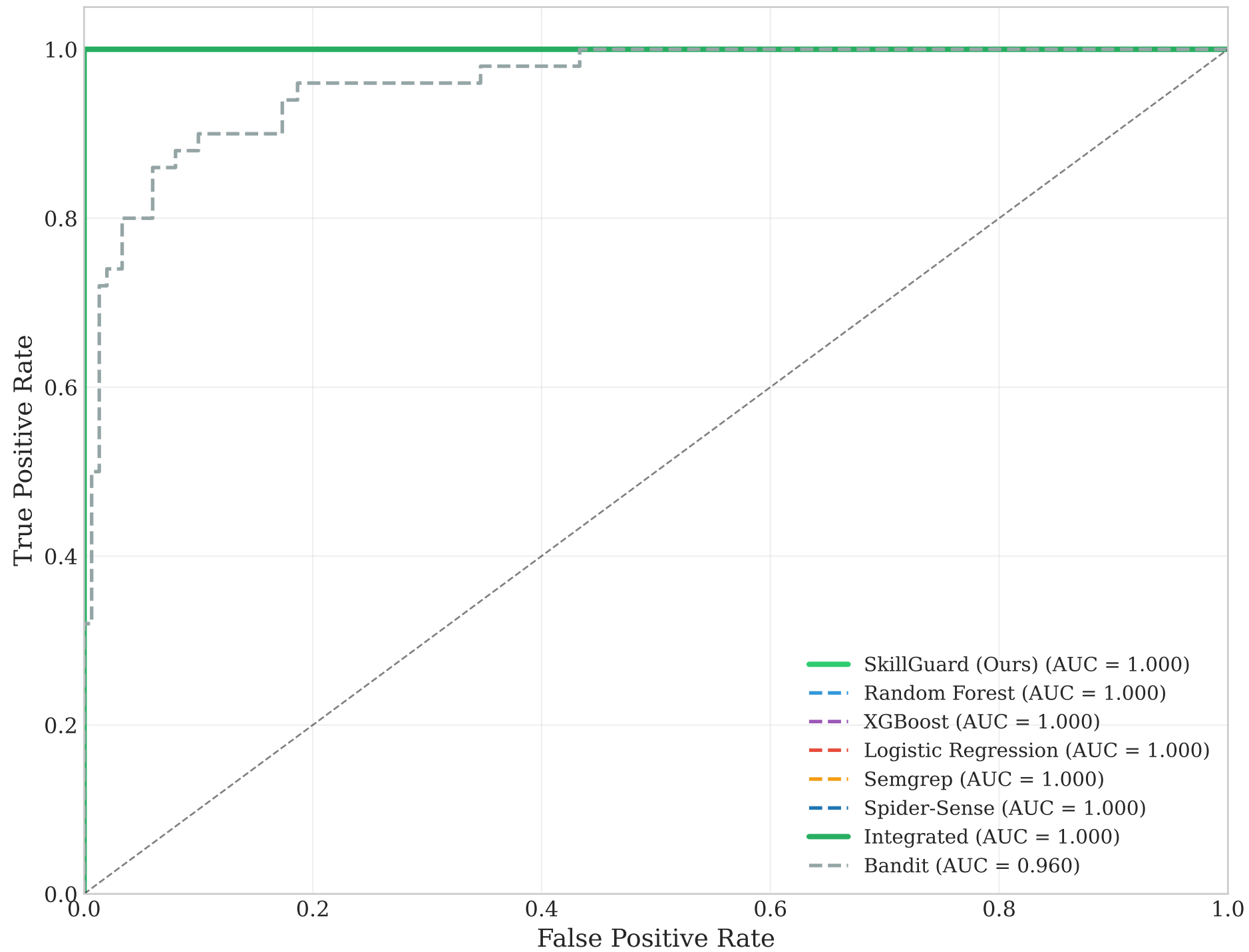
ROC Curves: Malicious Skill Detection
