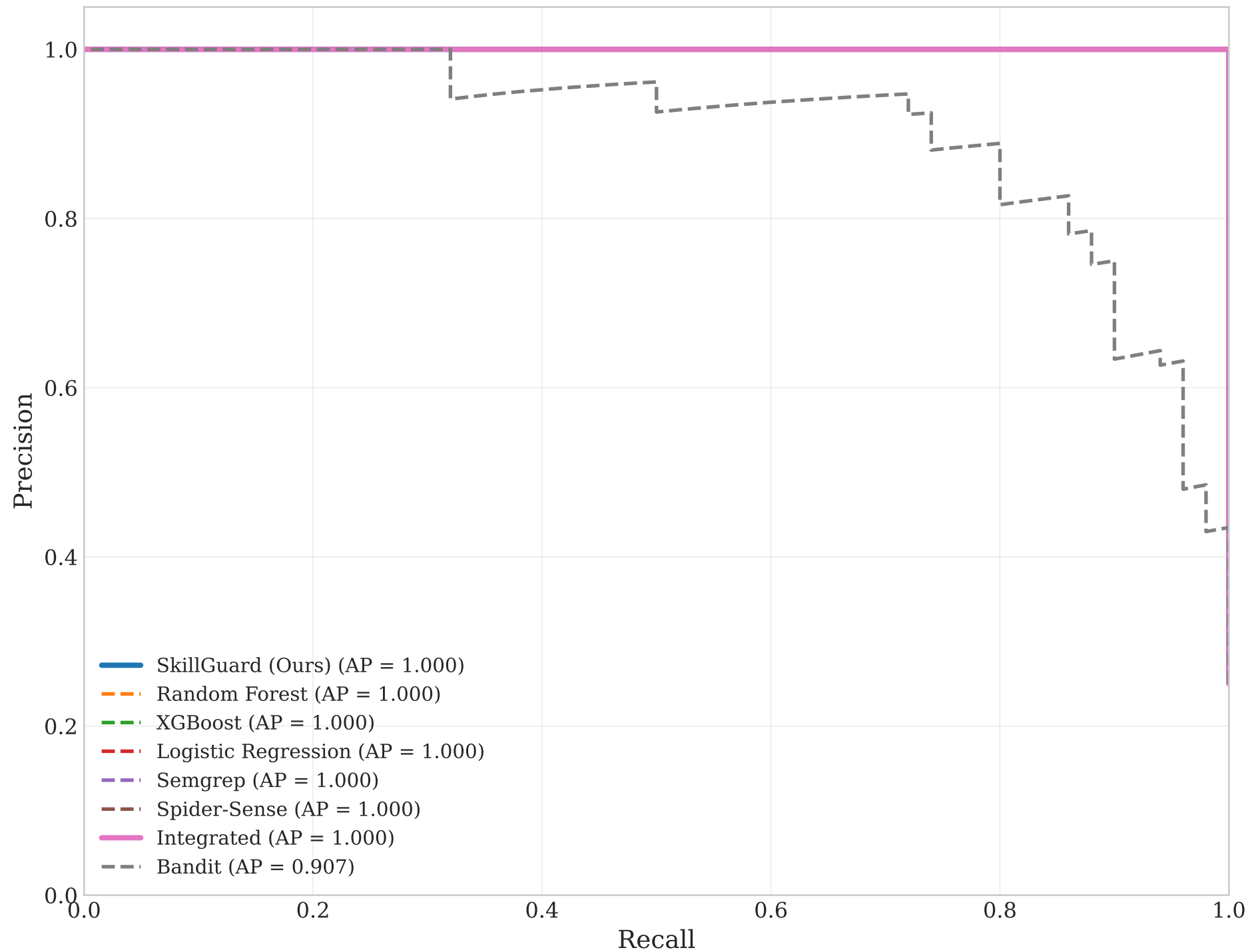
Precision-Recall Curves: Malicious Skill Detection
