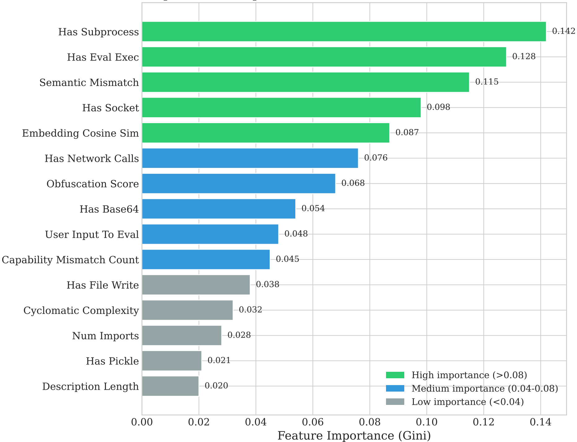
Top 15 Most Important Features for Malicious Skill Detection
