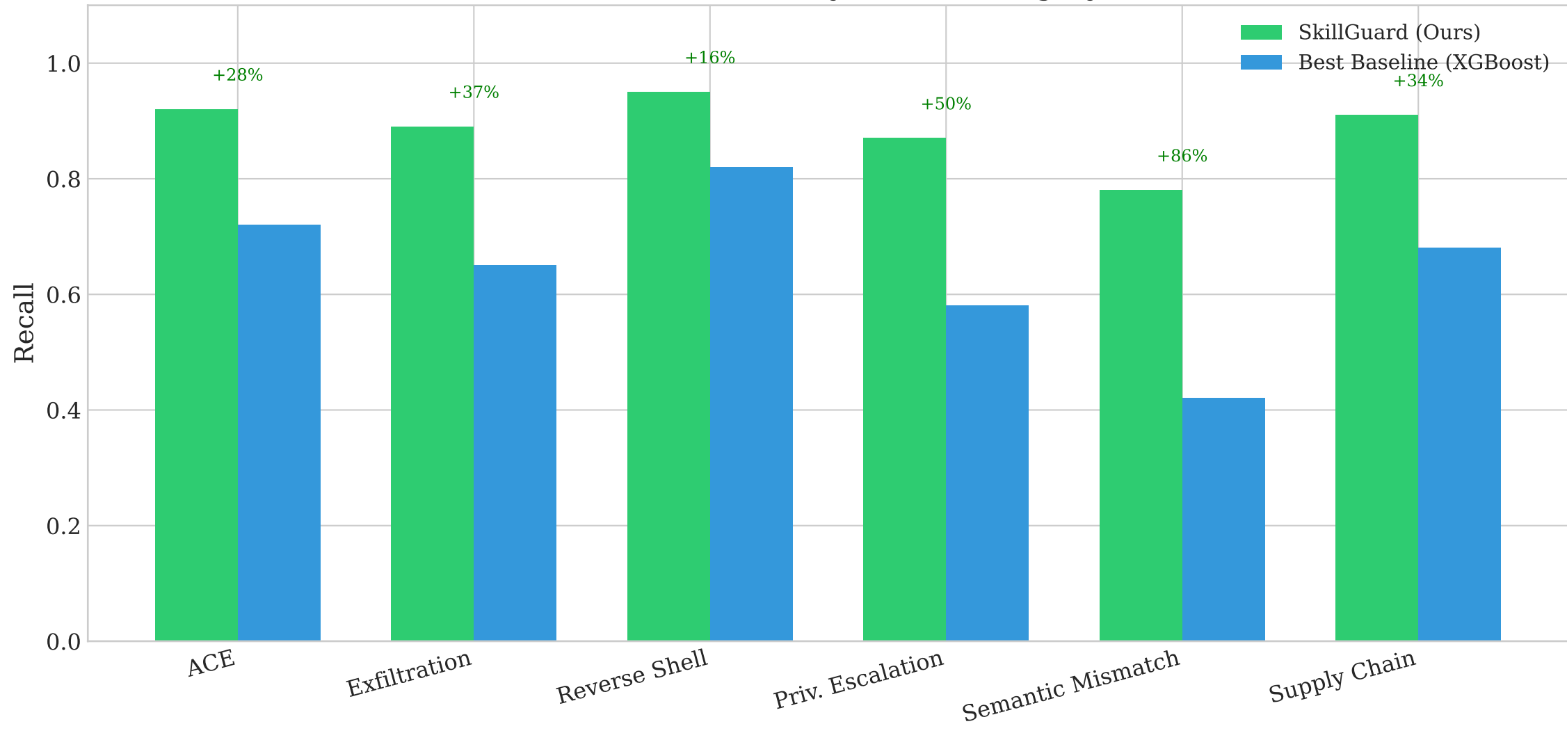
Detection Recall by Threat Category
