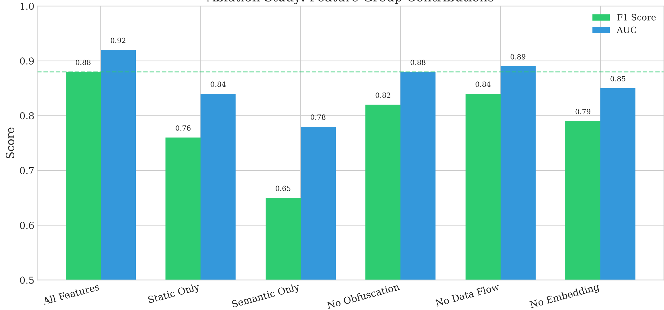
Ablation Study: Feature Group Contributions
