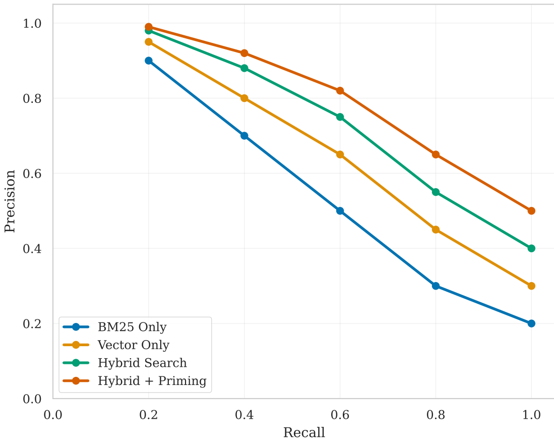
Precision-Recall Curves
